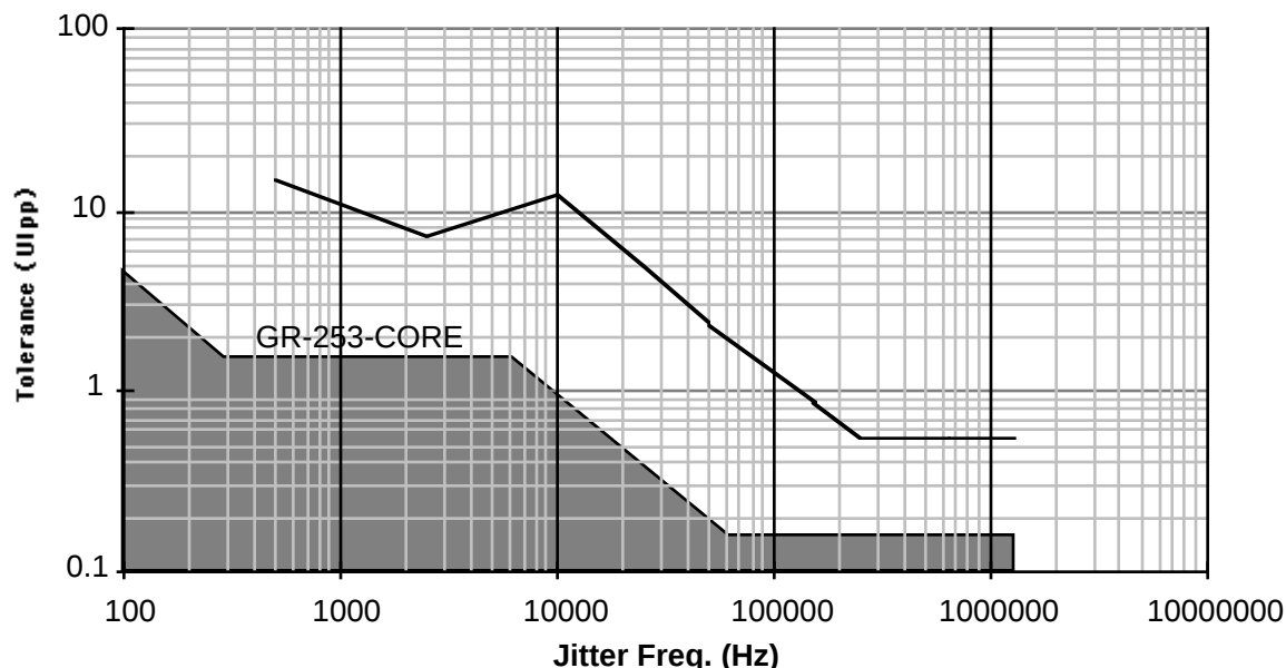
Fig. 2 STS-3c/STM-1Jitter Tolerance
