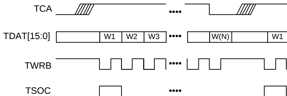
Figure 31 - Transmit FIFO
