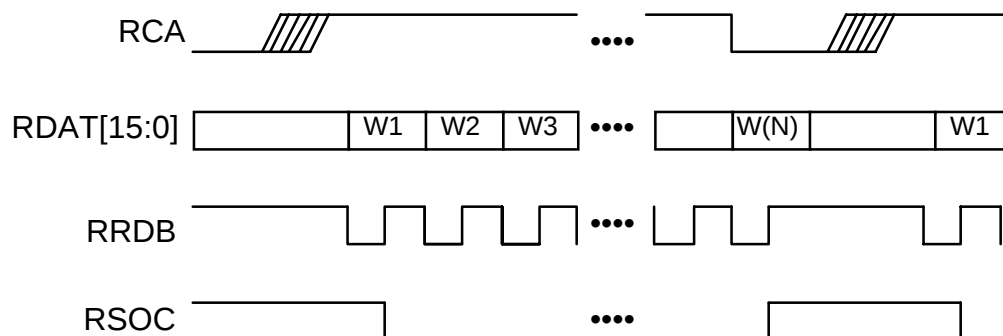
Figure 30 - Receive FIFO
