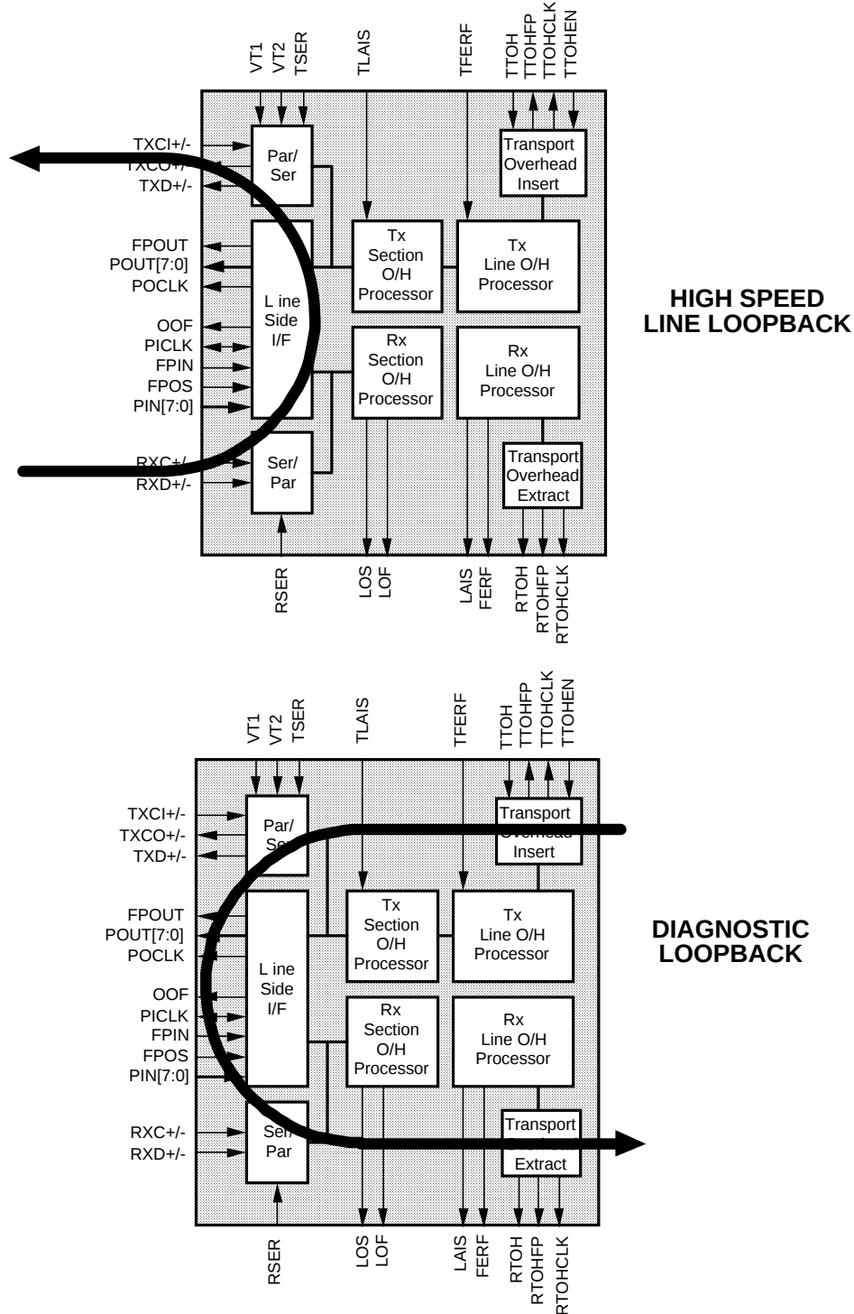
Figure 13 - Loopback Operation
