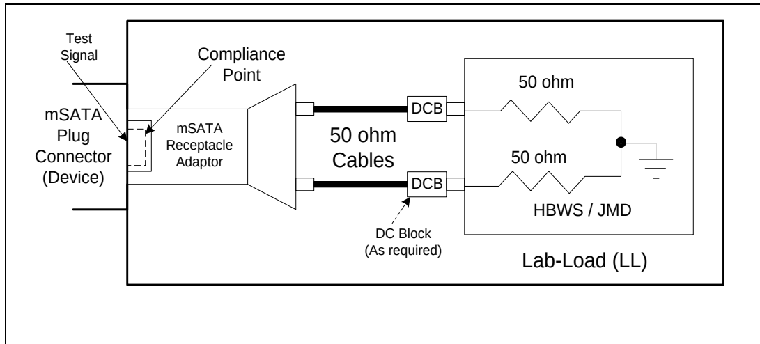
Figure 196 – Lab-Load (LL) for mSATA device
