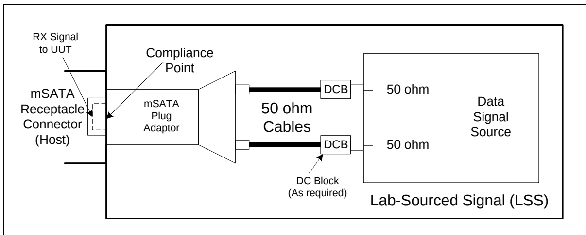
Figure 205 – Lab-Sourced Signal (LSS) for mSATA host
