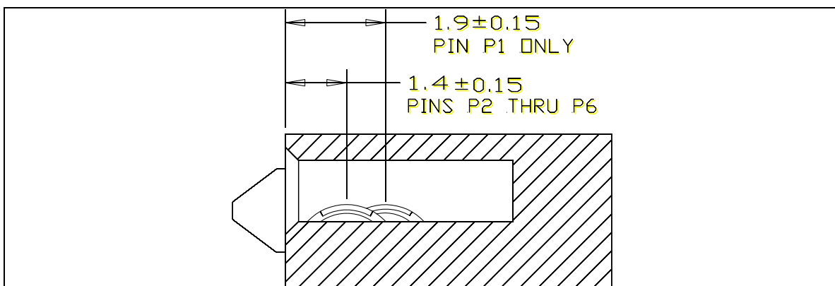
Figure 87 – Slimline host receptacle connector interface dimensions section Y-Y
