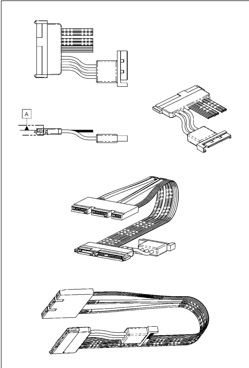
Figure 139 – Example power pigtail to be used with the 15 pin SATA power connector
