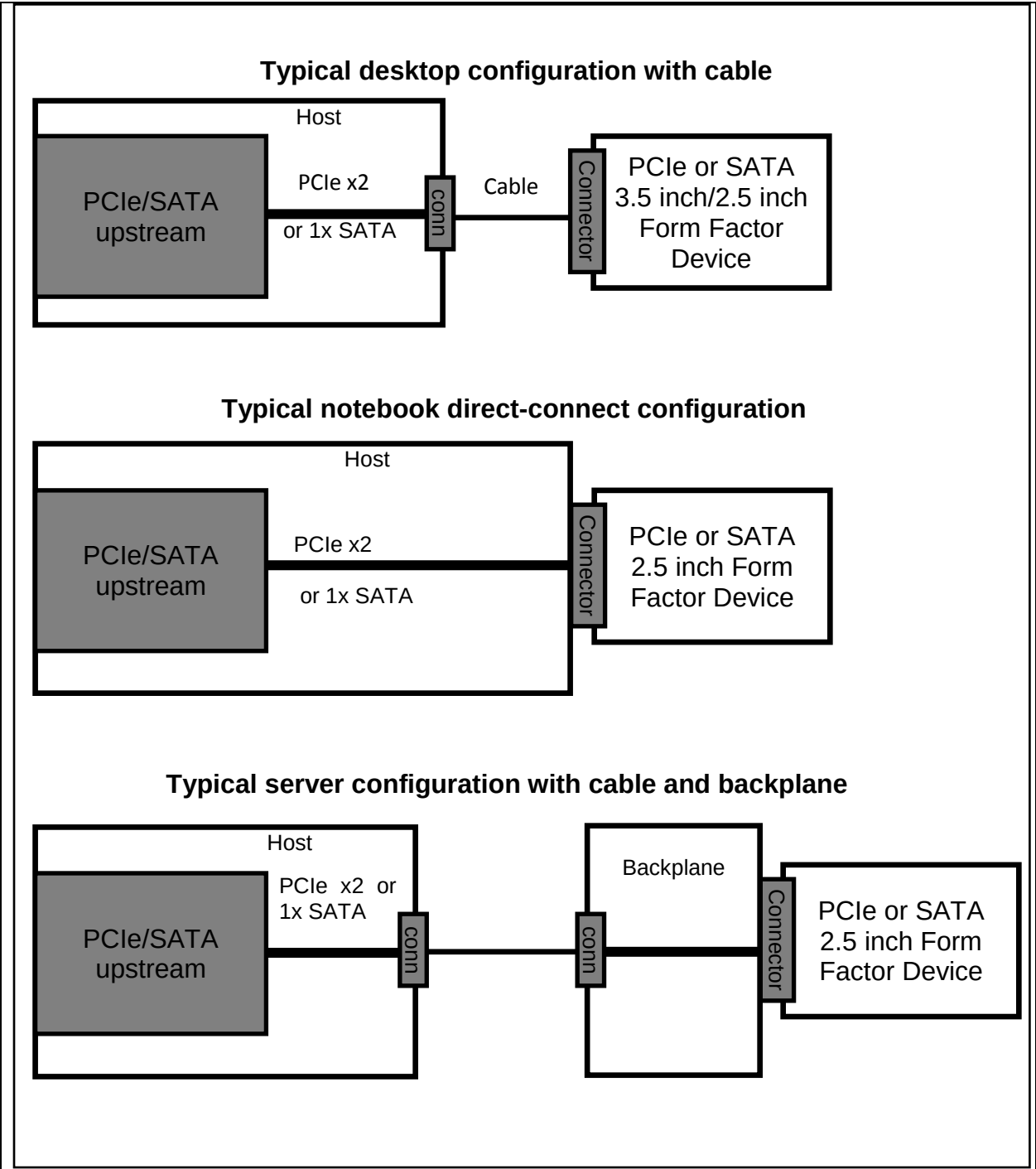
Figure 124 – Example configurations for client
