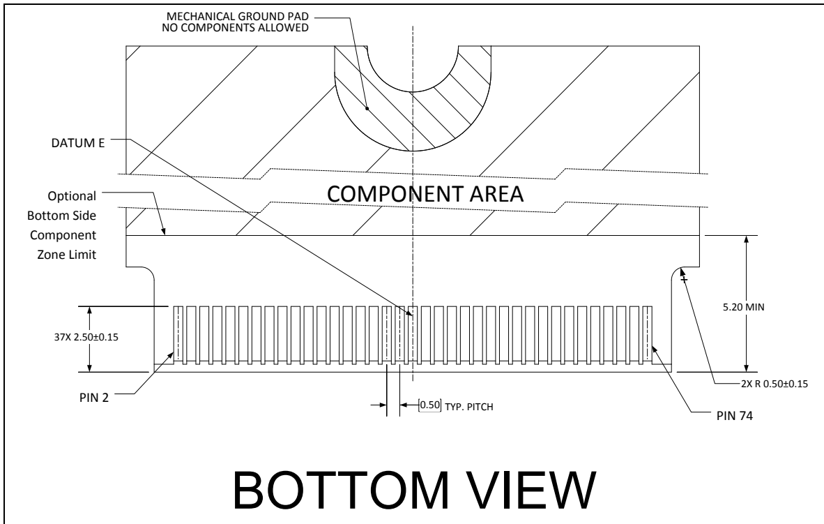
Figure 111 – M.2 board connector bottom details (informative)
