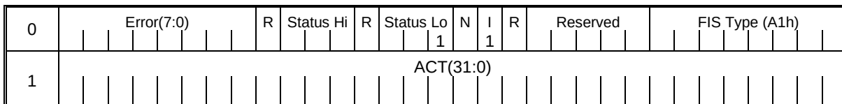
Figure 366 – HYBRID DEMOTE BY SIZE – error during processing
