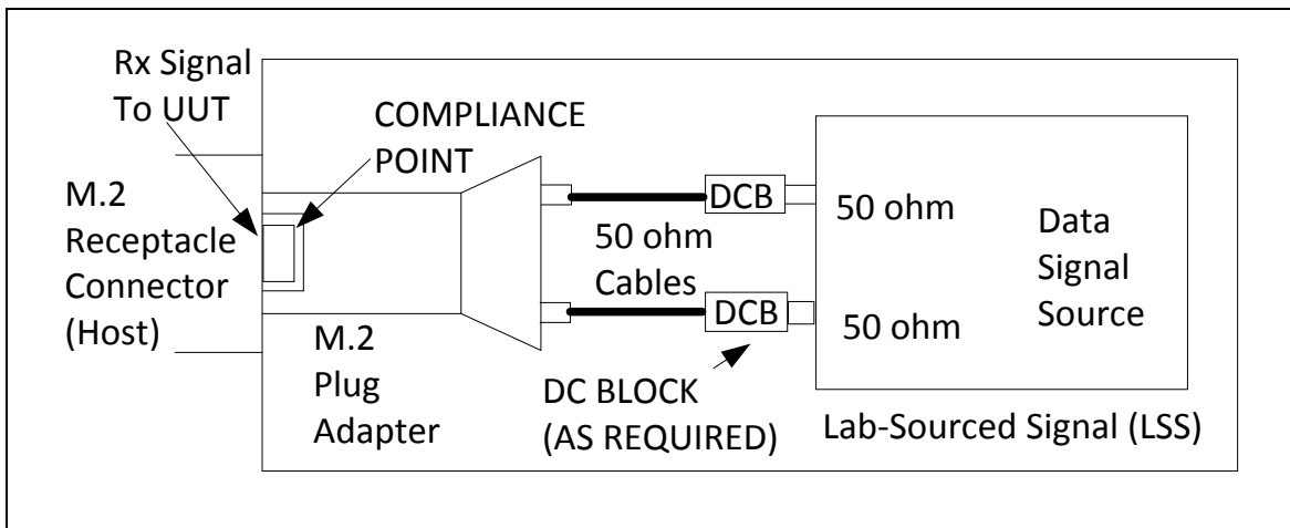
Figure 210 – Lab-Sourced Signal (LSS) for M.2 host
