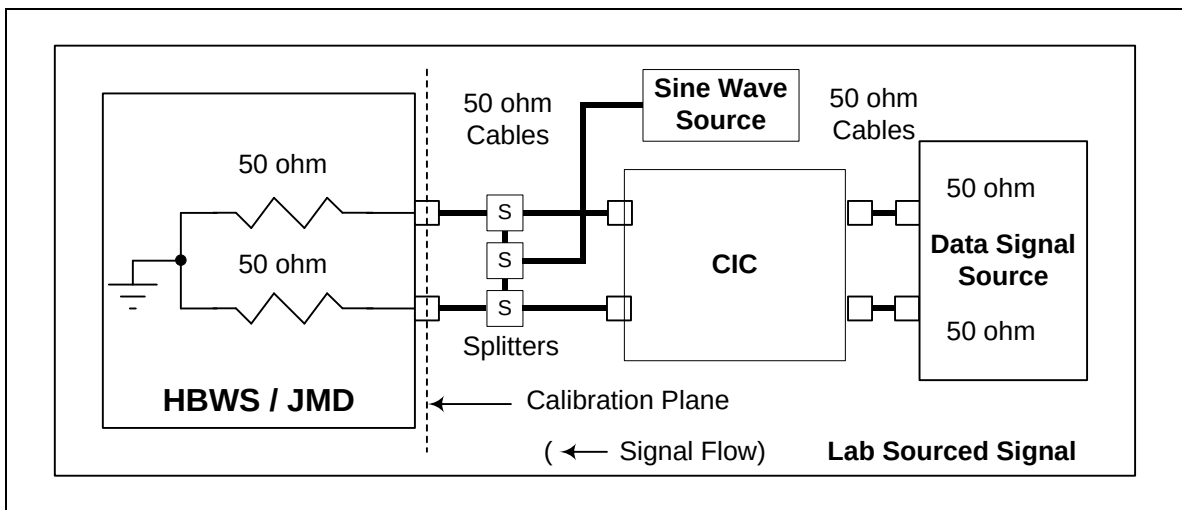
Figure 231 – Receiver jitter and CM tolerance test – setting TJ and CM levels (Gen3i)
