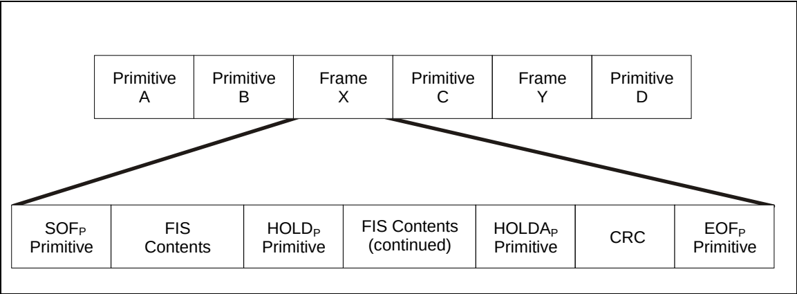
Figure 269 – Transmission structures
