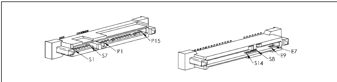
Figure 125 – SATA Express pinout for host receptacle connectors
