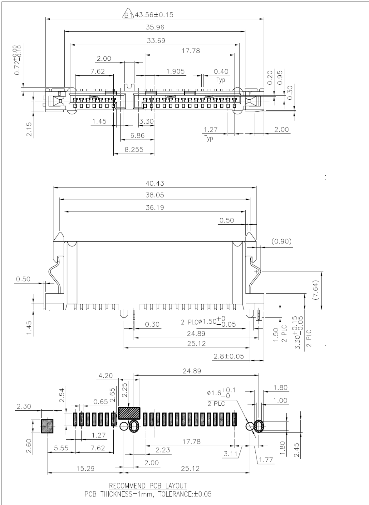
Figure 101 – SATA USM vertical receptacle (see INF-8280)
