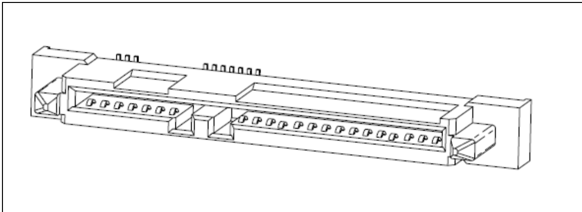
Figure 130 – SATA Express host receptacle connector isometric drawing
