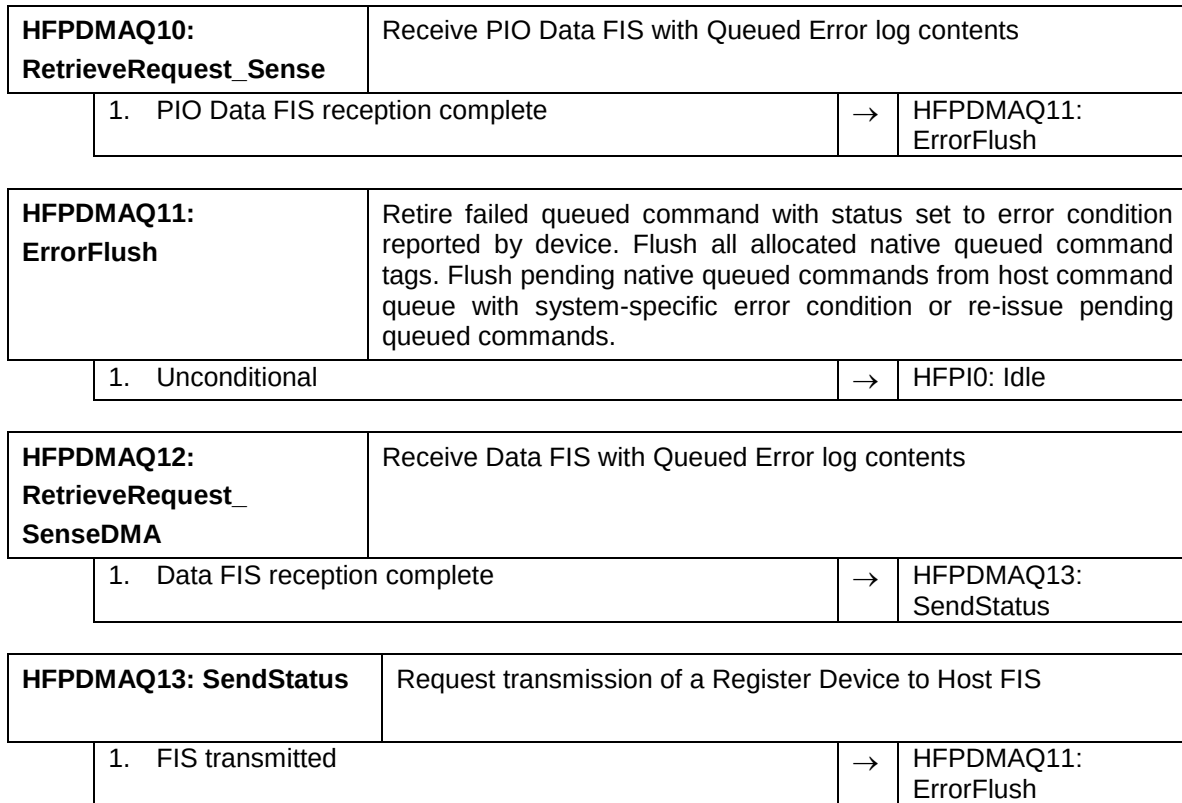
Figure 335 – Host command layer FPDMA queued state machine (part 3 of 3)
