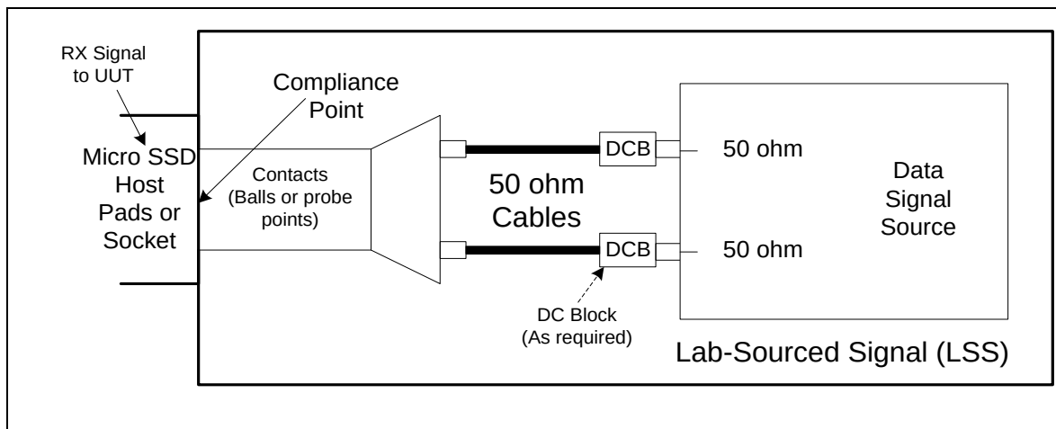
Figure 208 – Lab-Sourced Signal (LSS) for SATA MicroSSD host
