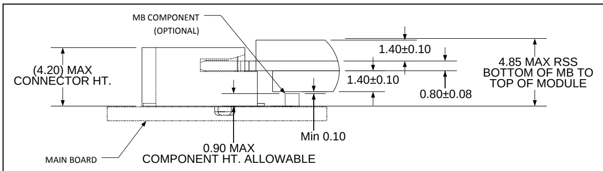
Figure 119 – M.2 double sided assembly – D5 (informative)
