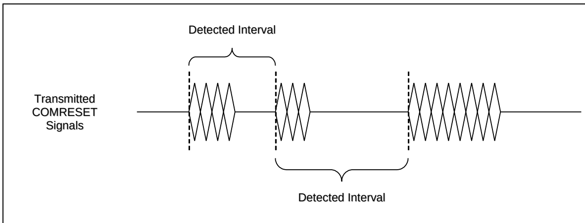
Figure 446 – Port selection signal based on assertion of COMRESET to assertion of following COMRESET
