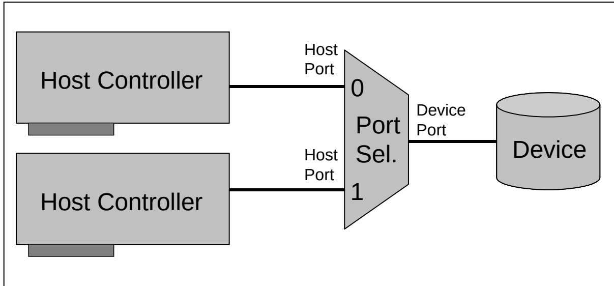
Figure 444 – Port Selector overview
