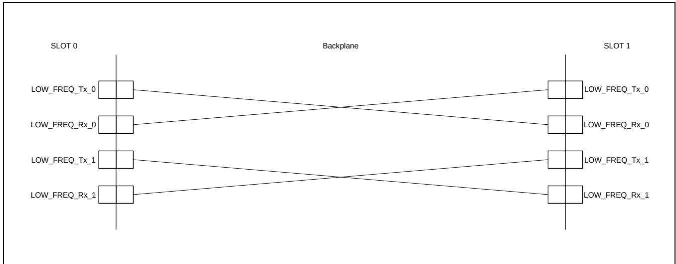
Figure D.6 – Low speed channels
