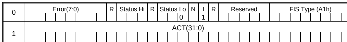
Figure 348 – ABORT NCQ QUEUE – successful completion
