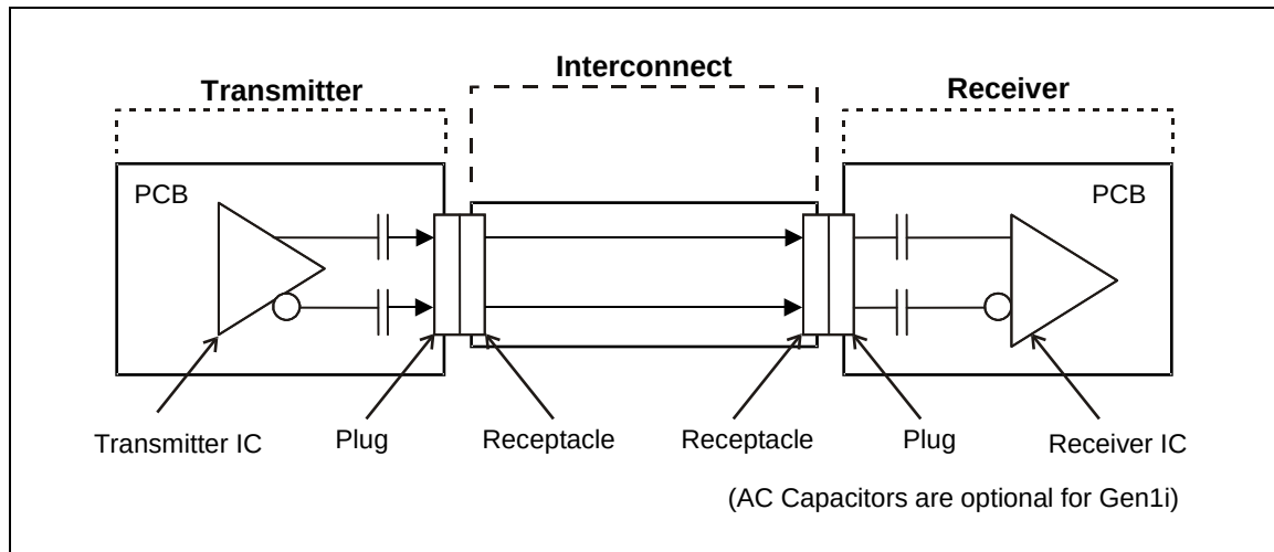
Figure 165 – The simplex link
