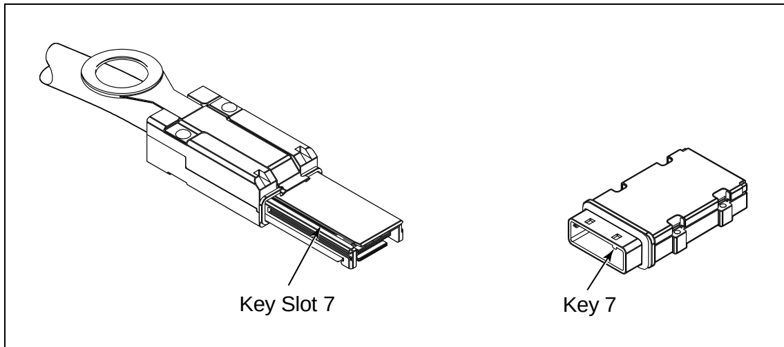
Figure 153 – Mini SATA External Multilane system, key slots 7 for m level signals
