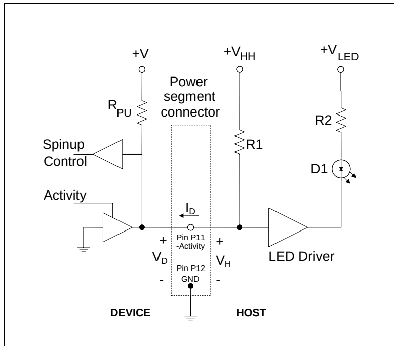
Figure 155 – Example Device Activity Signal (DAS) electrical block diagram
