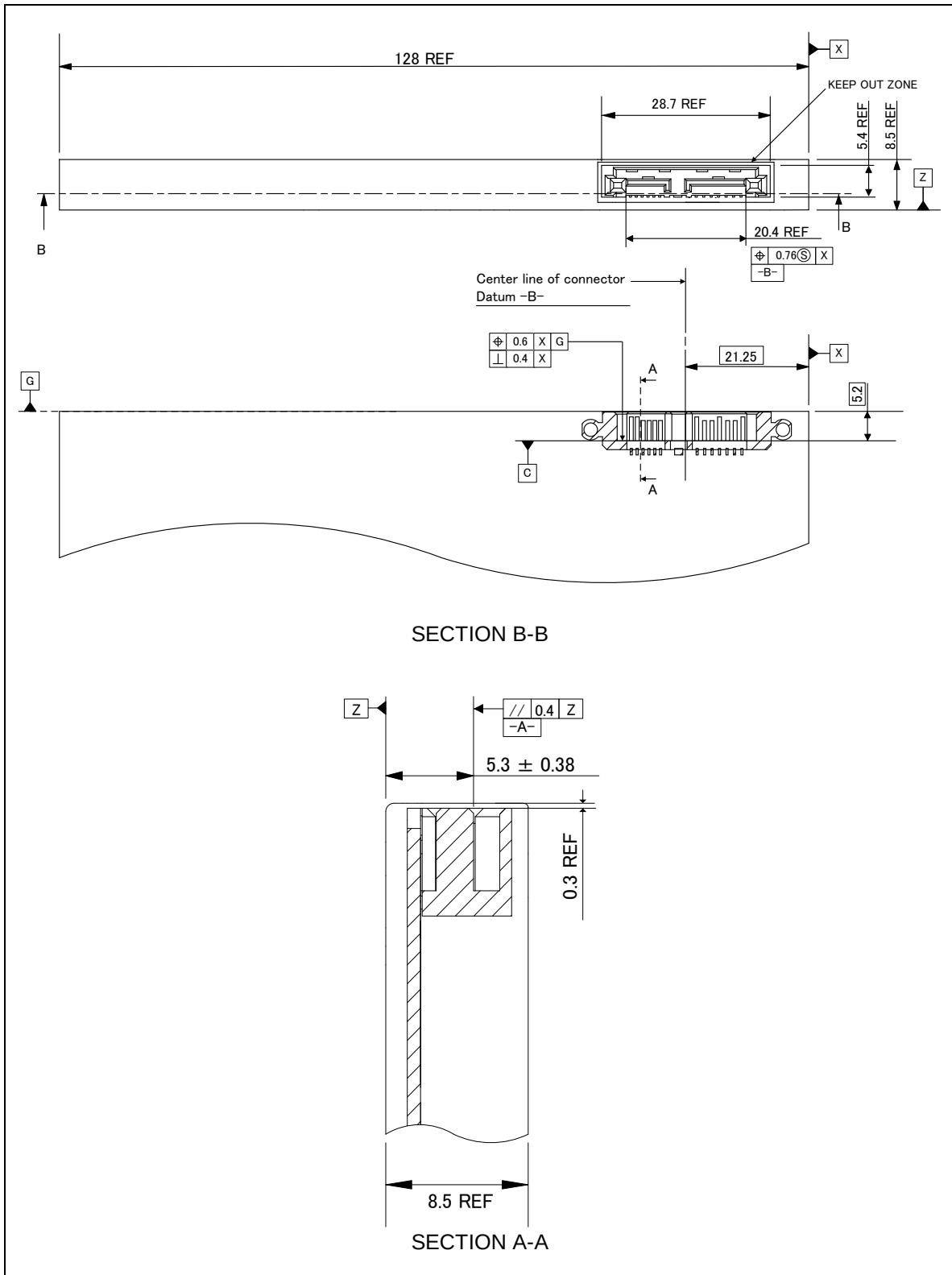
Figure 64 – 8.5 mm Slimline drive connector locations (informative)
