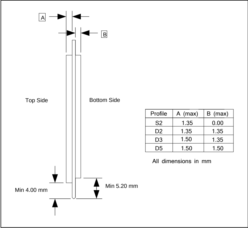
Figure 121 – M.2 component profile and keep out zone (informative)
