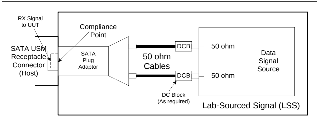
Figure 206 – Lab-Sourced Signal (LSS) for SATA USM host
