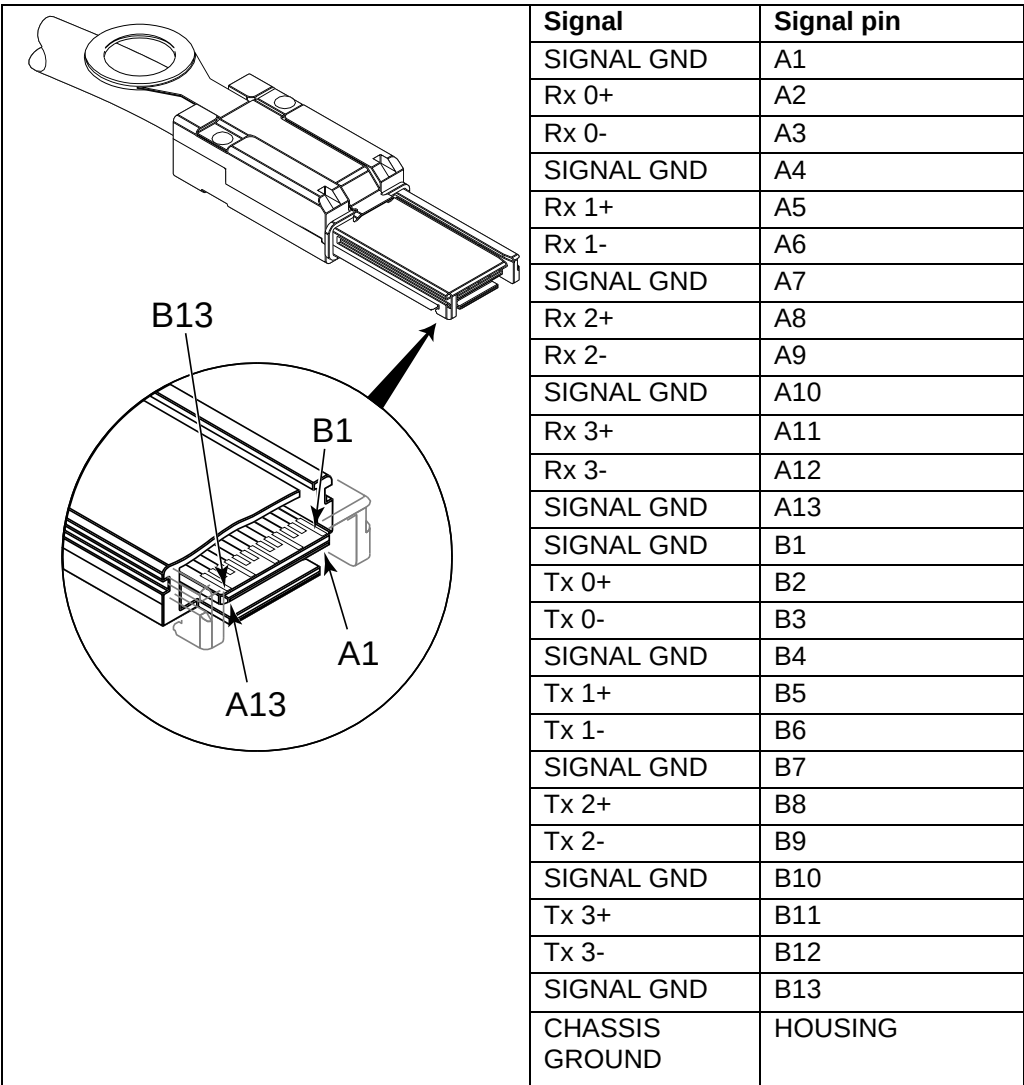
Figure 154 – Mini SATA External Multilane connector pin assignments
