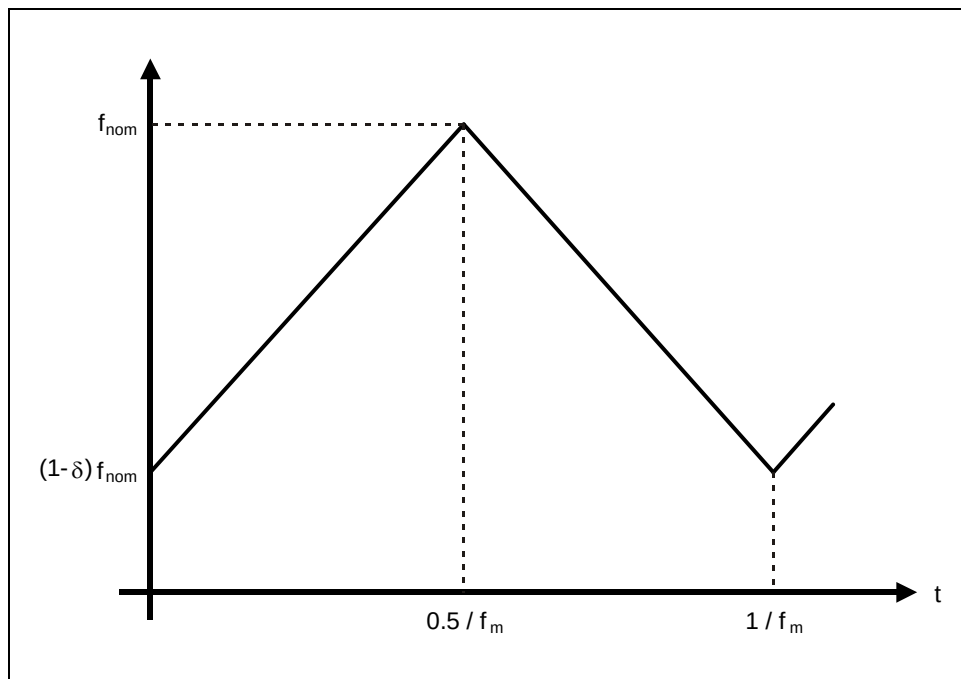
Figure 193 – SSC profile example, triangular
