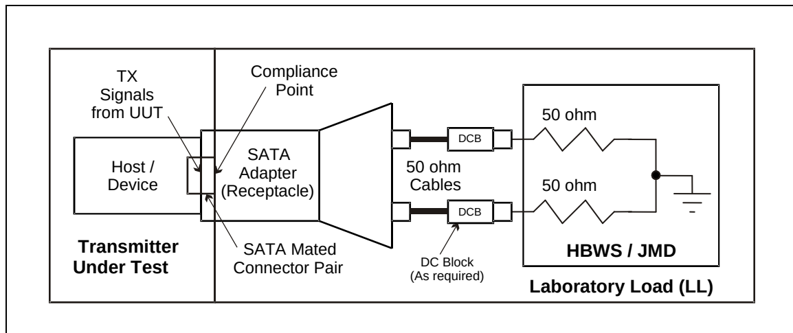
Figure 226 – Transmitter jitter test (Gen1i, Gen2i)
