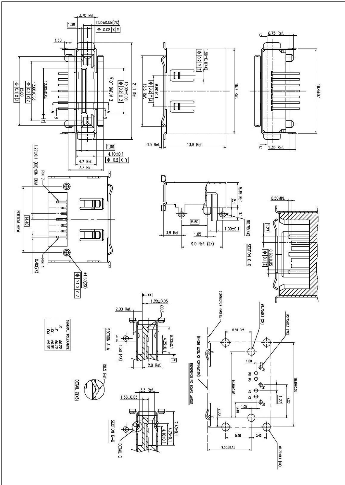
Figure 146 – Mechanical dimensions of External Serial ATA RA through-hole
