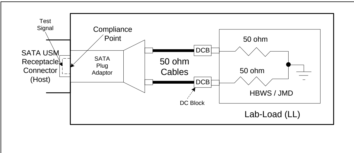
Figure 198 – Lab-Load (LL) for SATA USM host
