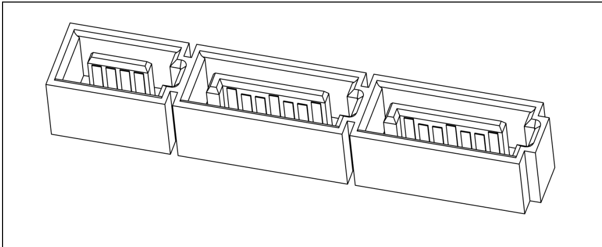
Figure 133 – SATA Express host plug connector isometric drawing
