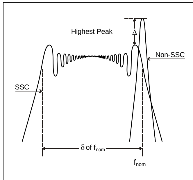
Figure 194 – Spectral fundamental frequency comparison
