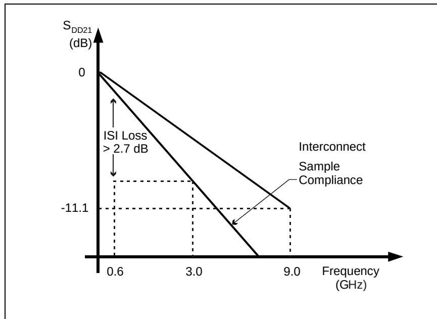
Figure 192 – Compliance Interconnect Channel (CIC) loss for Gen3i
