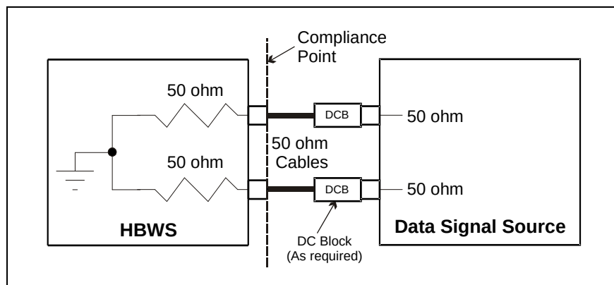
Figure 236 – Receiver intra-pair skew test – setting levels
