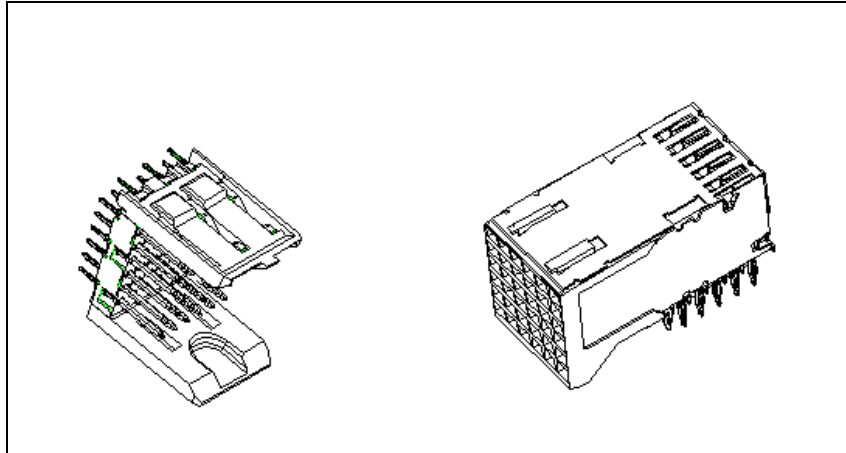
Figure D.8 – I/O controller module connector rendering
