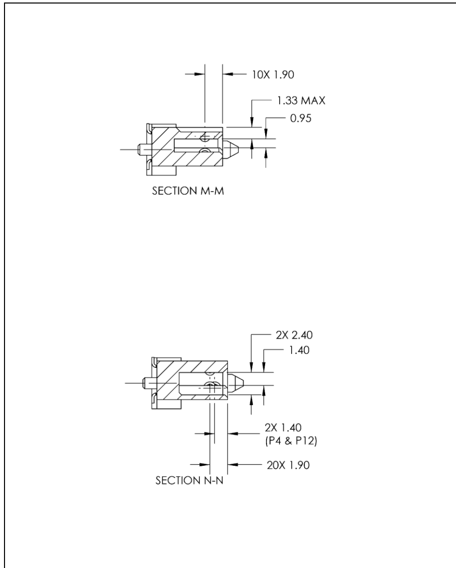
Figure 131 – SATA Express host receptacle connector drawing (part 2 of 2)
