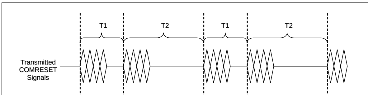
Figure 447 – Complete port selection signal consisting of two sequences with requisite inter-reset spacings
