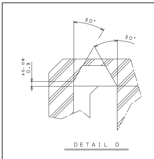
Figure 71 – 7.0 mm Slimline device plug connector interface dimensions detail D
