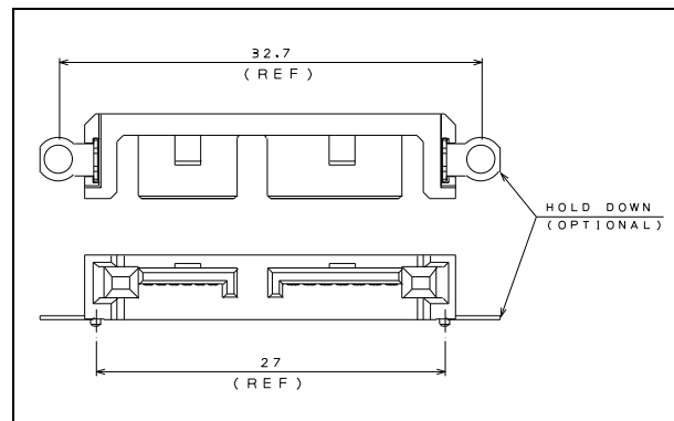
Figure 72 – 7.0 mm Slimline device plug connector interface dimensions optional hold down mounting
