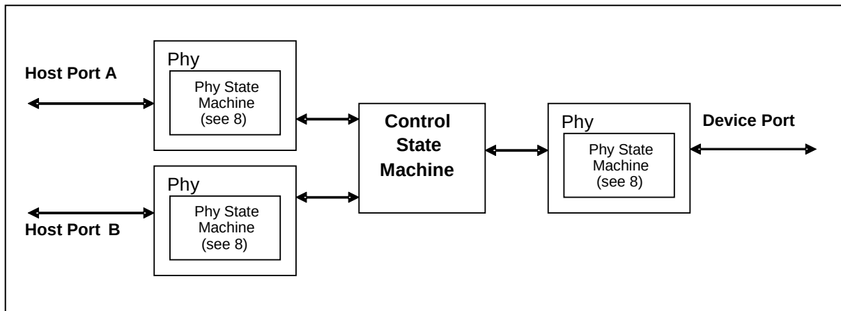
Figure 449 – Control state machine
