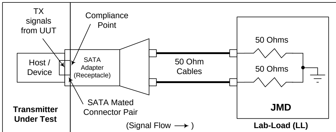
Figure 227 – Transmitter jitter test at Tx (Gen3i)
