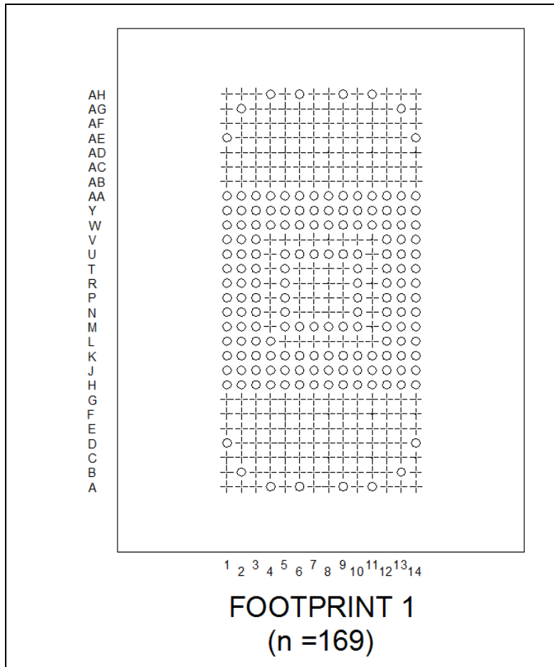
Figure 105 – Footprint 1, SATA MicroSSD variant AC, 169 balls (informative)
