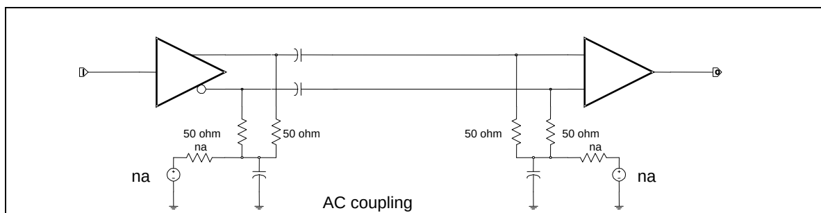
Figure 171 – Common mode biasing for SATA MicroSSD
