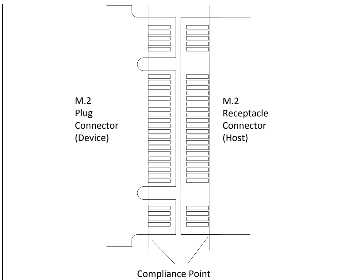
Figure 191 – M.2 compliance point
