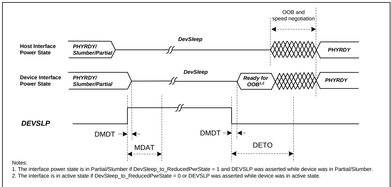
Figure 264 – DEVSLP protocol overview
