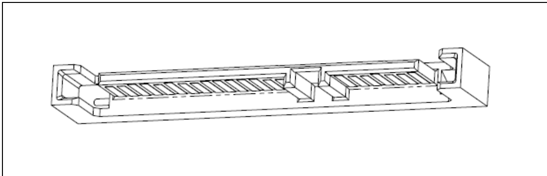
Figure 127 – SATA Express device plug connector isometric drawing
