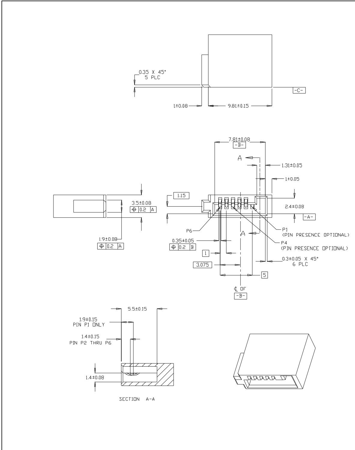
Figure 81 – Slimline power receptacle connector interface dimensions
