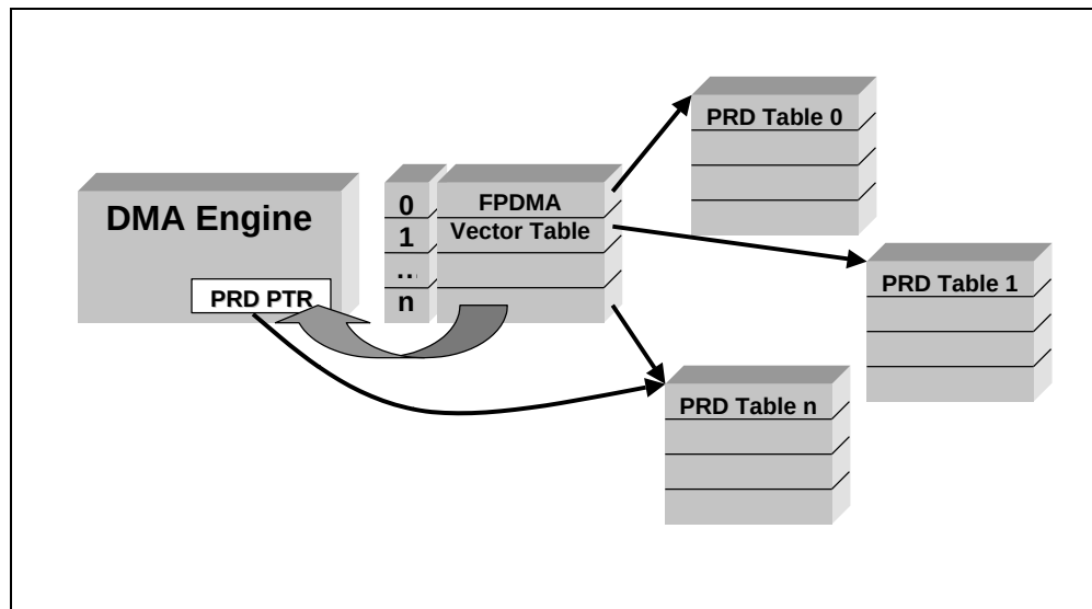
Figure 386 – Example DMA engine indirection for First-party DMA support
