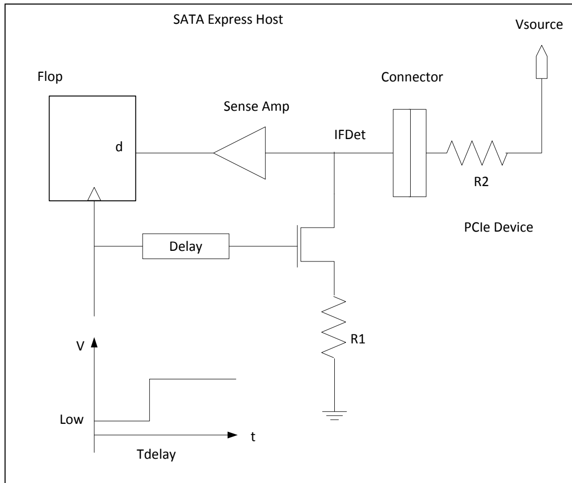
Figure 168 – Interface Detect, shutting down DC path after detection
