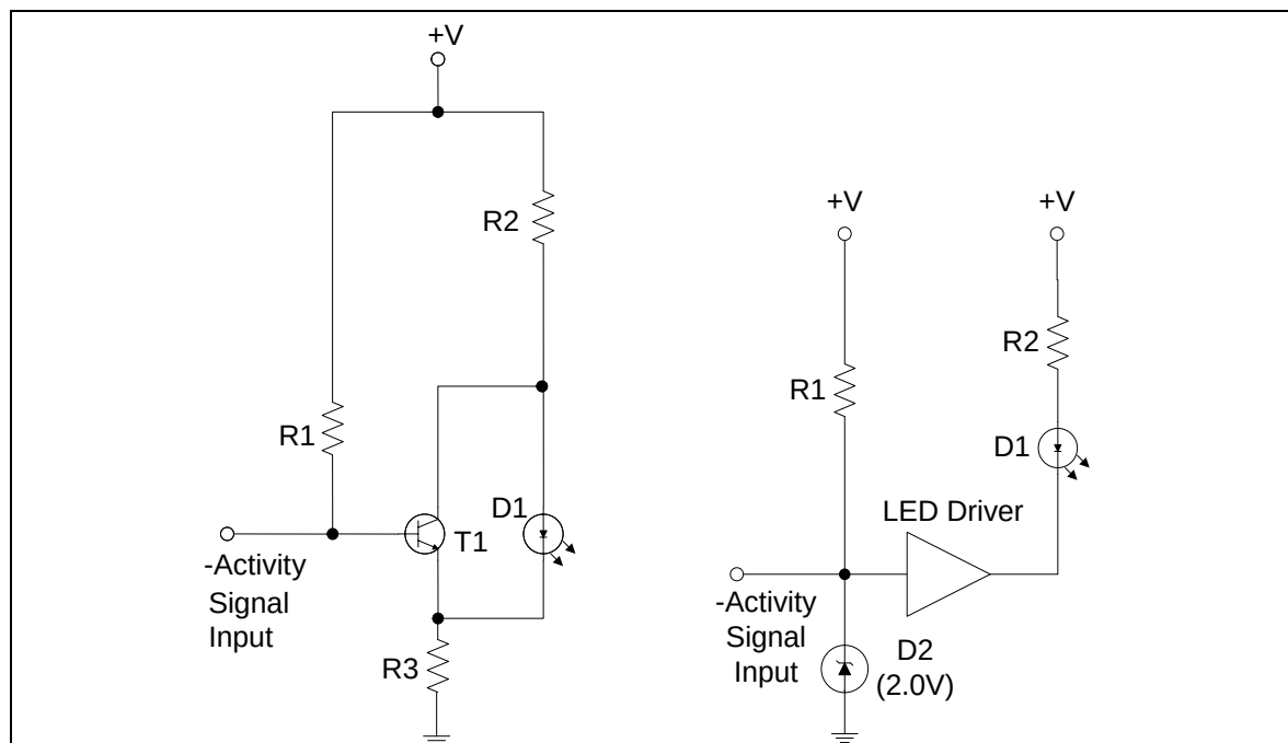
Figure 156 – Example host LED driver circuits
