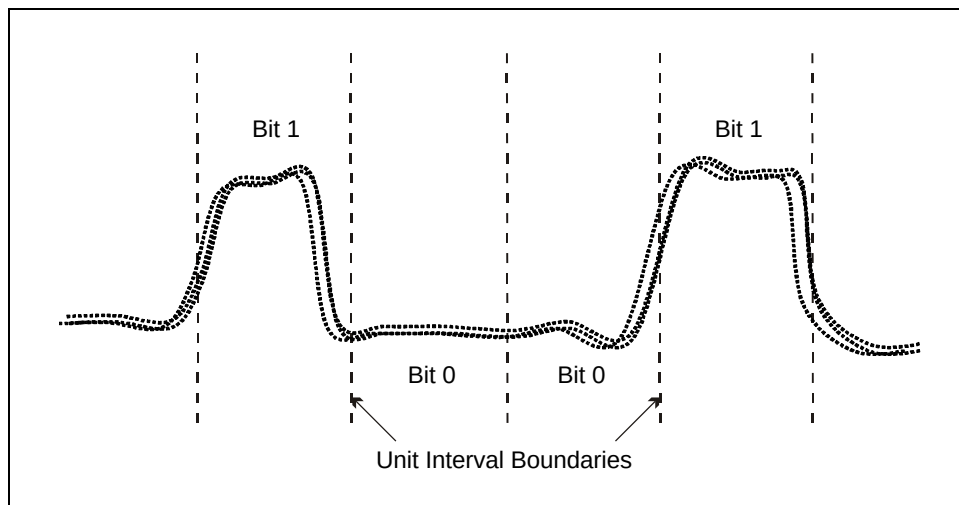
Figure 212 – Differential Voltage amplitude measurement pattern example
