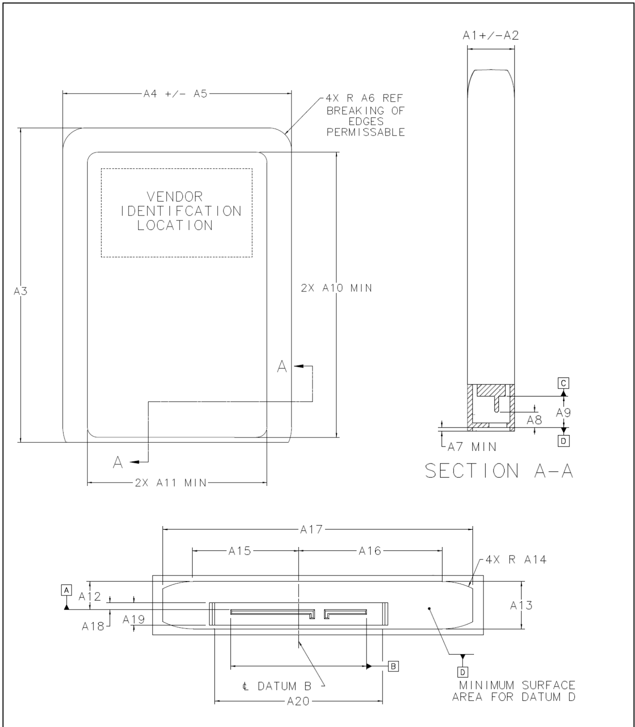
Figure 99 – 14.5 mm SATA USM physical dimensions (see INF-8280)
