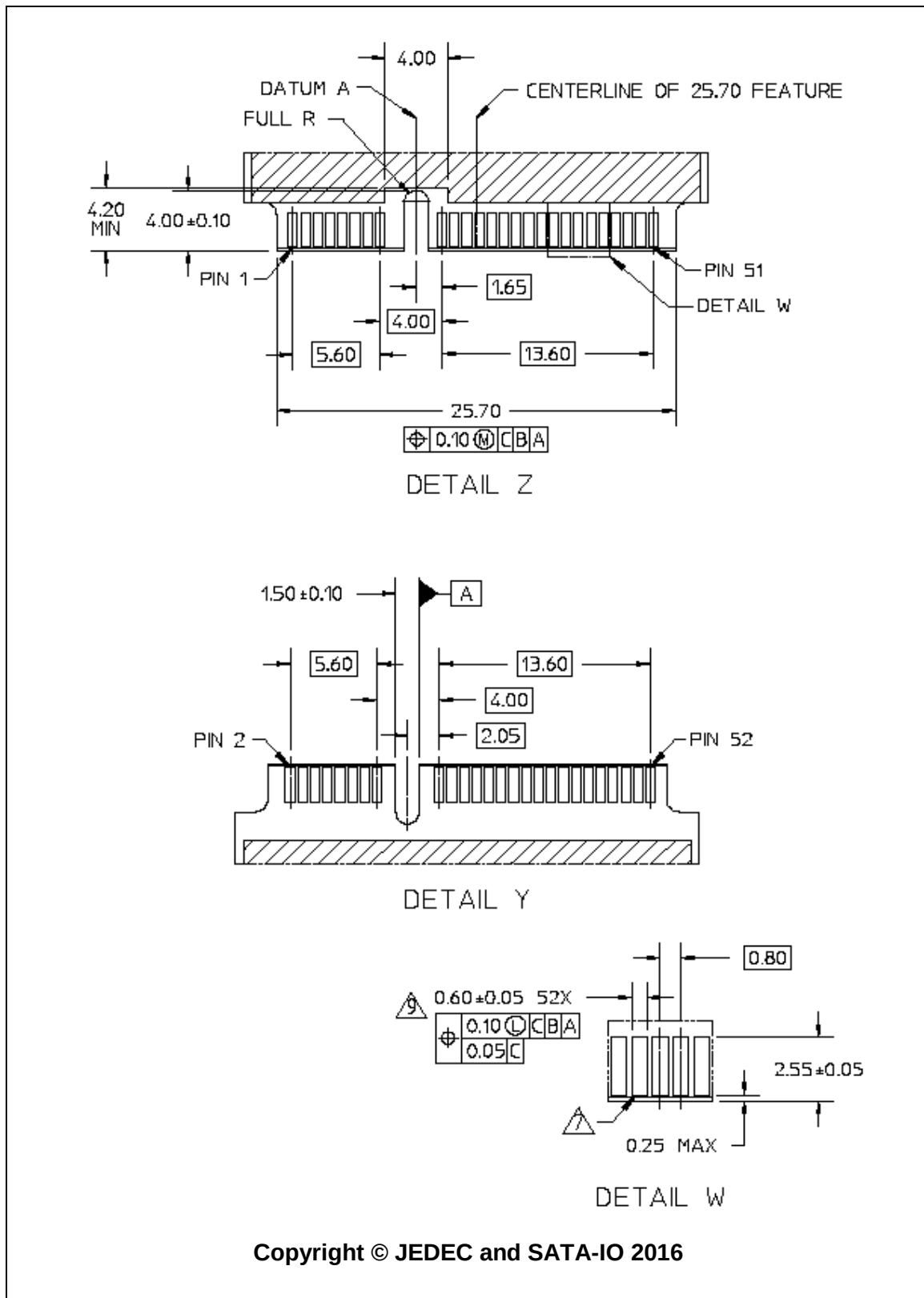
Figure 97 – Device mSATA card type internal connector (informative) (part 2 of 2)
