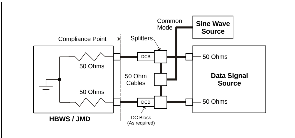
Figure 228 – Receiver jitter and CM tolerance test – setting levels
