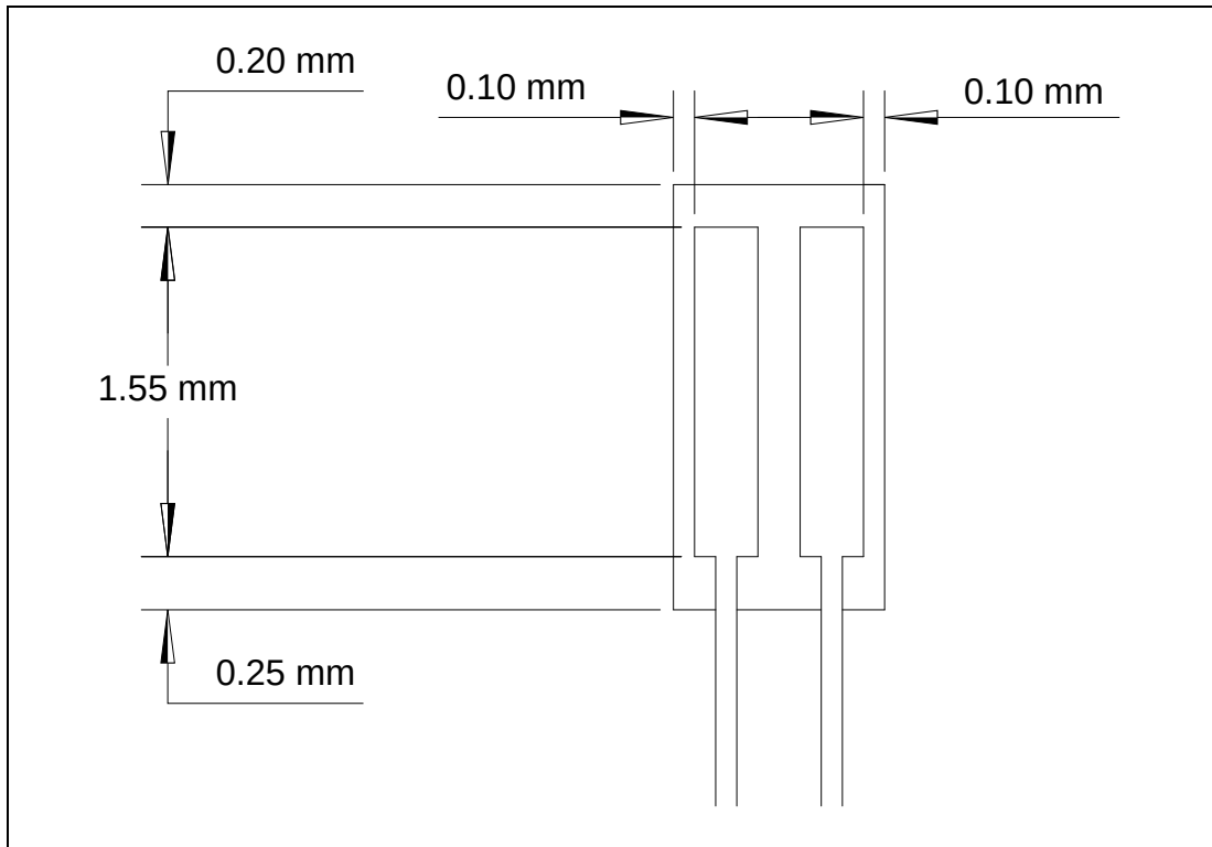
Figure 122 – M.2 mother board pad and void dimensions (informative)
