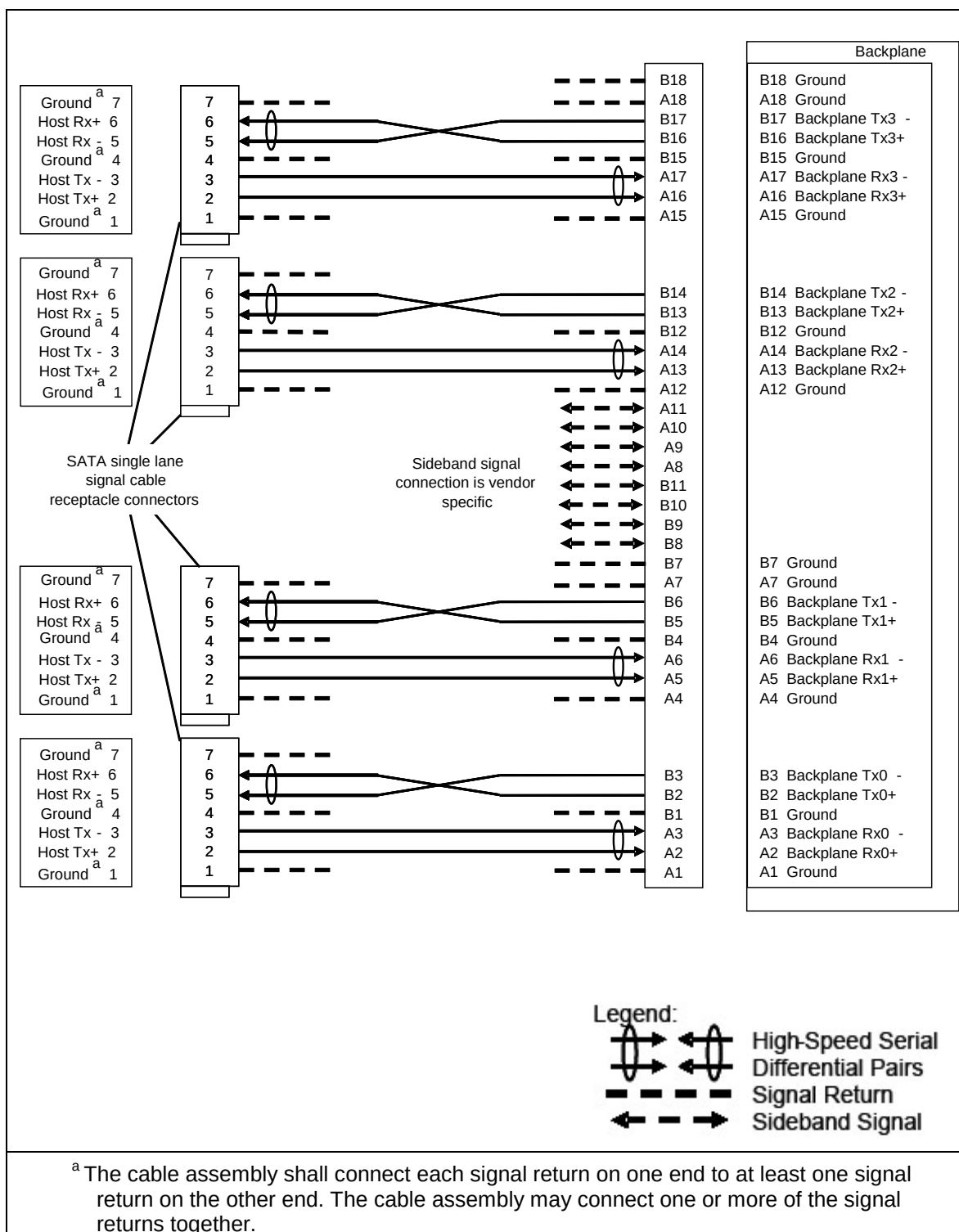
Figure 56 – Mini SATA Internal Multilane system, backplane based fanout cable implementation
