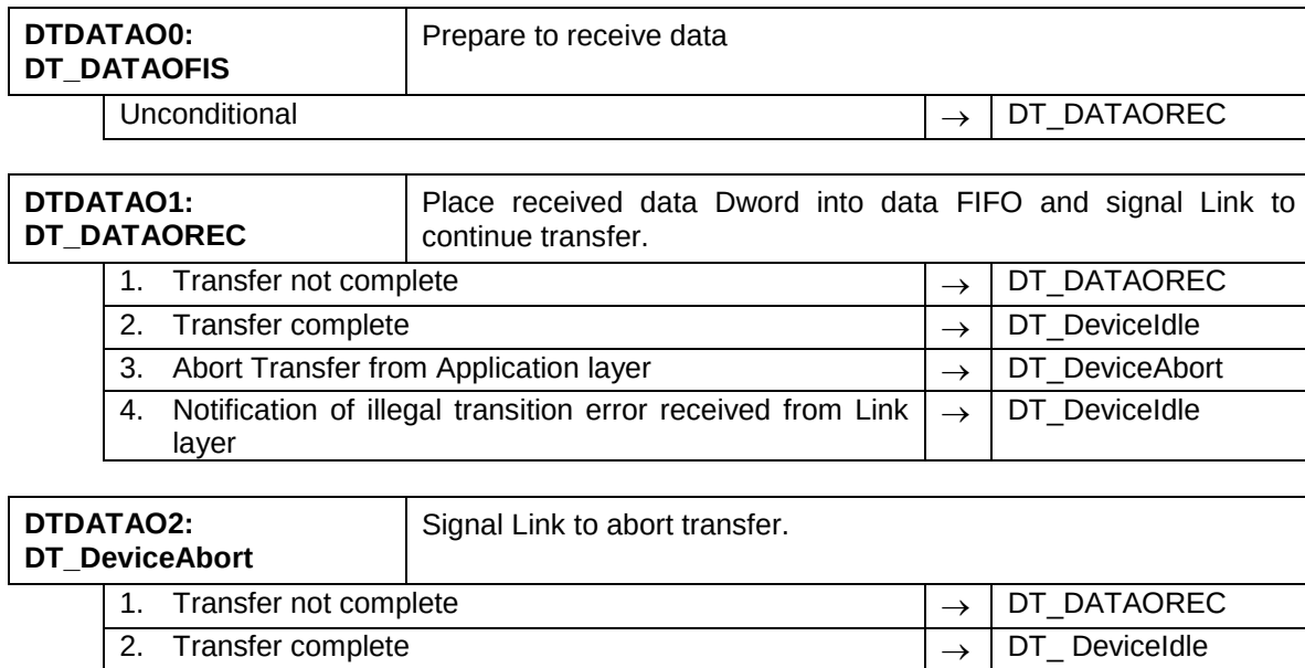
Figure 303 – Device transport data host to device state machine
