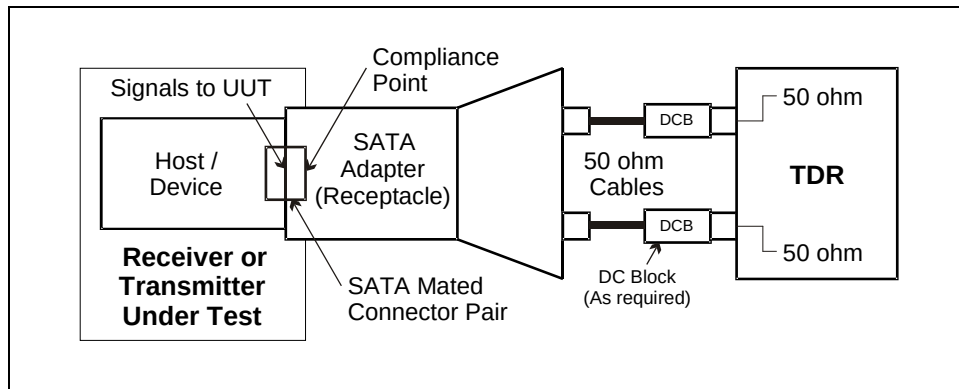
Figure 244 – TDR impedance test
