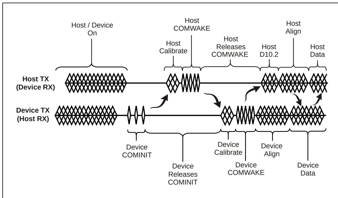
Figure 255 – COMINIT sequence
