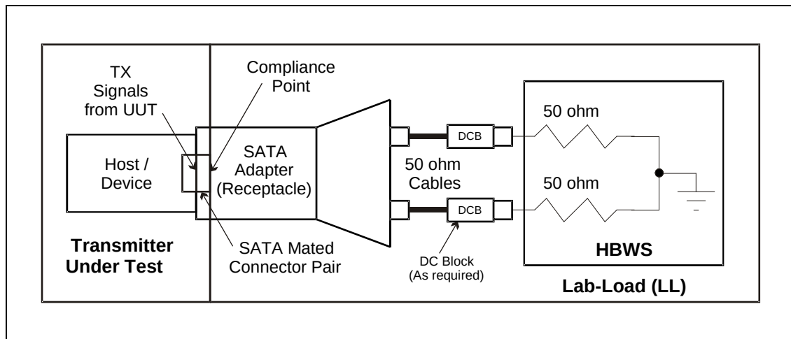
Figure 215 – Transmit amplitude test with Lab-Load (LL)
