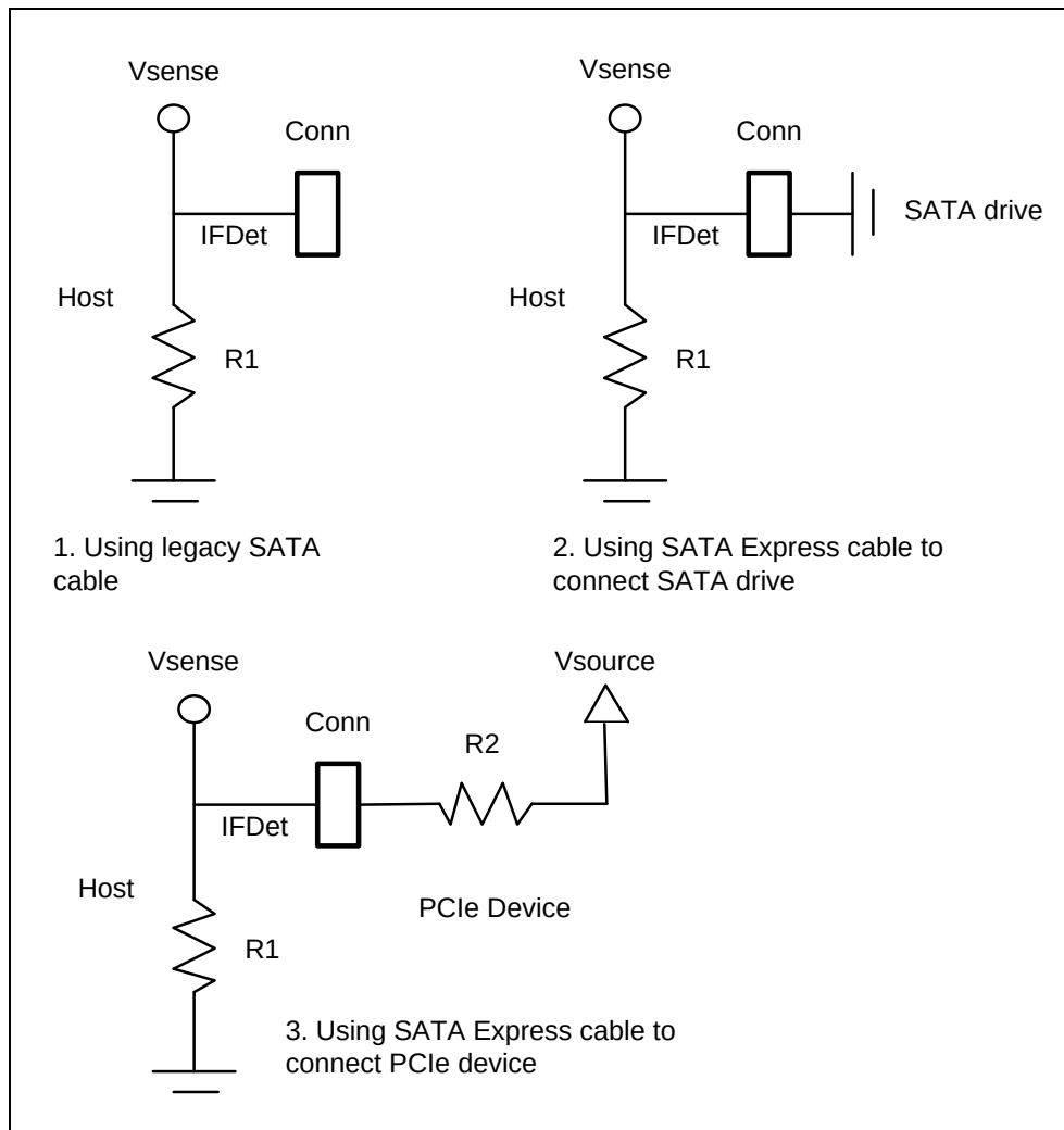
Figure 167 – SATA Express interface detect mechanism
