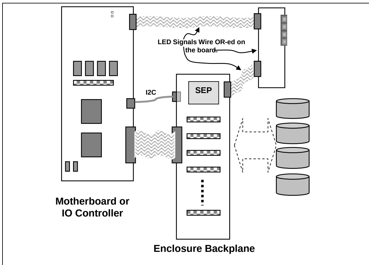
Figure 421 – Device activity LEDs in a storage subsystem
