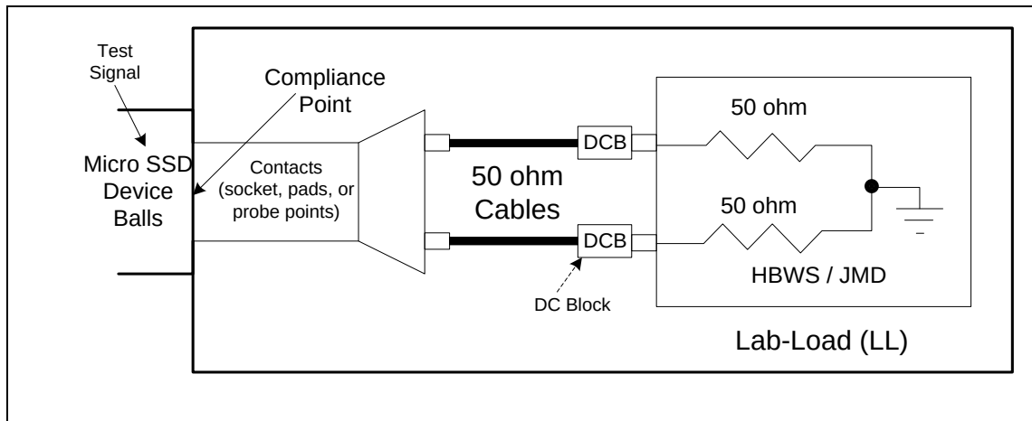
Figure 199 – Lab-Load (LL) for SATA MicroSSD device
