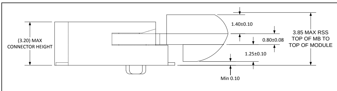
Figure 118 – M.2 double sided assembly – D3 (informative)
