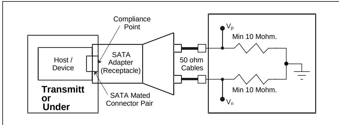
Figure 239 – Tx/Rx sequencing transient Voltage measurement
