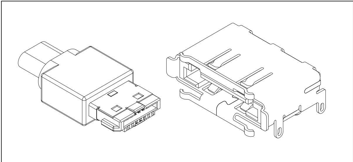
Figure 142 – Renderings of External Serial ATA cable receptacle and right angle plug
