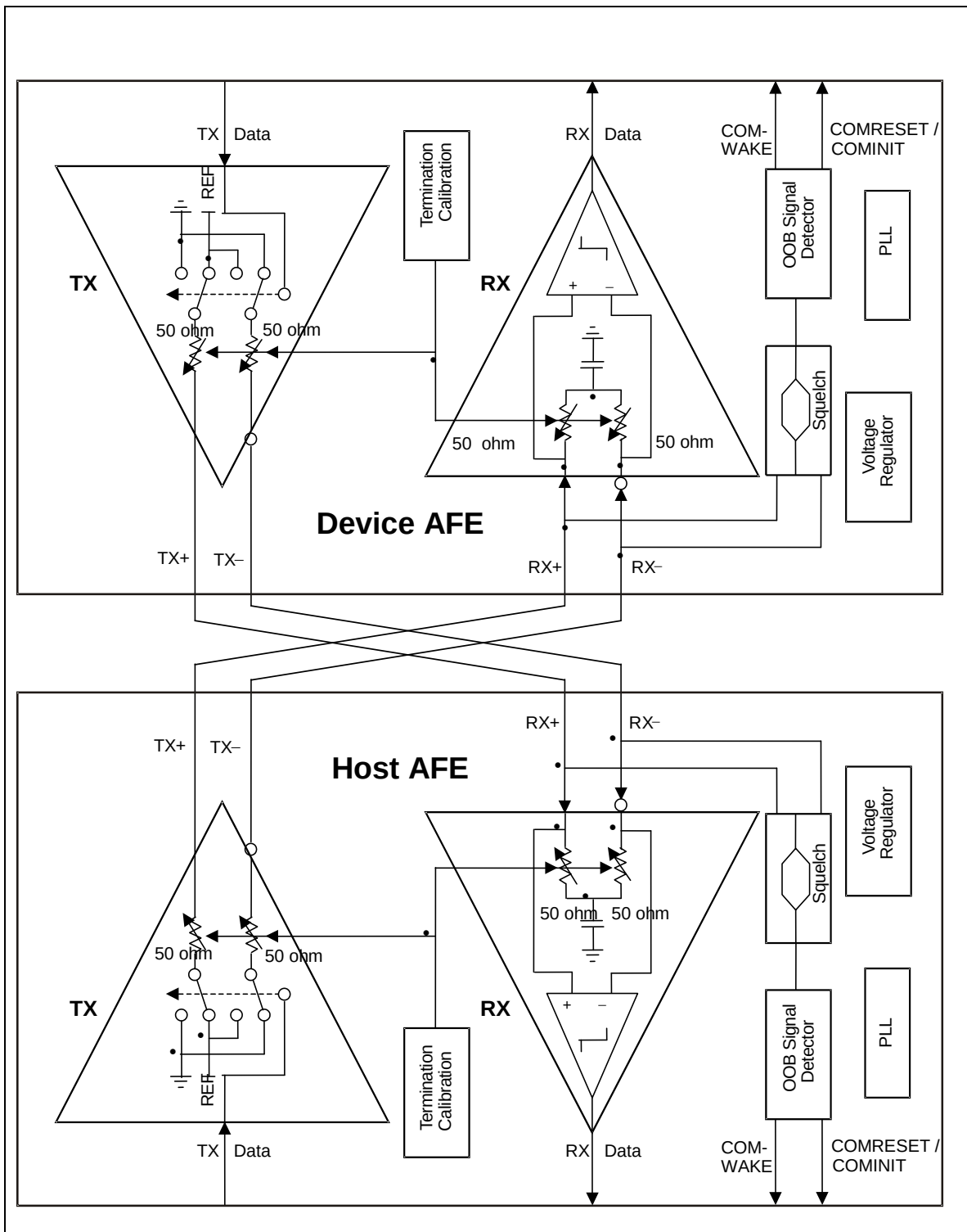
Figure 164 – Analog Front End (AFE) cabling
