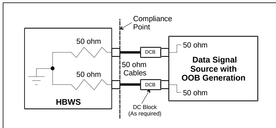
Figure 241 – Squelch detector threshold test – setting levels
