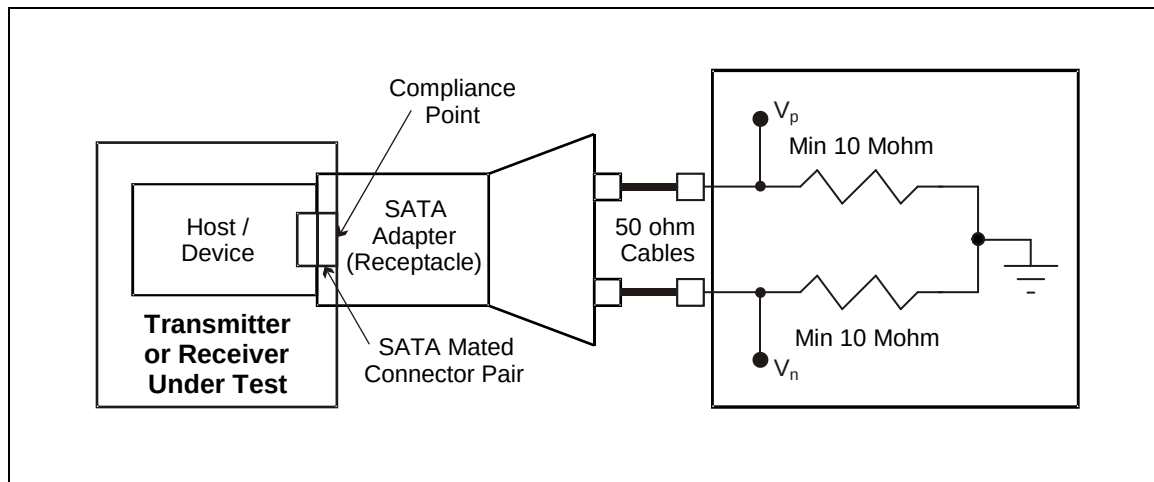
Figure 246 – DC coupled common mode Voltage measurement
