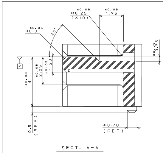
Figure 69 – 7.0 mm Slimline device plug connector interface dimensions section A-A
