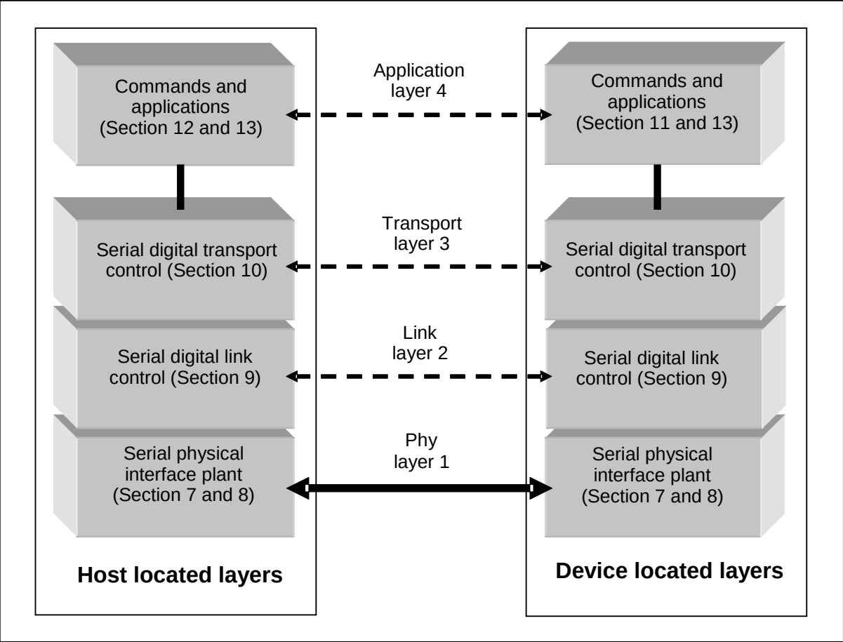
Figure 5 – Communication layers
