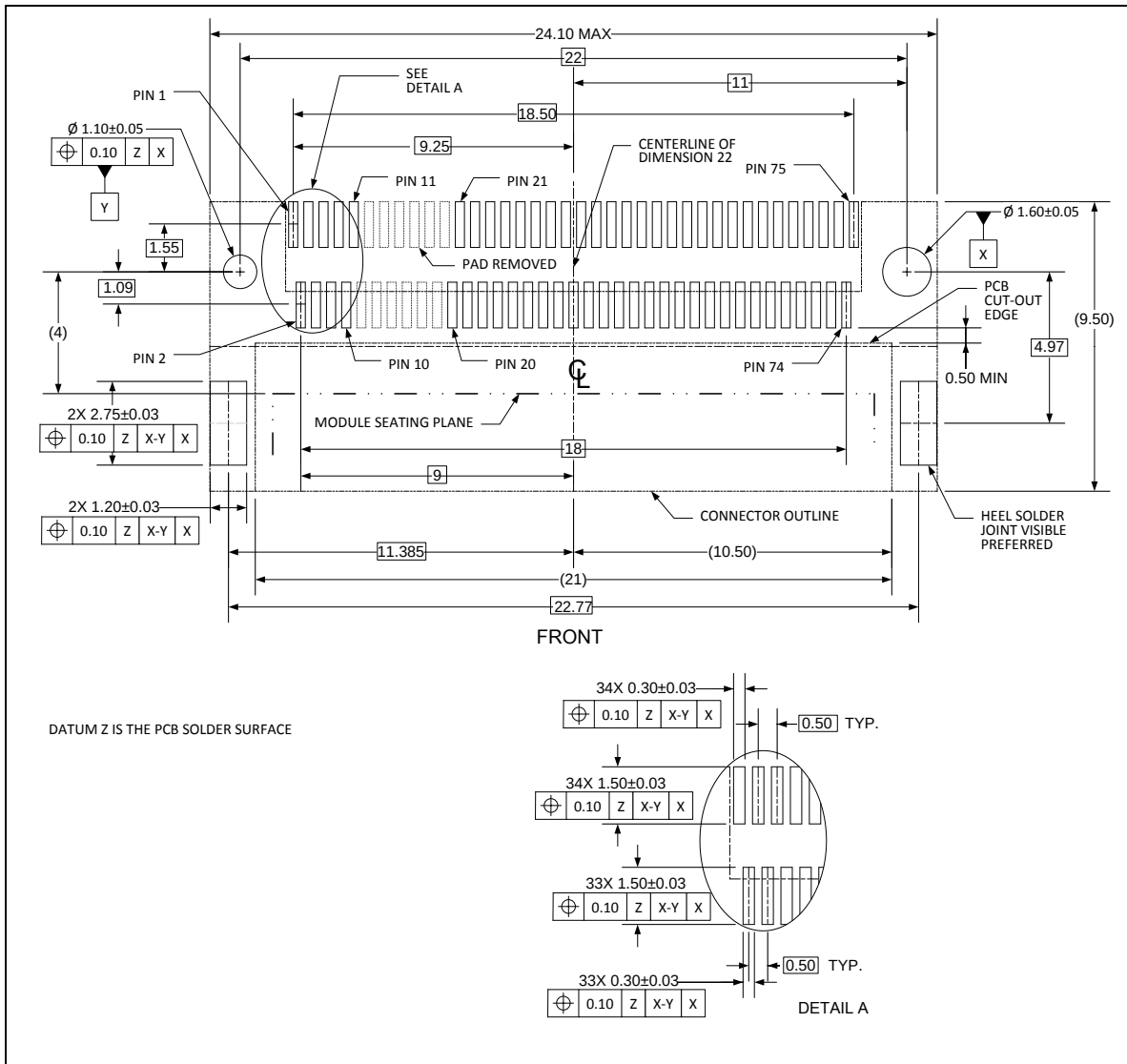
Figure 115 – M.2 land pattern for mother board (informative)
