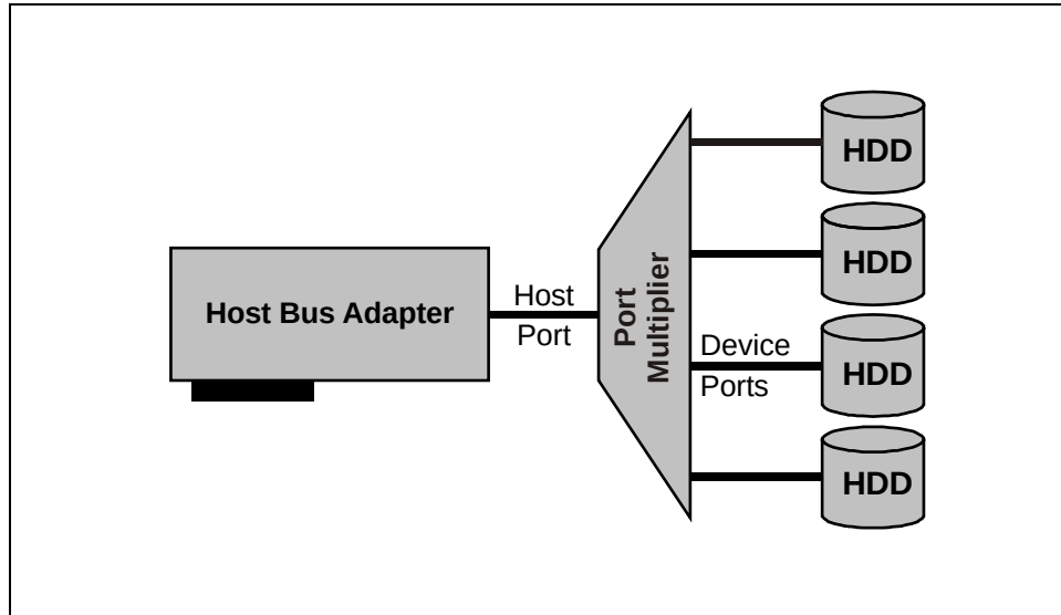
Figure 433 – Port Multiplier overview
