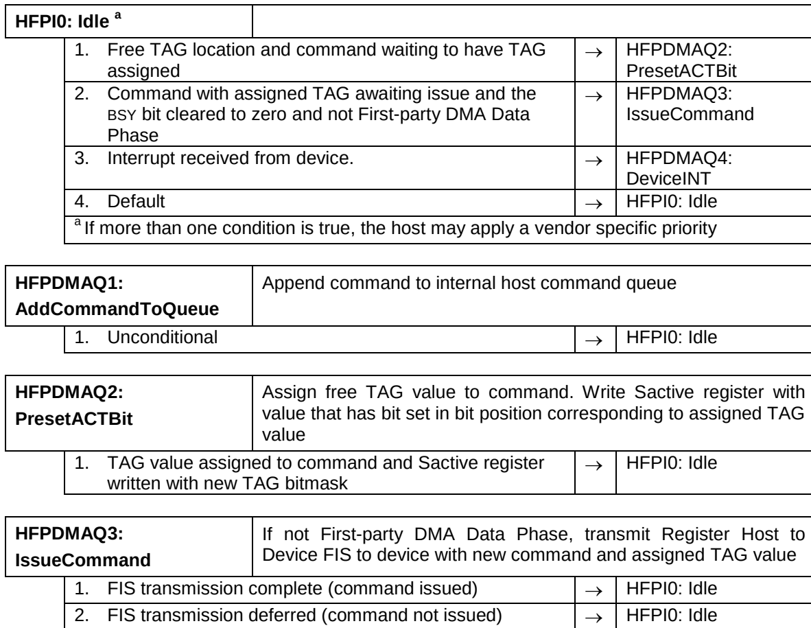
Figure 335 – Host command layer FPDMA queued state machine
