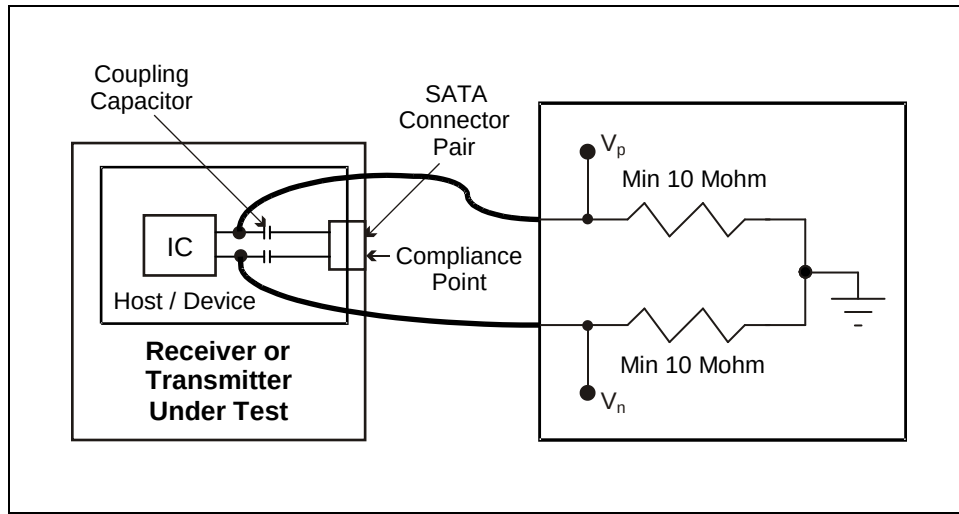
Figure 247 – AC coupled common mode Voltage measurement
