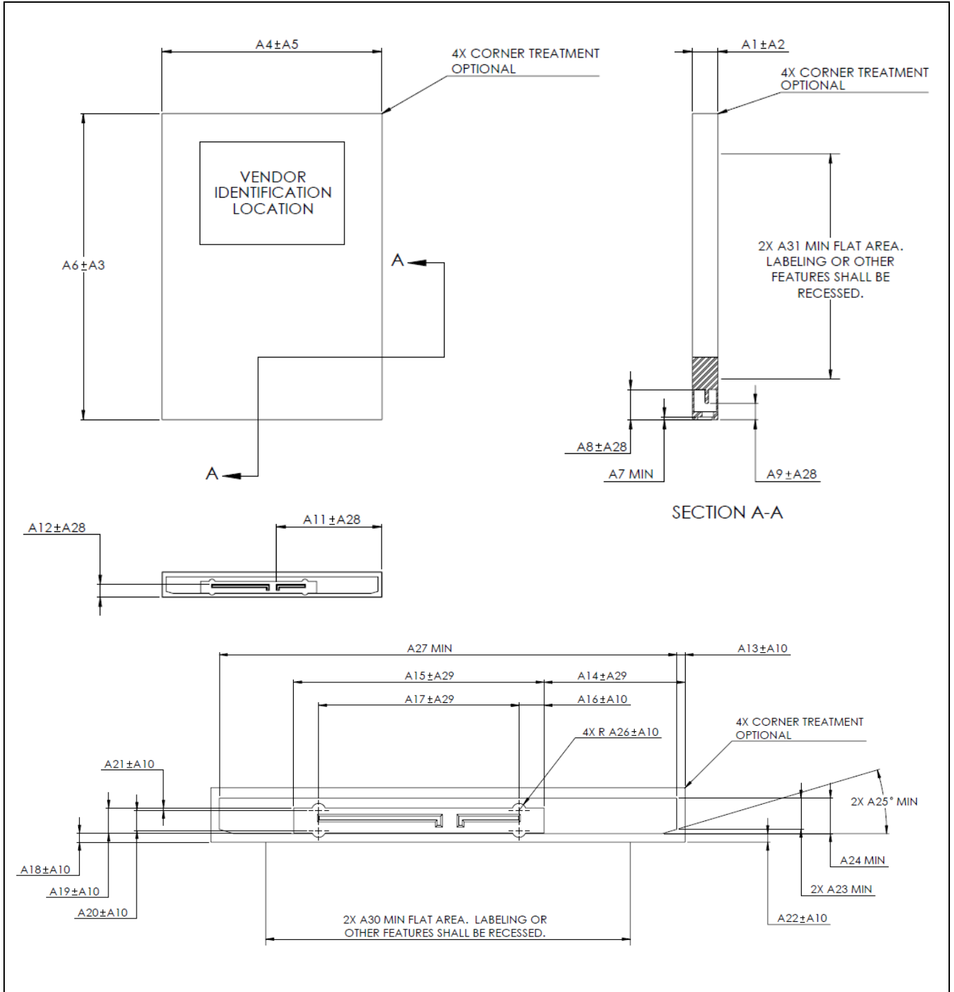
Figure 100 – 9 mm SATA USM physical dimensions (see INF-8280)
