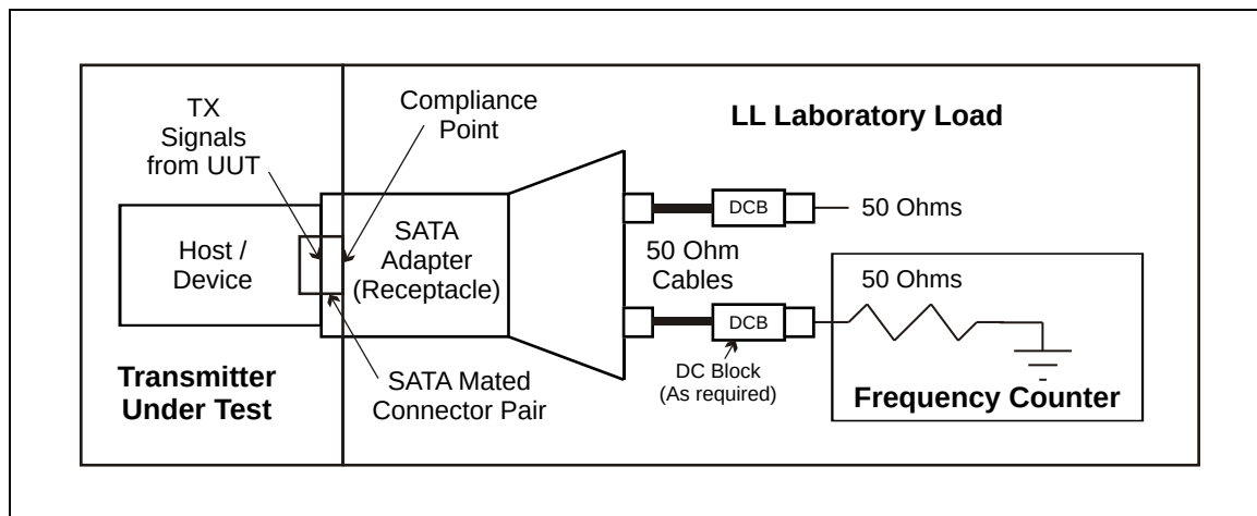
Figure 221 – Tx long term frequency measurement
