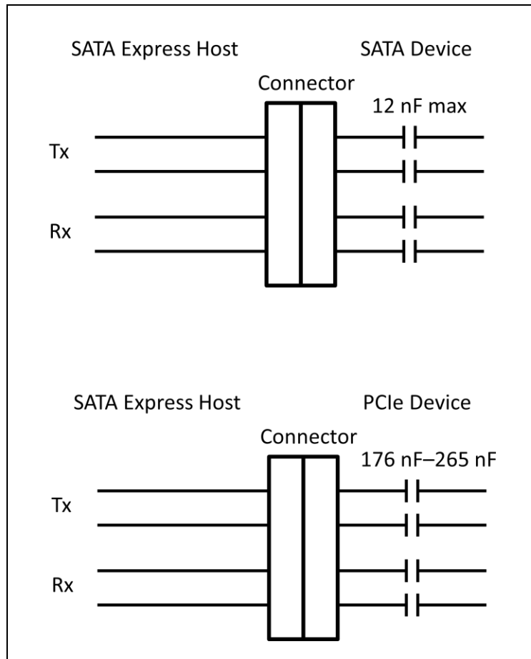
Figure 166 – AC coupling capacitor requirements
