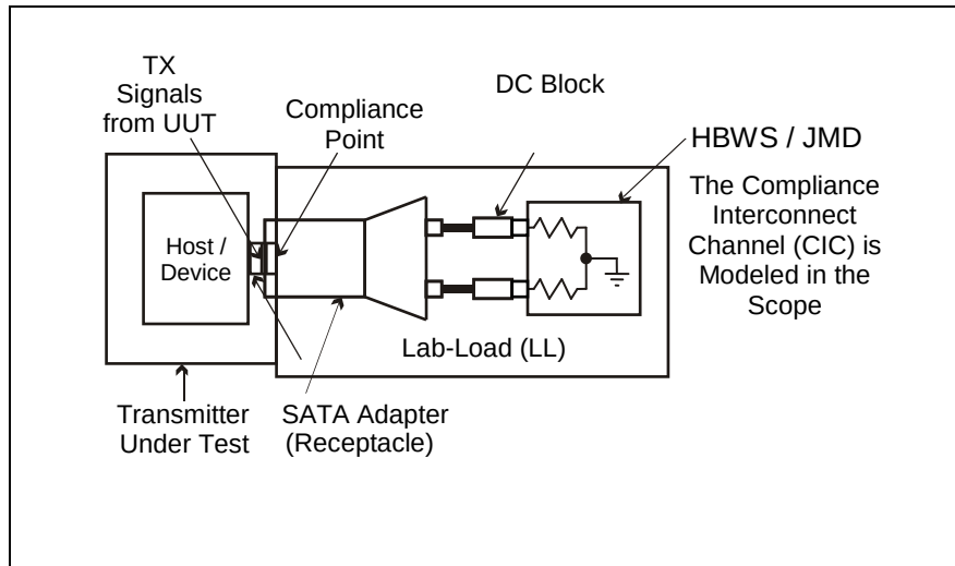
Figure 217 – Transmit amplitude test with simulated CIC
