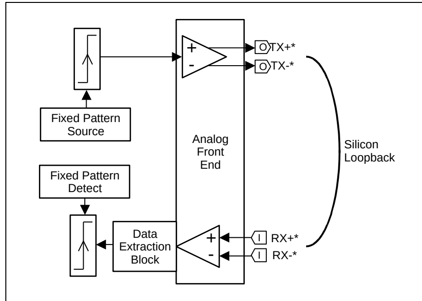
Figure 184 – Near-End Analog Loopback
