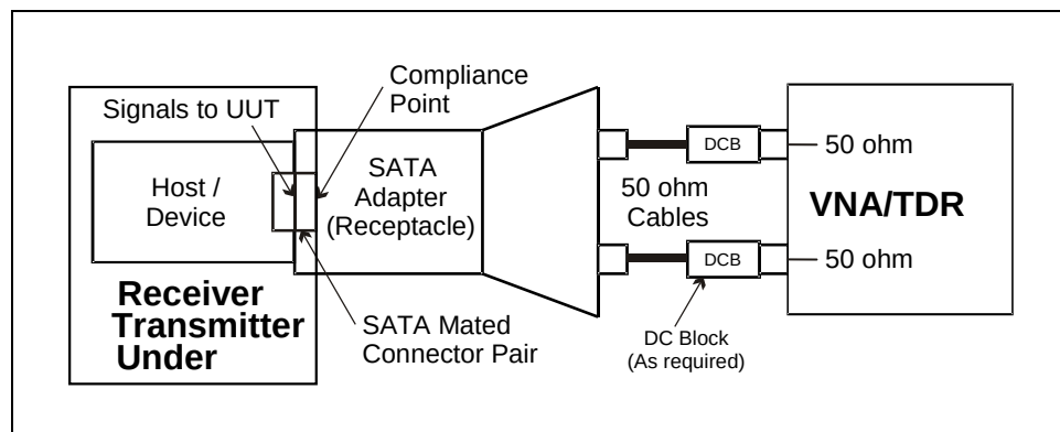
Figure 234 – Return loss test
