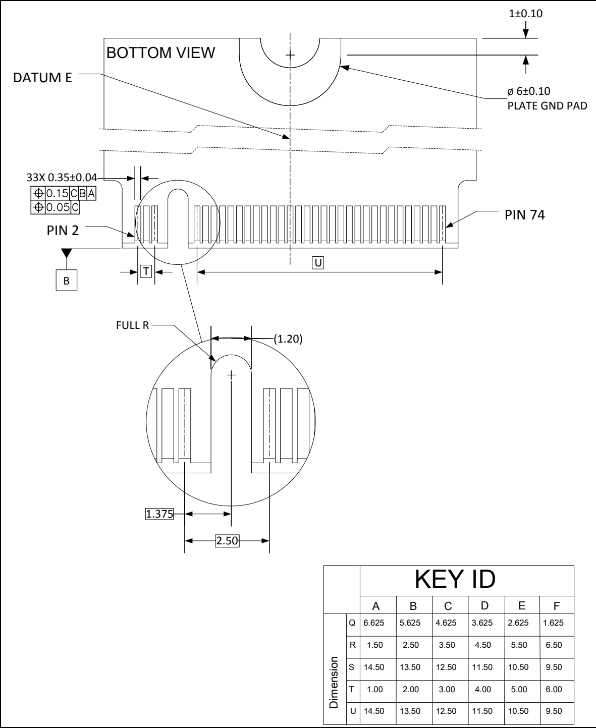
Figure 113 – M.2 board connector bottom slot details (informative)
