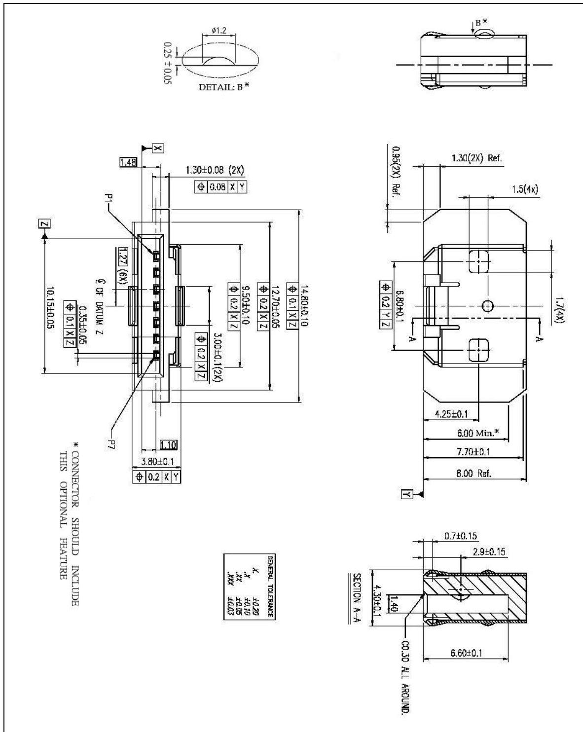
Figure 143 – Mechanical dimensions of External Serial ATA cable receptacle assembly
