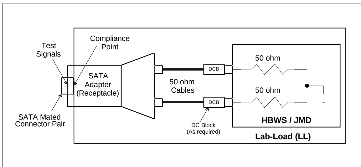
Figure 195 – Lab-Load (LL)
