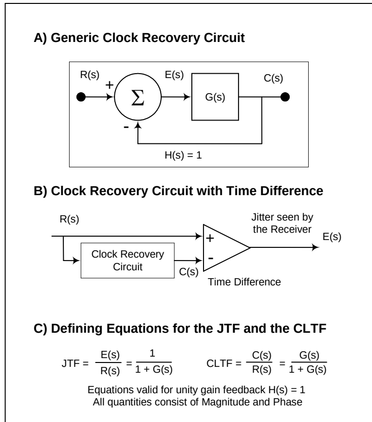
Figure 225 – JTF and CLTF definition
