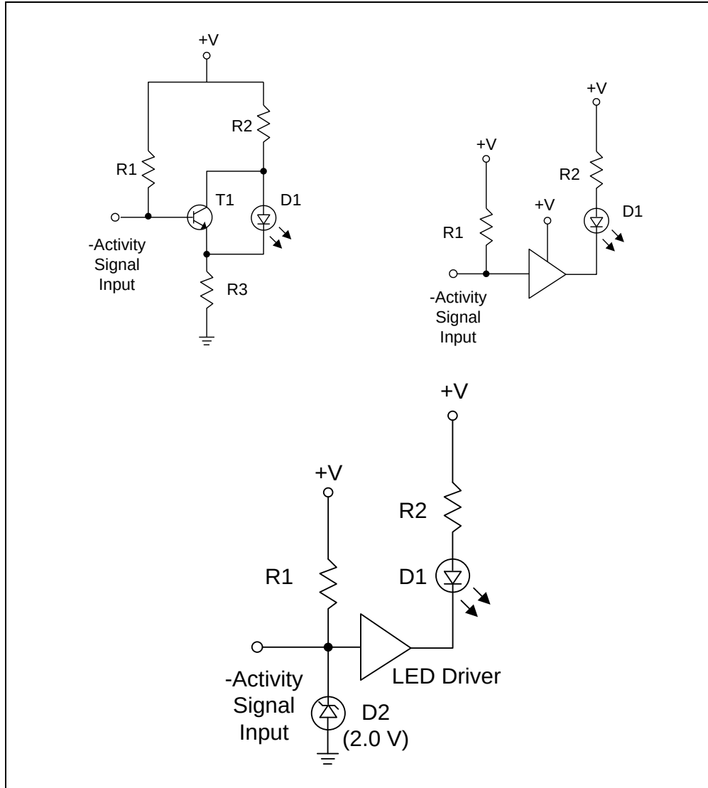
Figure 159 – Example host LED driver circuits
