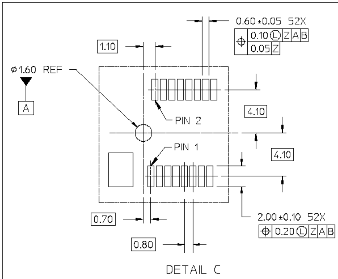
Figure 96 – mSATA card connector location detail C (informative)
