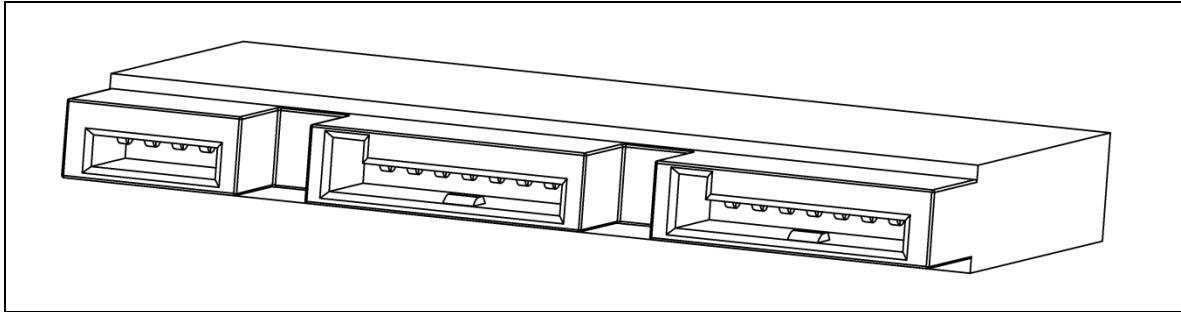
Figure 135 – SATA Express host cable receptacle connector isometric drawing
