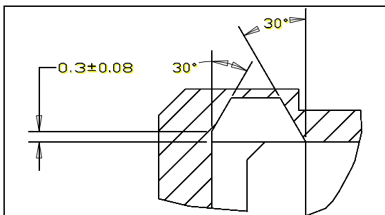
Figure 77 – Slimline device plug connector interface dimensions (detail D)
