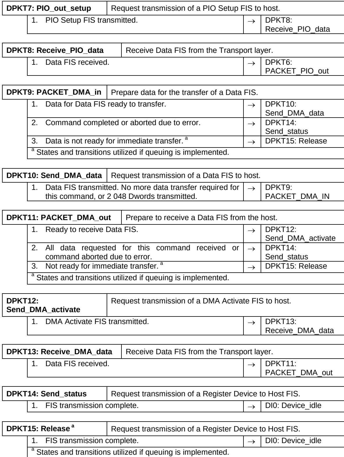
Figure 331 – Device command layer packet state machine (part 2 of 2)
