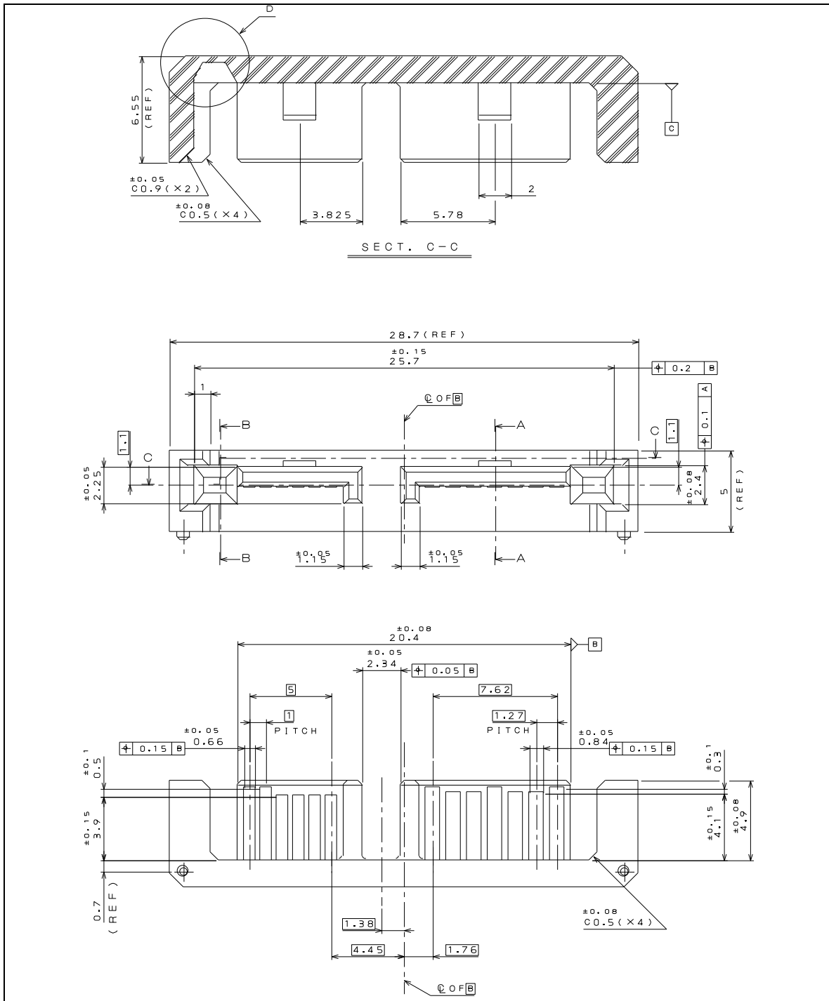
Figure 68 – 7.0 mm Slimline device plug connector interface dimensions
