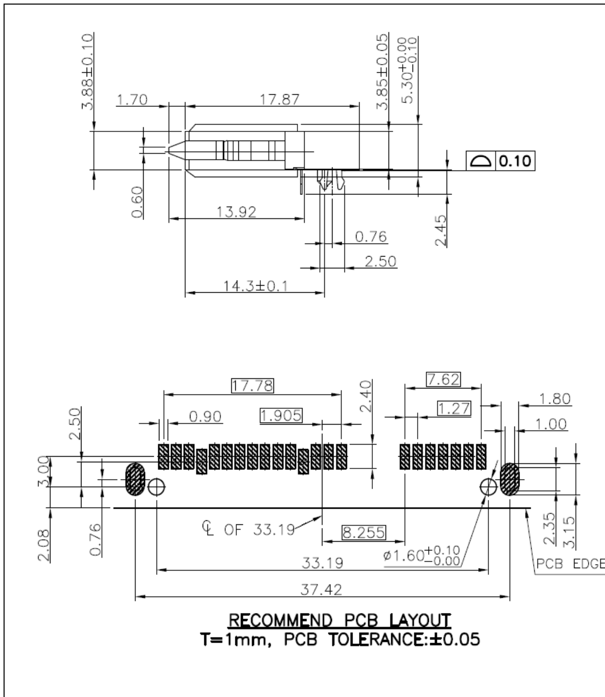
Figure 104 – SATA USM horizontal receptacle continued (see INF-8280)
