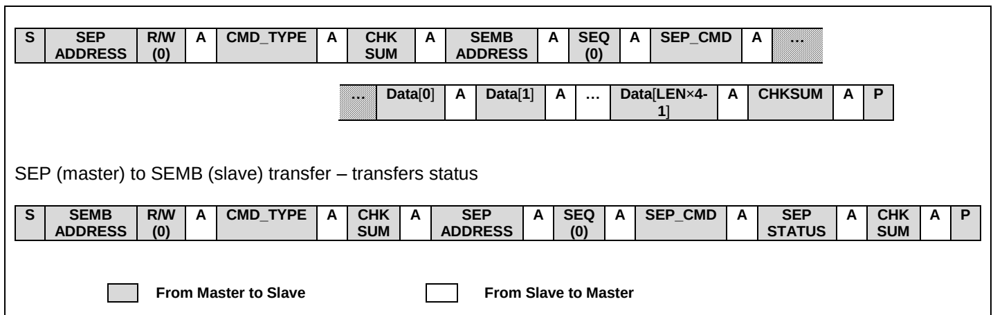
Figure 409 – I 2 C transactions corresponding to a WRITE SEP command
