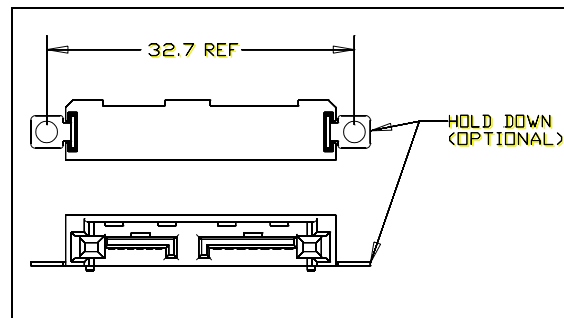
Figure 79 – Slimline device plug connector optional hold down mounting
