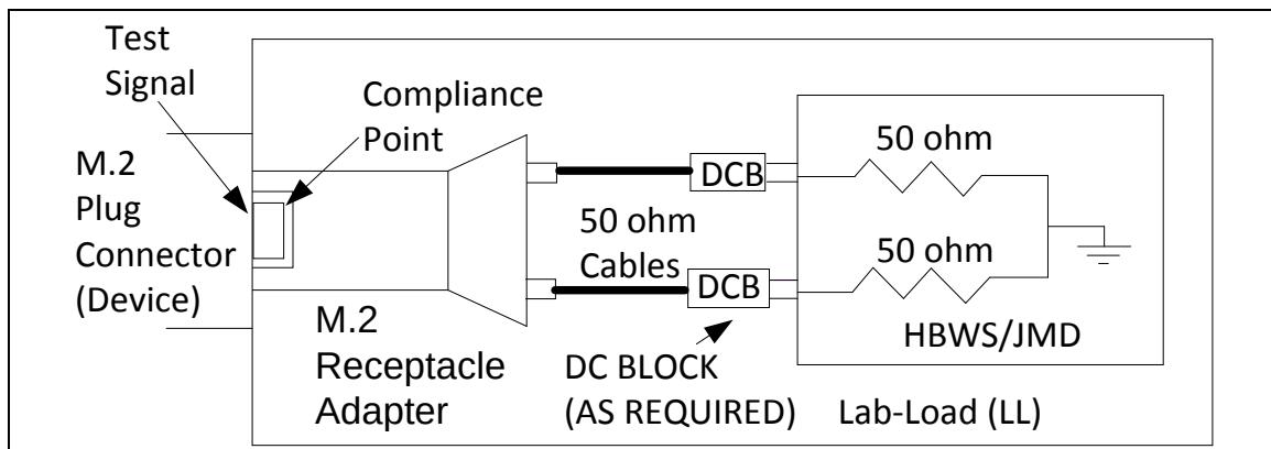
Figure 201 – Lab-Load (LL) for M.2 device
