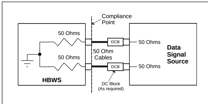
Figure 218 – Receiver amplitude test, setting levels
