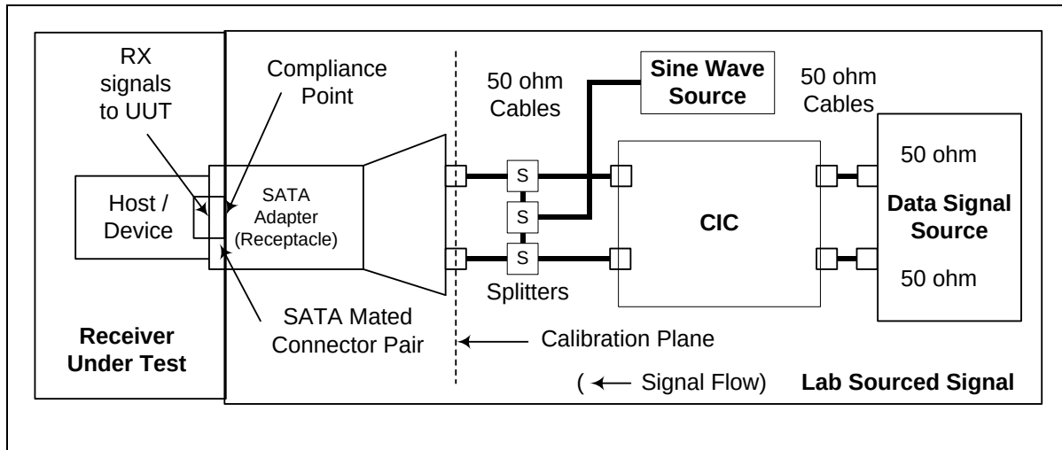
Figure 232 – Receiver jitter and CM tolerance test (Gen3i)
