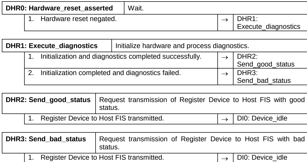
Figure 306 – Device command layer reset state machine
