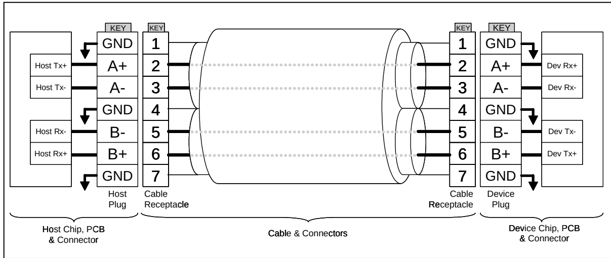
Figure 21 – SATA cable / connector connection diagram
