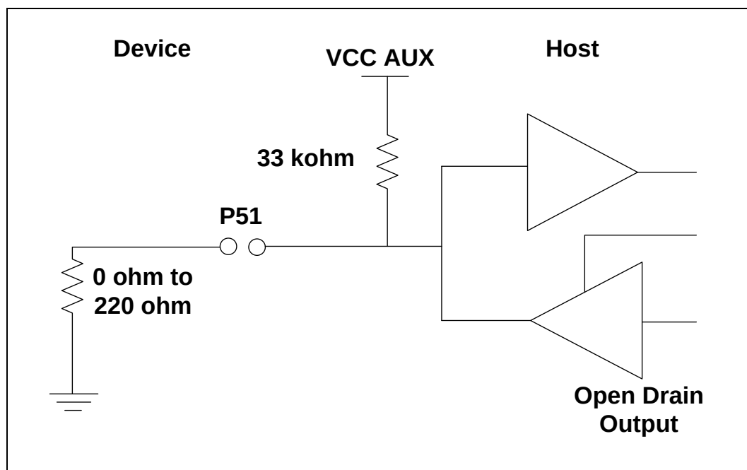
Figure 98 – Bi-directional host side implementation of P51 for compatibility with non-mSATA devices (informative)
