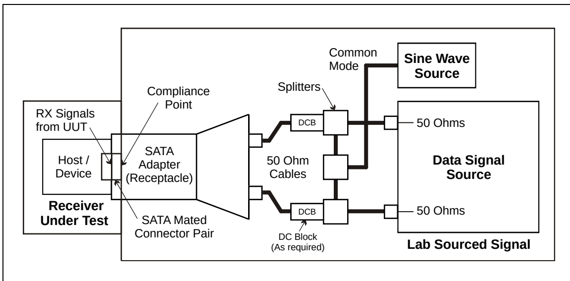
Figure 229 – Receiver jitter and CM tolerance test
