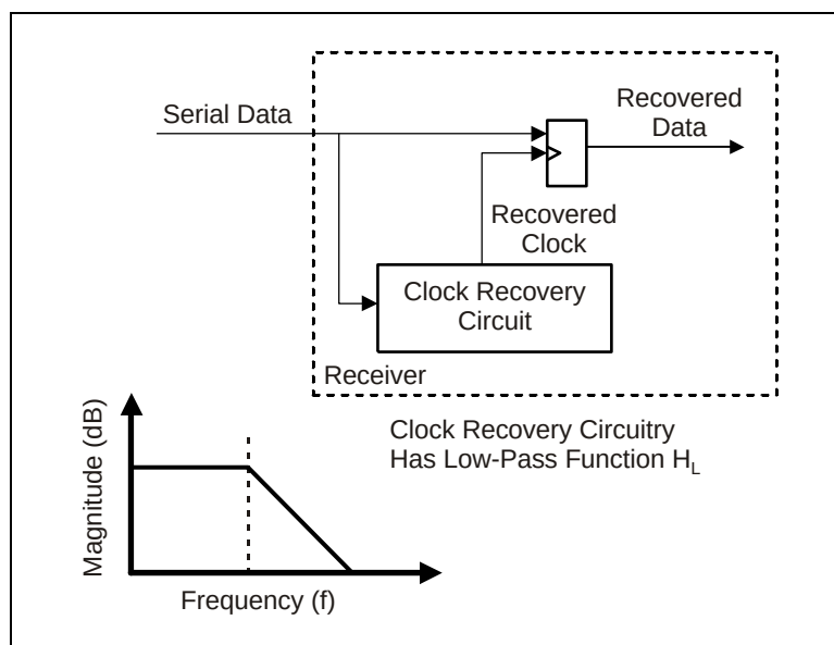
Figure 222 – Receiver model for jitter
