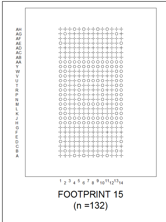
Figure 109 – Footprint 15, SATA MicroSSD variant AR, DB, and DC, 132 balls (informative)
