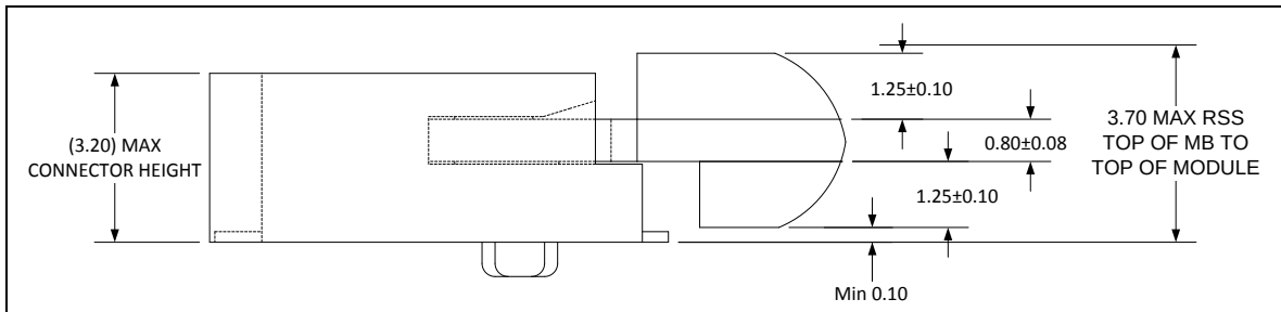
Figure 117 – M.2 double sided assembly – D2 (informative)
