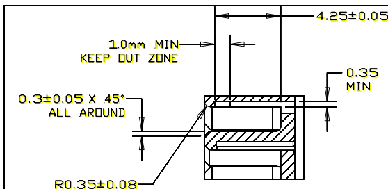
Figure 76 – Slimline device plug connector interface dimensions (section C-C)
