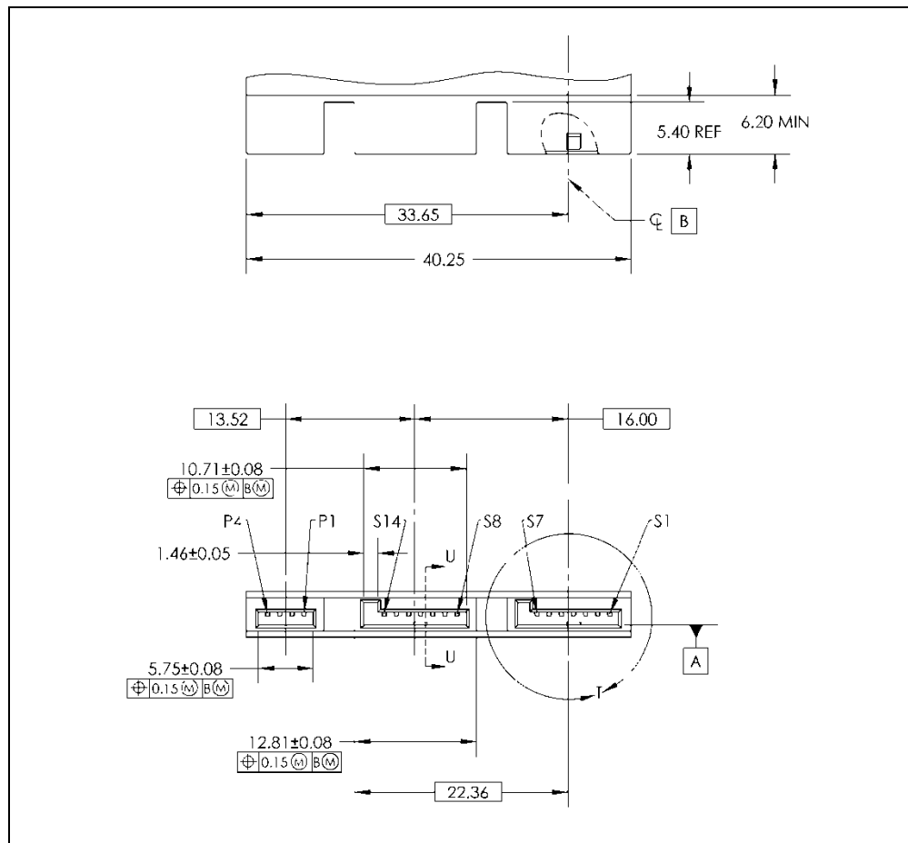
Figure 136 – SATA Express host cable receptacle connector drawing
