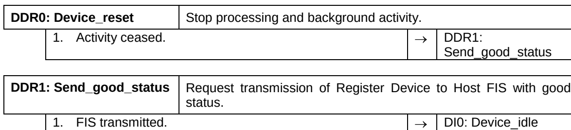
Figure 324 – Device command layer reset state machine
