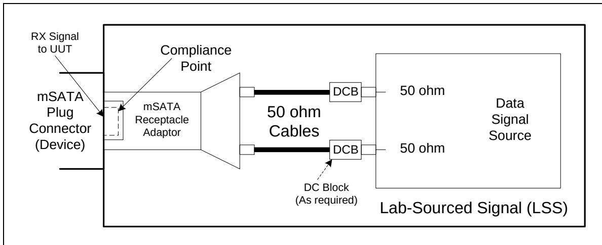
Figure 204 – Lab-Sourced Signal (LSS) for mSATA device
