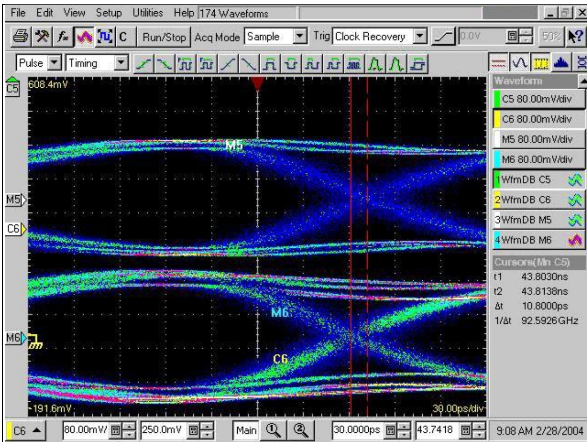
Figure 238 – Example intra-pair skew test for transmitter (10.8 ps)
