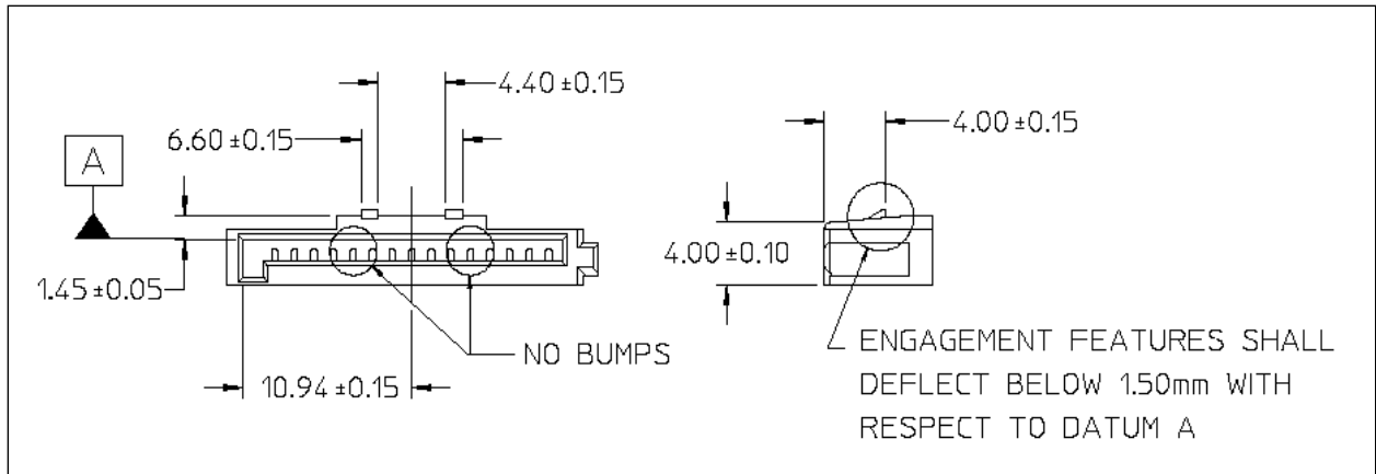
Figure 82 – Slimline power receptacle connector option with latch
