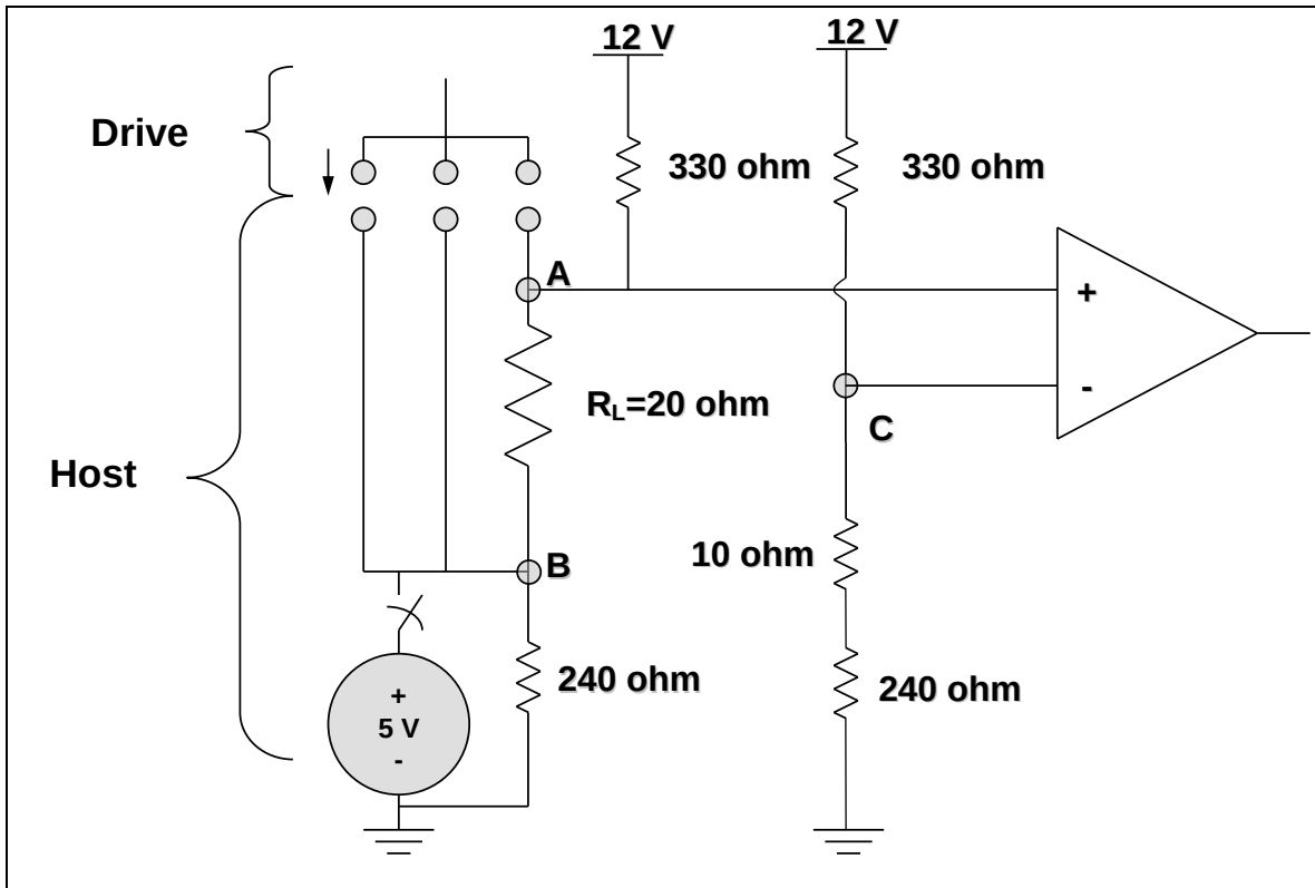
Figure 161 – Example presence detection implementation
