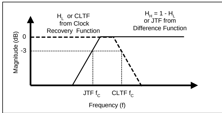
Figure 224 – Jitter at receiver, high pass function
