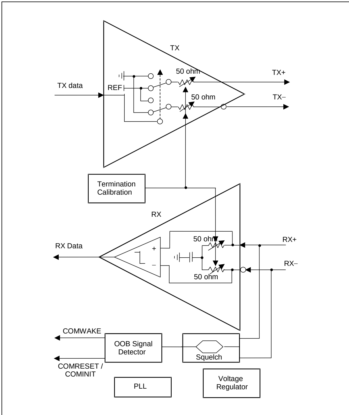
Figure 163 – Analog Front End (AFE) block diagram
