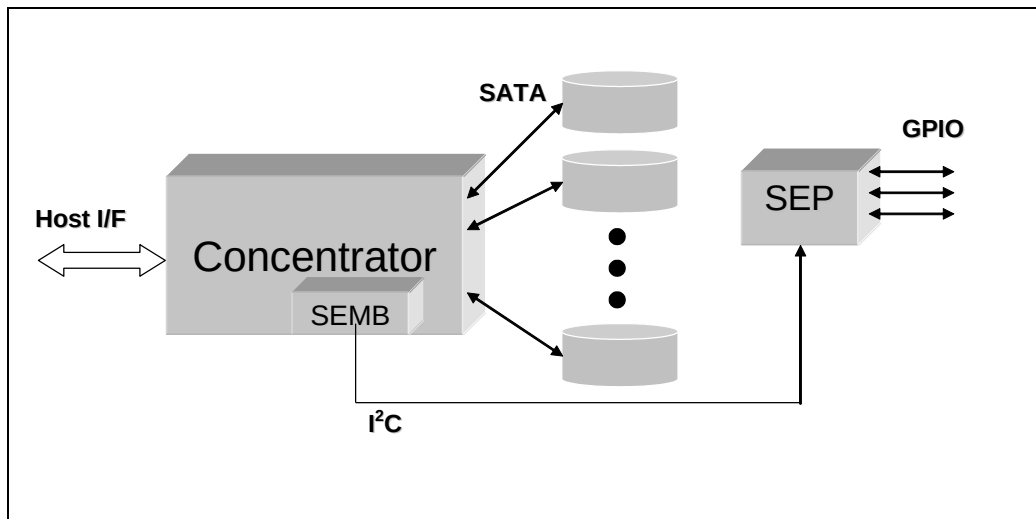
Figure 401 – Generic enclosure services topology
