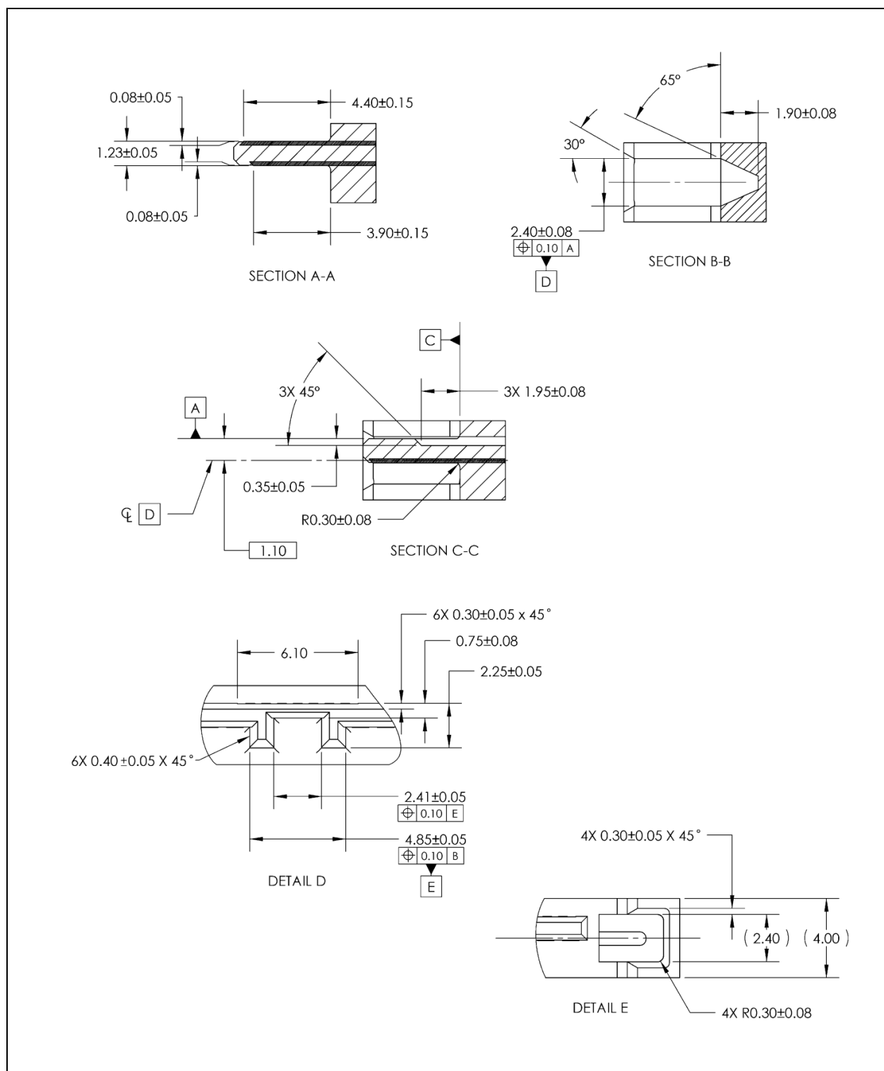
Figure 128 – SATA Express device plug connector drawing (part 2 of 2)
