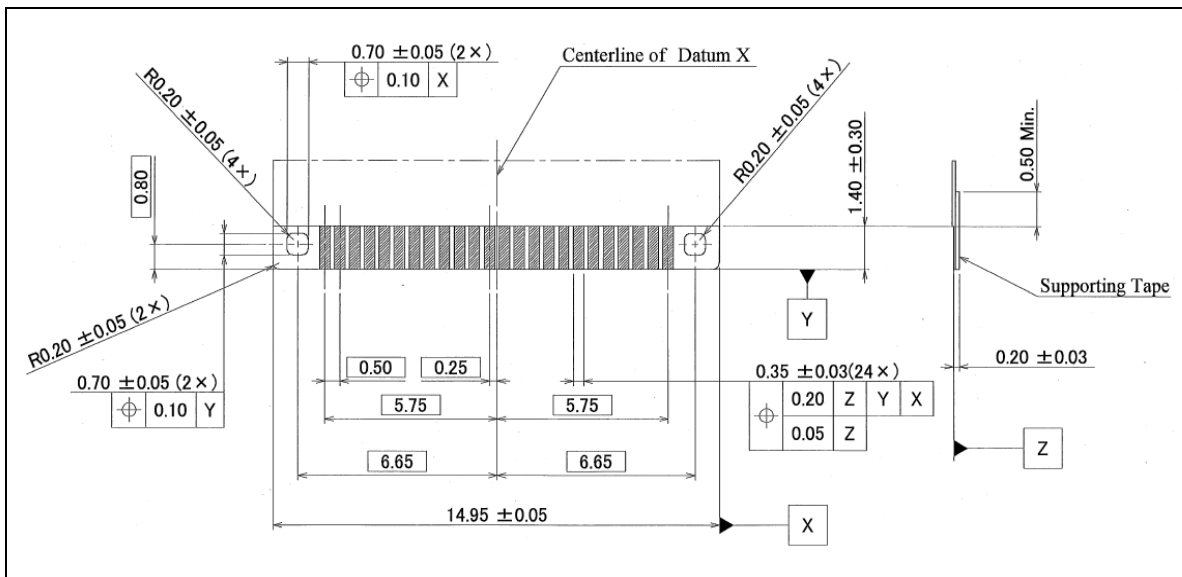
Figure 93 – FPC for internal LIF-SATA
