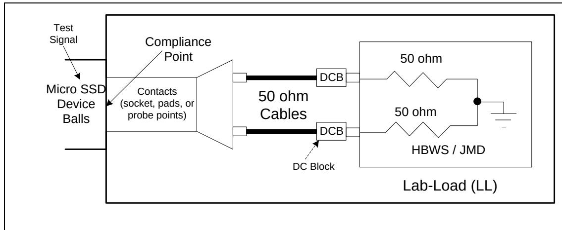
Figure 200 – Lab-Load (LL) for SATA MicroSSD host
