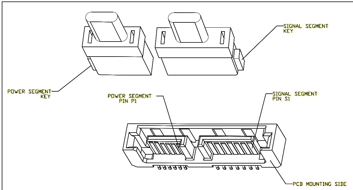
Figure 80 – Slimline connector pin and feature locations
