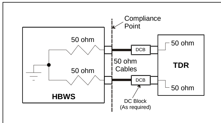
Figure 245 – TDR single-ended impedance test – setting risetime
