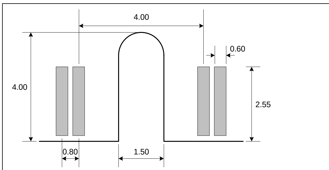
Figure 190 – mSATA connector pin detail
