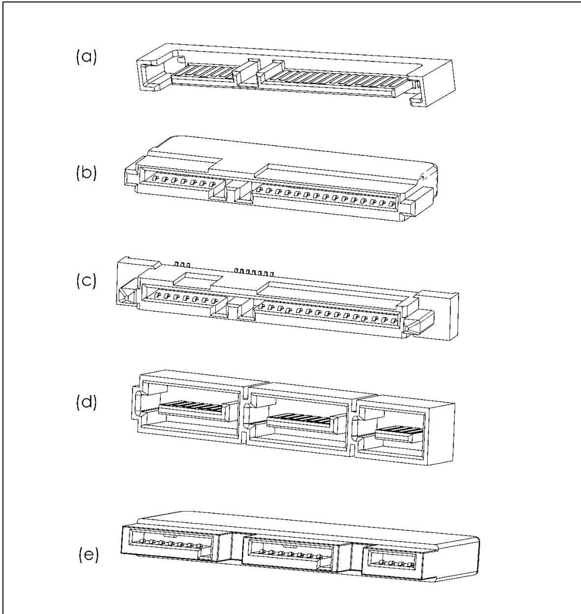
Figure 126 – Examples of SATA Express connectors
