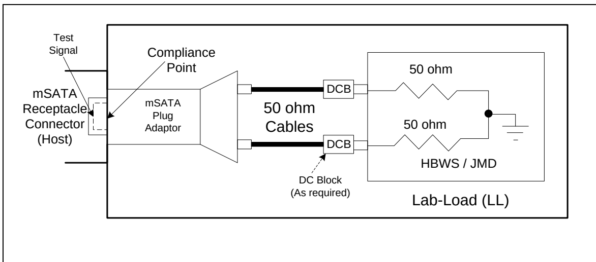
Figure 197 – Lab-Load (LL) for mSATA host
