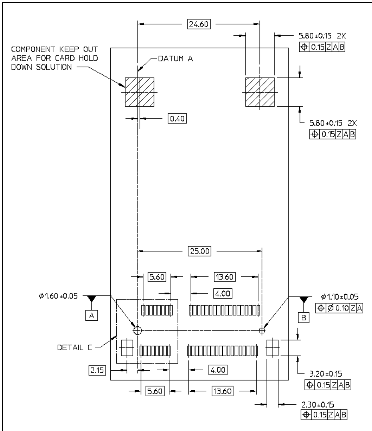
Figure 95 – mSATA card footprint and keepout (informative)
