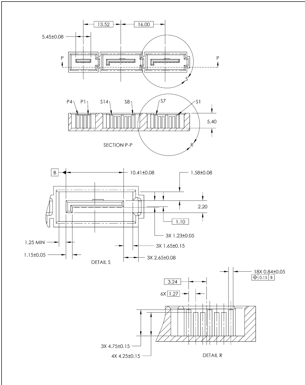
Figure 134 – SATA Express host plug connector drawing
