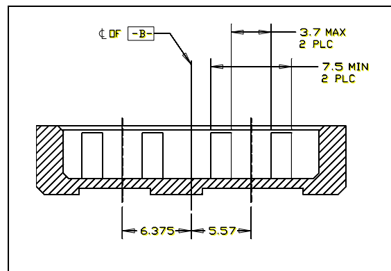
Figure 78 – Slimline device plug connector interface dimensions (section G-G)
