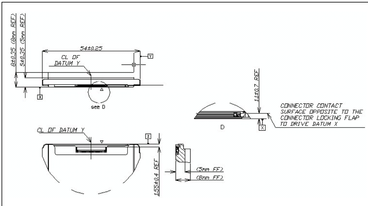
Figure 89 – Internal LIF-SATA connector location for 1.8 inch HDD
