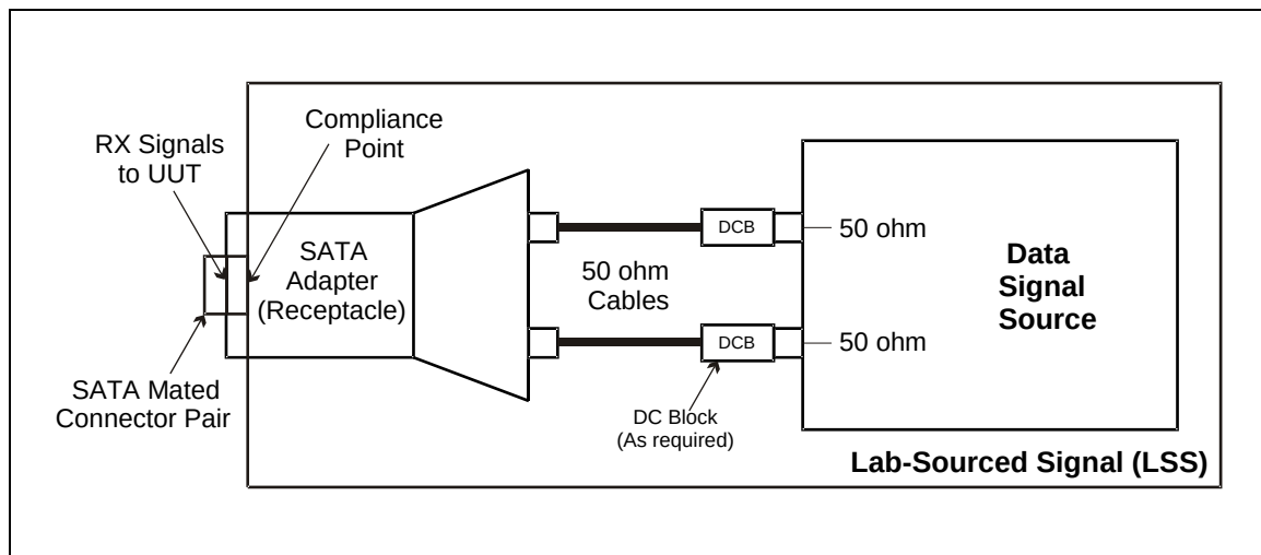
Figure 203 – Lab-Sourced Signal (LSS)
