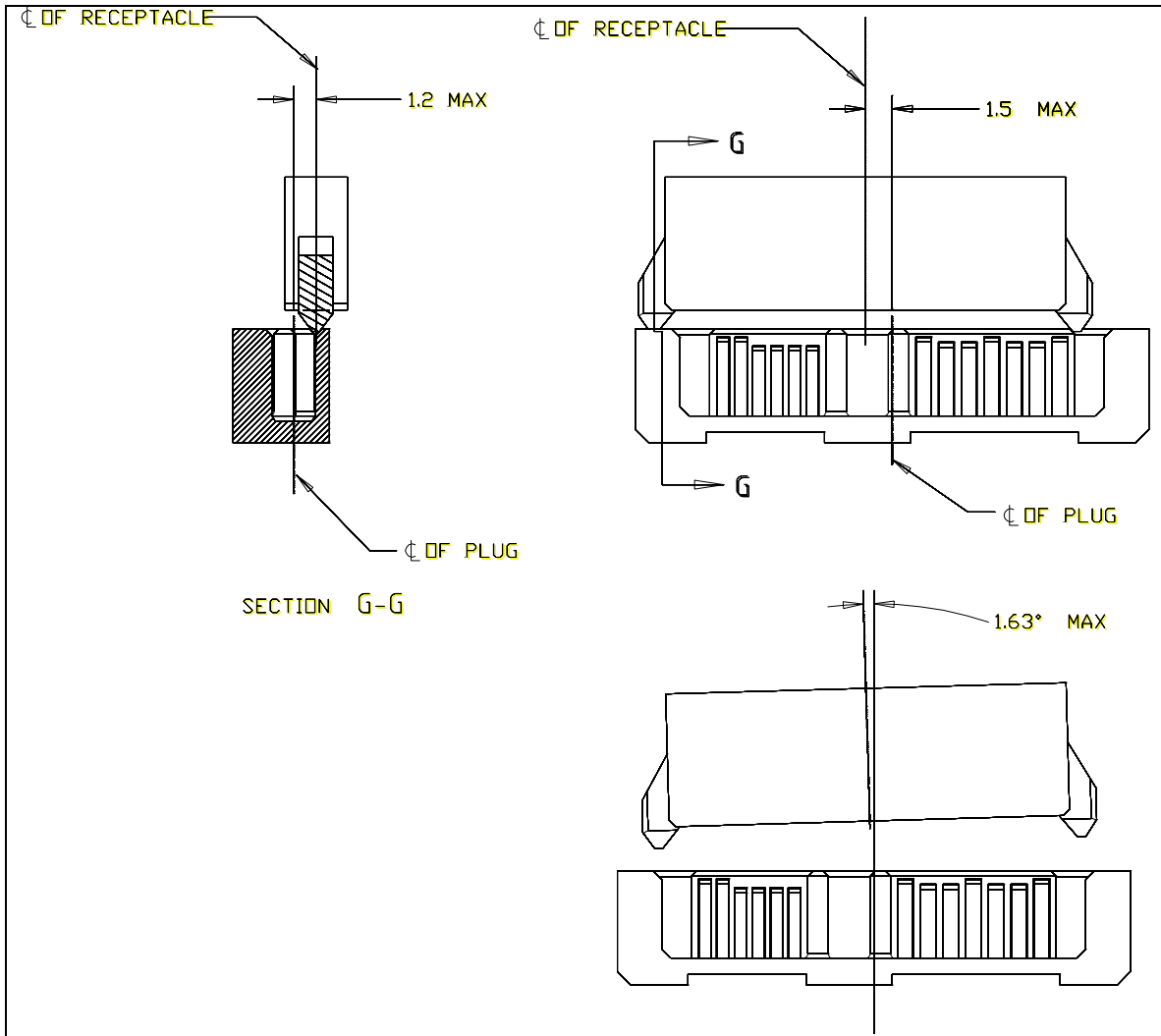
Figure 88 – Slimline connector pair blind-mate misalignment tolerance
