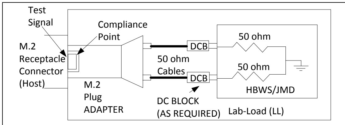
Figure 202 – Lab-Load (LL) for M.2 host
