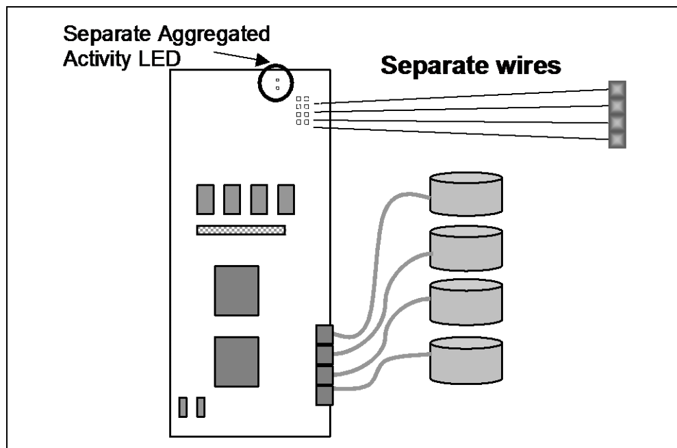
Figure 419 – Device activity LEDs with separate wires
