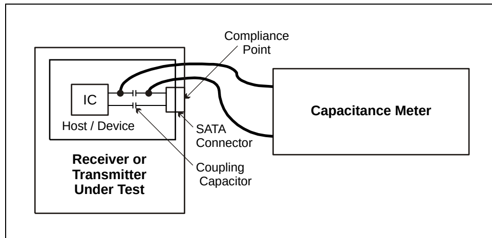
Figure 240 – AC coupled capacitance measurement
