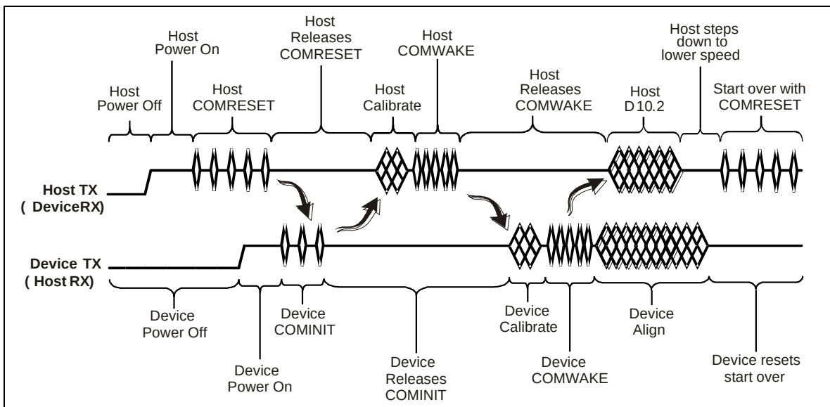
Figure 261 – Speed negotiation using COMRESET (RSN)
