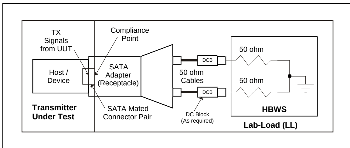
Figure 235 – Intra-pair skew test for a transmitter
