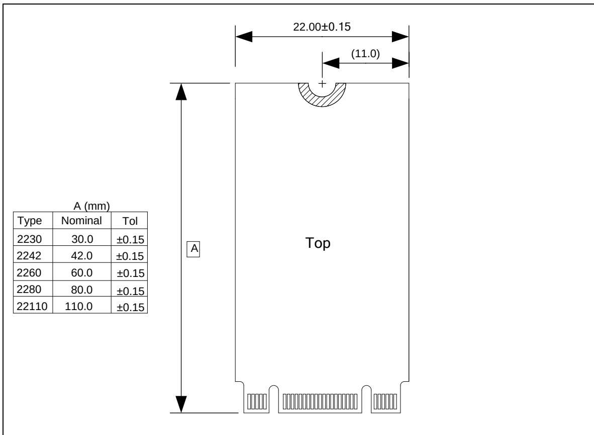
Figure 120 – M.2 board sizes (informative)
