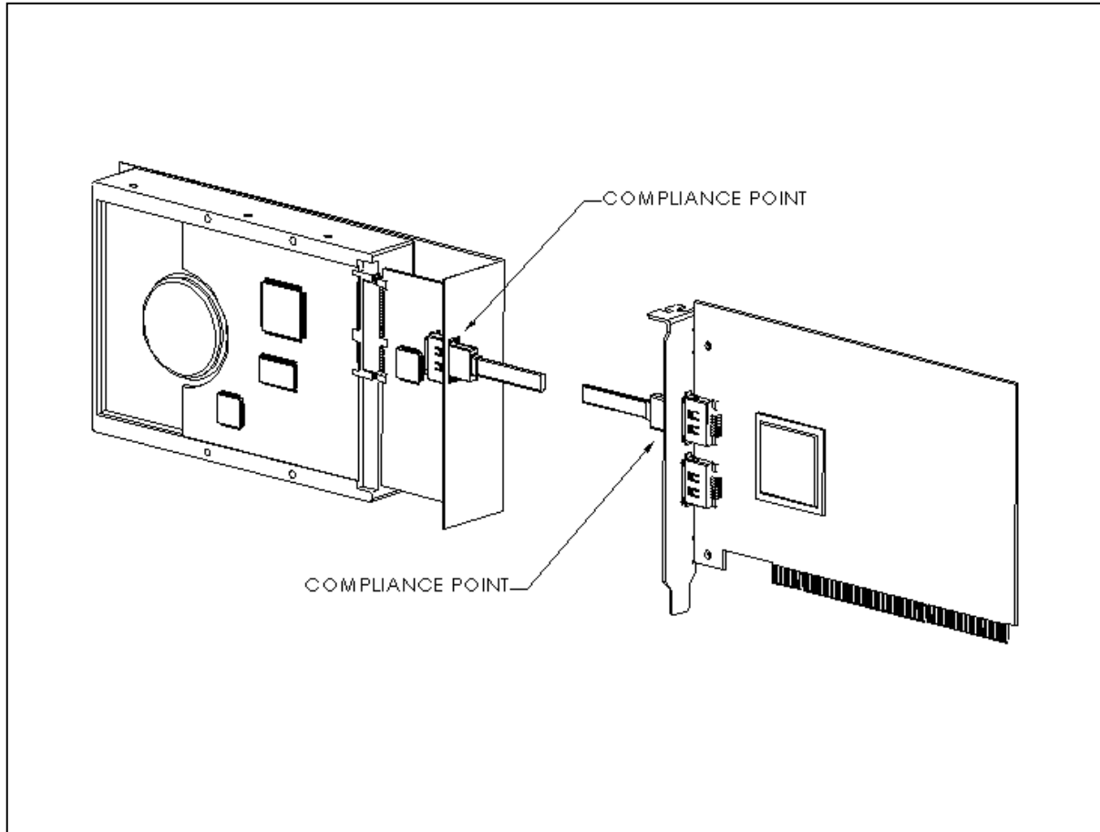
Figure 140 – Usage model for HBA with external cable and single device enclosure
