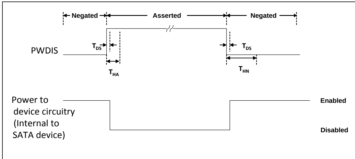
Figure 266 – Power Disable protocol overview
