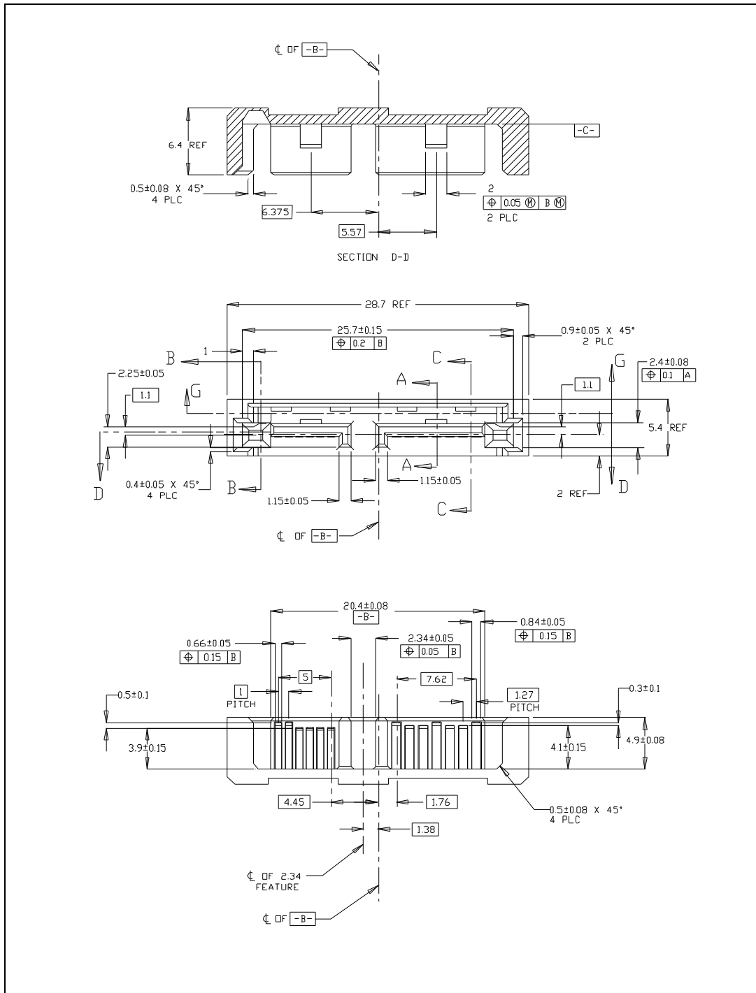
Figure 73 – Slimline device plug connector interface dimensions
