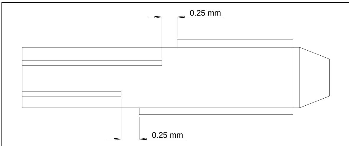
Figure 123 – M.2 pull back (informative)
