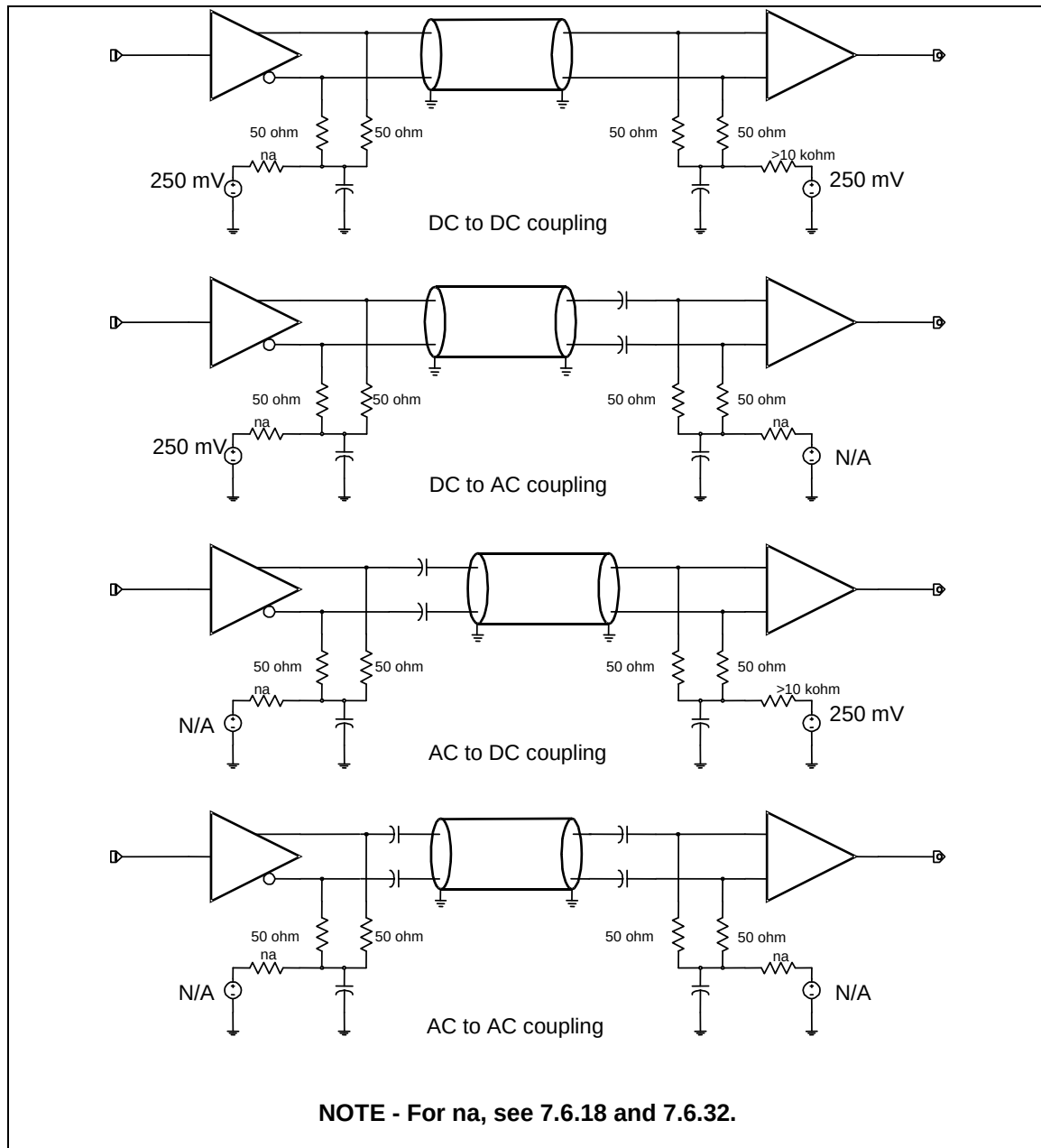
Figure 169 – Common mode biasing examples for Gen1i (informative)
