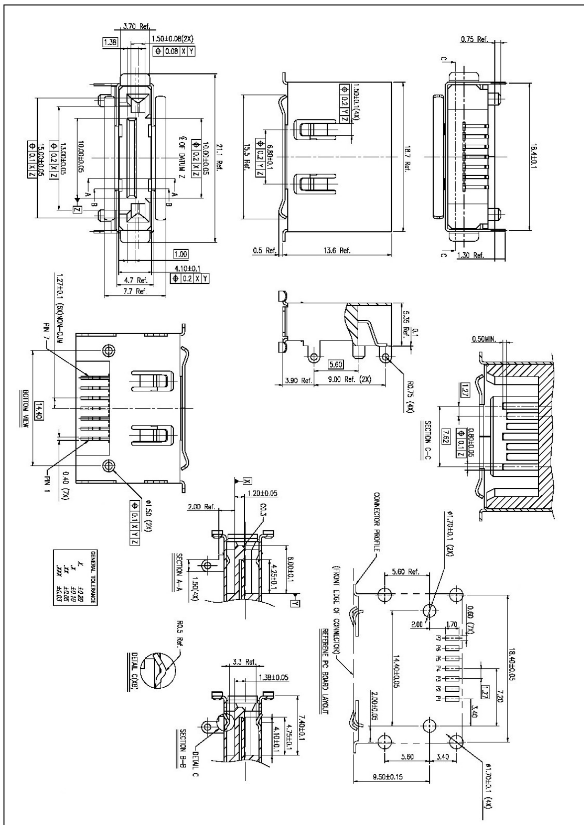
Figure 144 – Mechanical dimensions of External Serial ATA RA SMT plug
