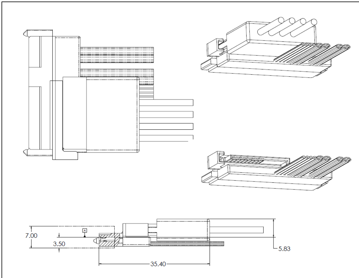
Figure 138 – Example power dangle to be used with the 15 pin SATA power connector
