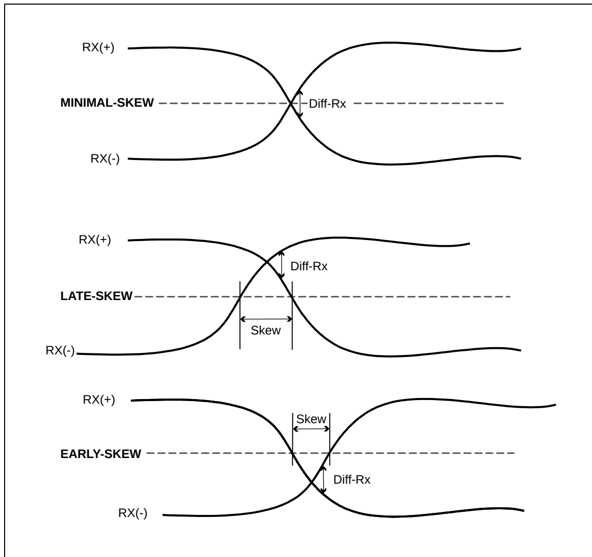
Figure 181 – Rx intra-pair skew
