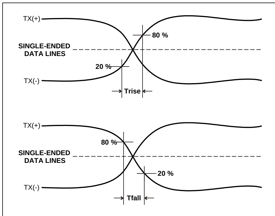
Figure 214 – Single ended rise and fall time
