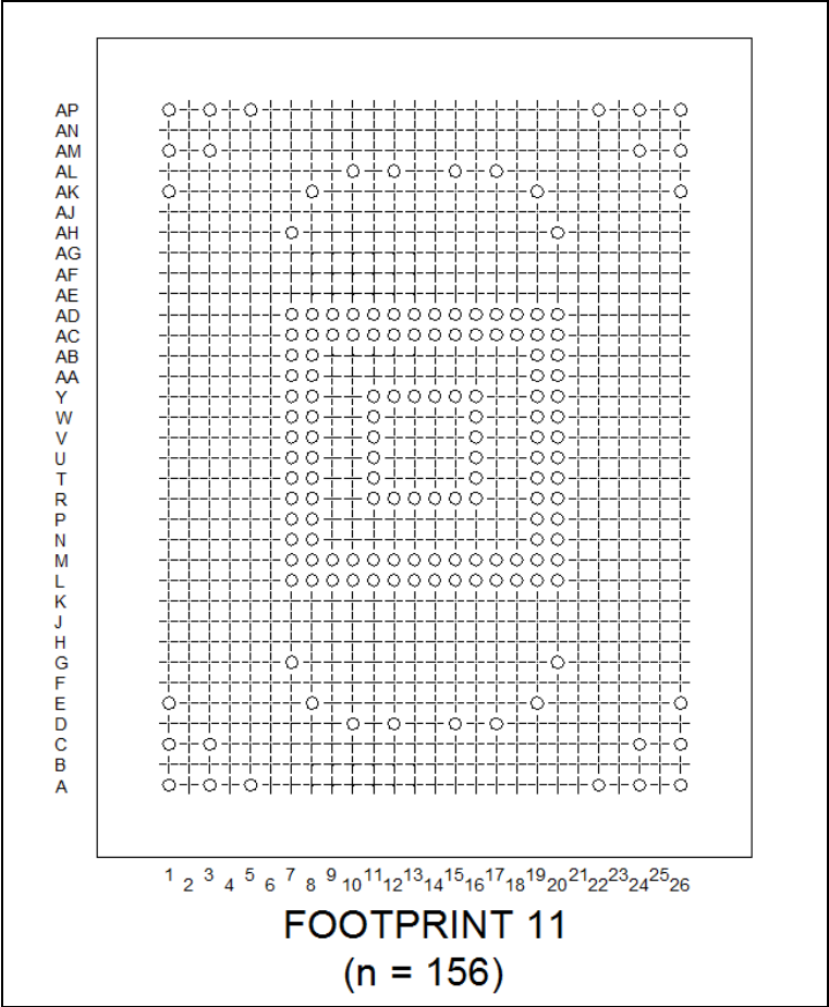
Figure 108 – Footprint 11, SATA MicroSSD variant AM and CA, 156 balls (informative)
