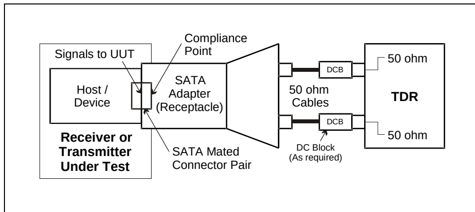
Figure 248 – TDR impedance test
