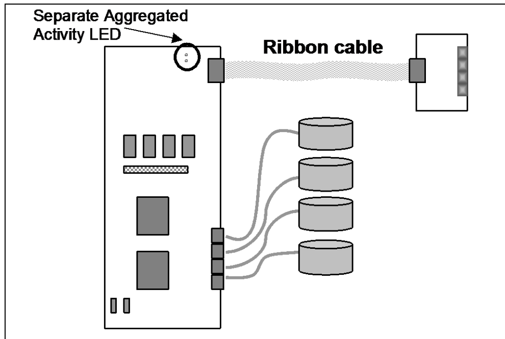
Figure 420 – Device activity LEDs with ribbon cable
