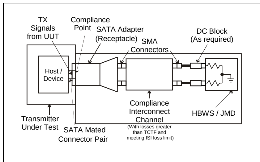
Figure 216 – Transmit amplitude test with CIC
