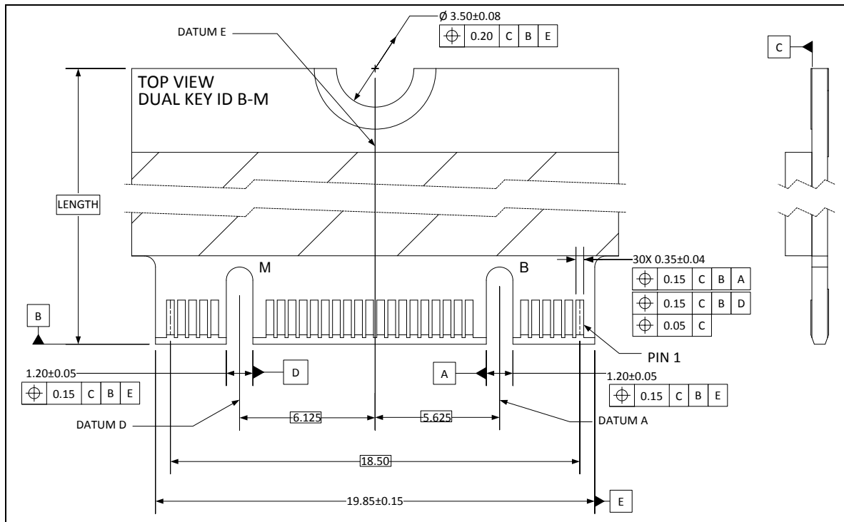
Figure 114 – M.2 keys (informative)
