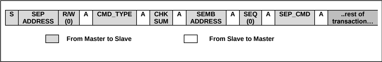
Figure 407 – I 2 C frame for conveying an enclosure services command
