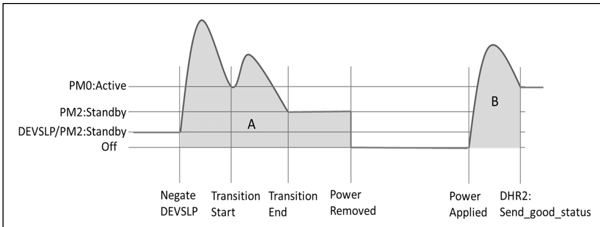
Figure 397 – Transitional Energy, DevSleep/PM2: Standby to PM0: Active, and Off to DHR2:Send_good_status
