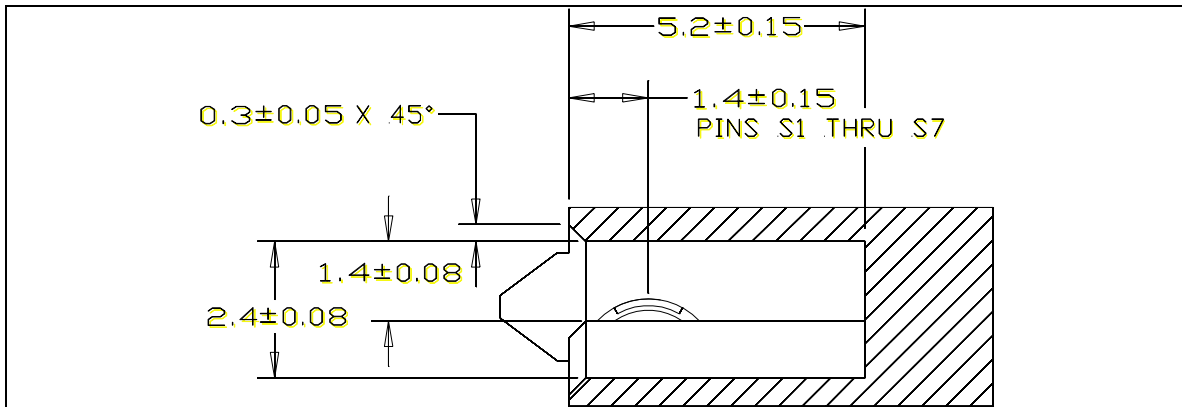
Figure 86 – Slimline host receptacle connector interface dimensions section X-X
