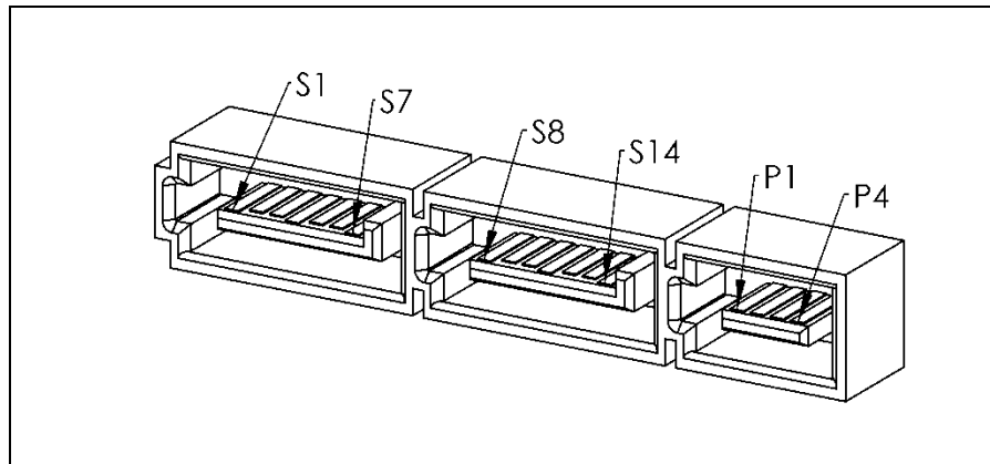
Figure 132 – SATA Express host plug connector pinout (isometric view)
