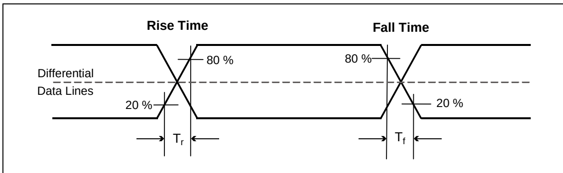
Figure 176 – Signal rise and fall times
