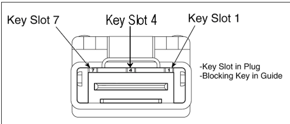
Figure 152 – Mini SATA External Multilane system, key features
