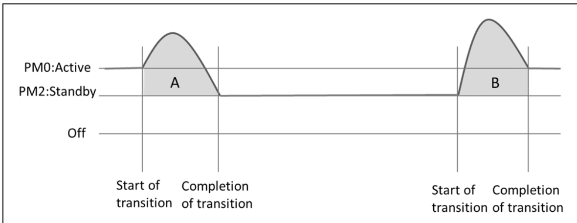
Figure 396 – Transitional Energy, PM0: Active to PM2: Standby, and PM2: Standby to PM0: Active
