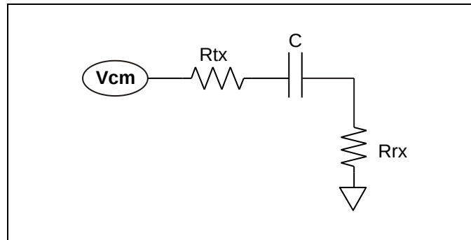
Figure 186 – Example circuit for common mode transients
