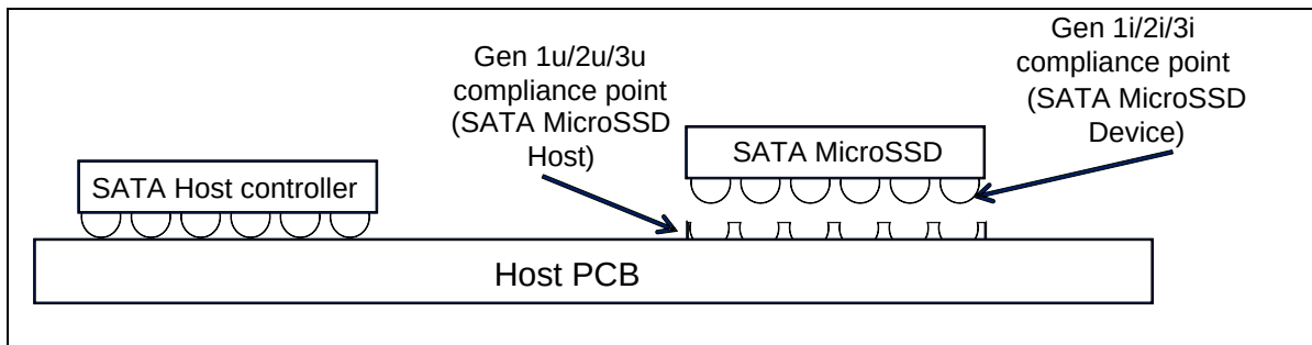
Figure 14 – Embedded SATA MicroSSD application
