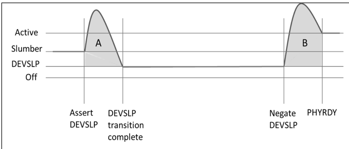
Figure 394 – Transitional Energy, Slumber to DevSleep, and DevSleep to PHYRDY
