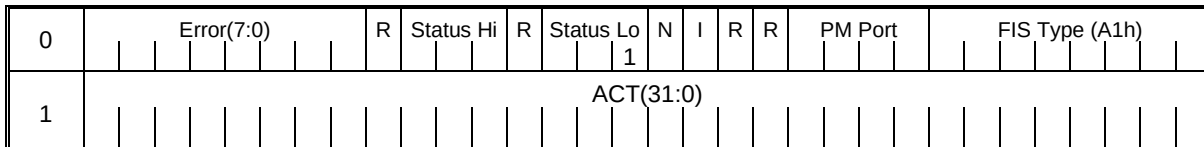
Figure 379 – Set Device Bits FIS with error notification and command completions
