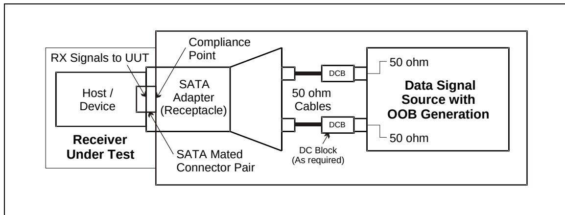
Figure 242 – Squelch detector threshold test
