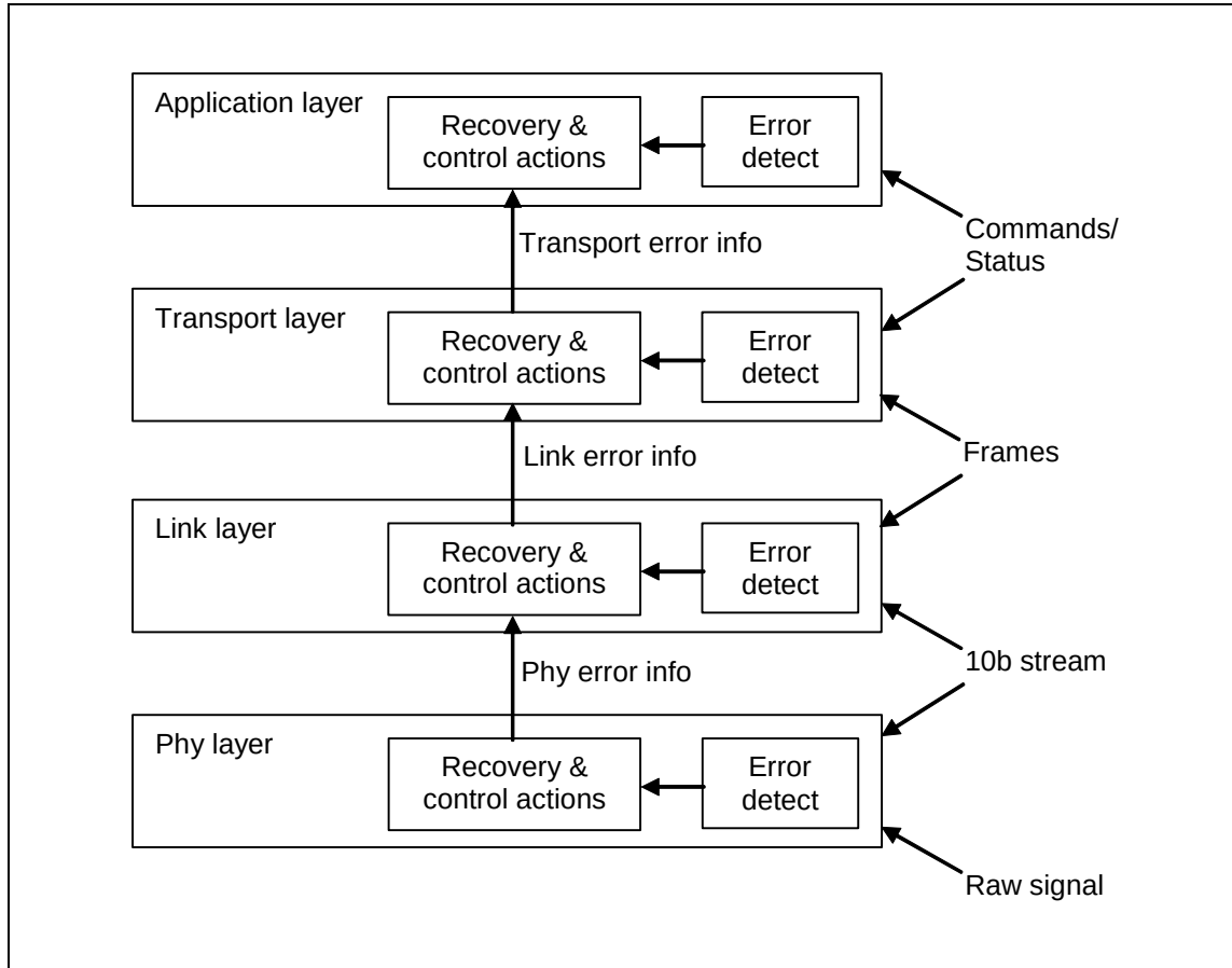
Figure 432 – Error handling architecture
