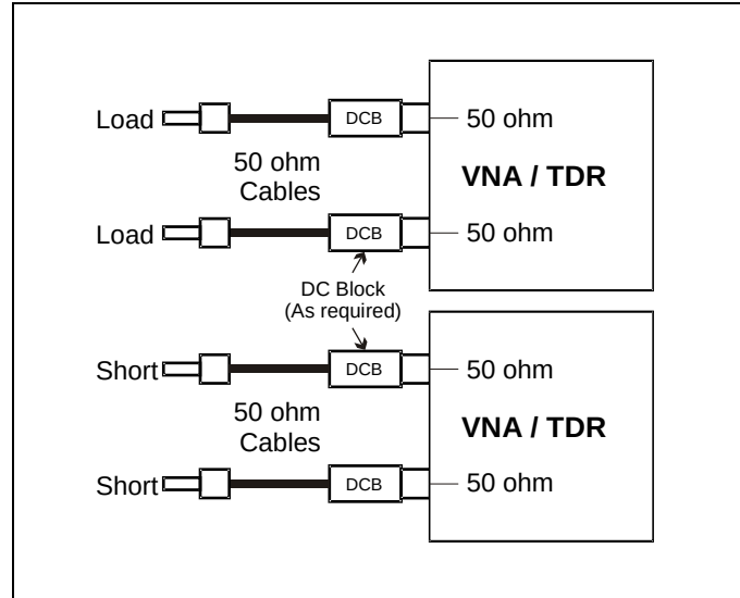
Figure 233 – Return loss test-calibration
