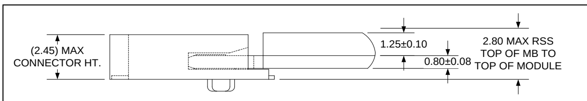
Figure 116 – M.2 single sided assembly – S2 profile (informative)
