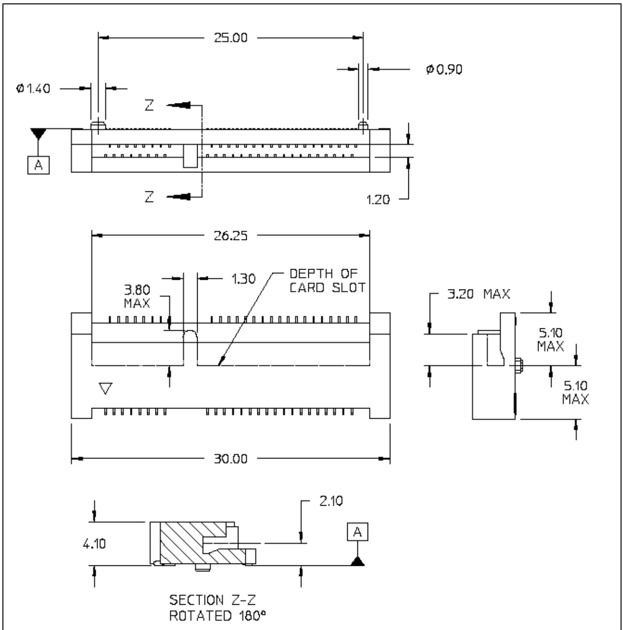
Figure 94 – mSATA card connector (informative)
