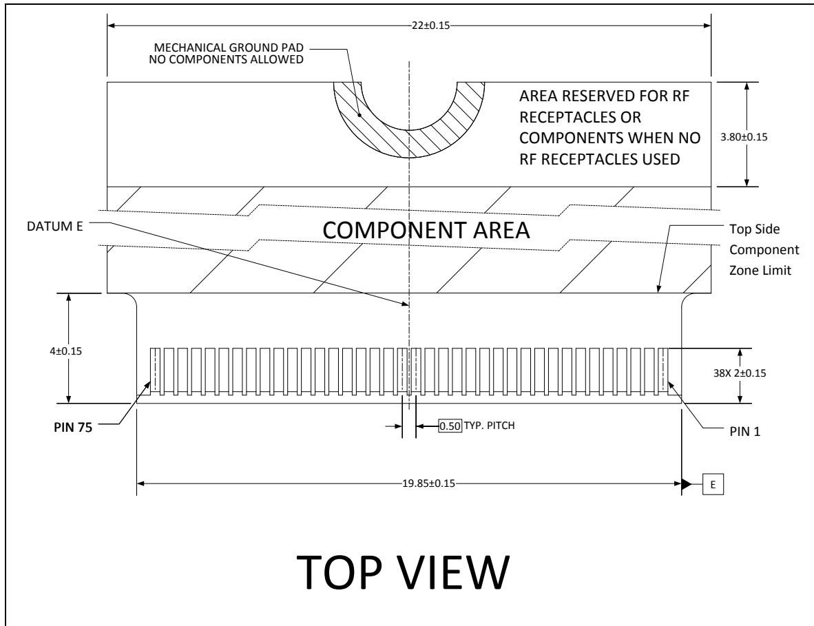
Figure 110 – M.2 board connector top details (informative)
