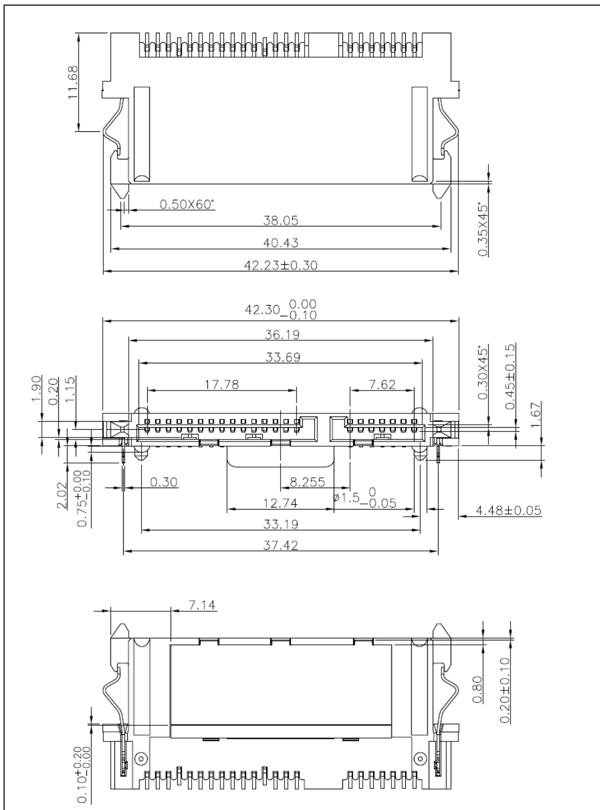
Figure 103 – SATA USM horizontal receptacle (see INF-8280)
