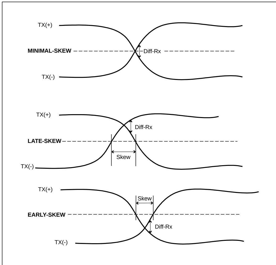
Figure 177 – Tx intra-pair skew
