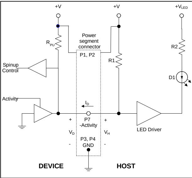
Figure 158 – Example Device Activity Signal (DAS) electrical block diagram
