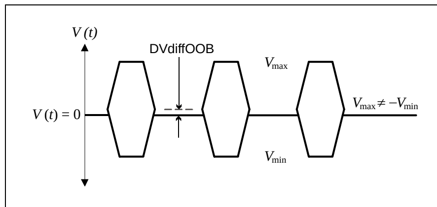
Figure 178 – OOB differential delta (at compliance point with AC coupling)
