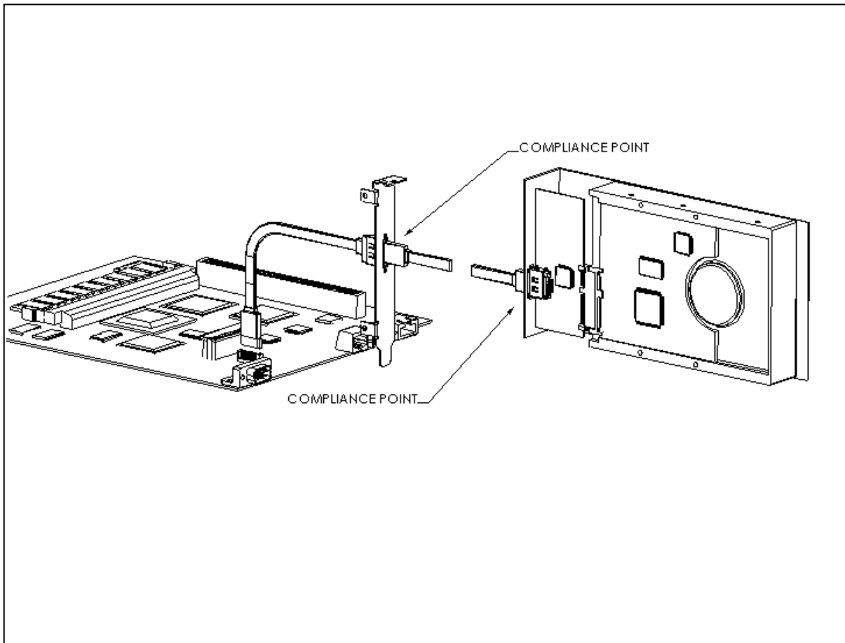
Figure 141 – Usage model for on-board Serial ATA connector with extension cable to external cable to disk
