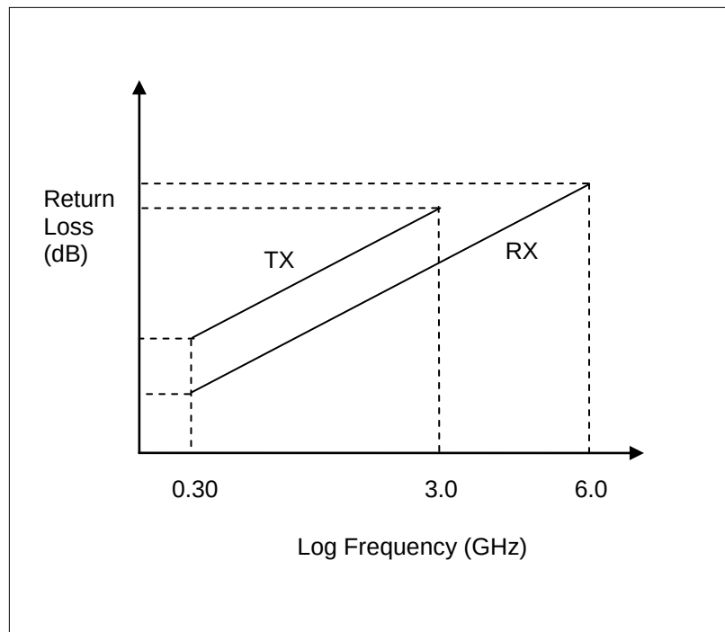
Figure 175 – Differential return loss limits, Gen3i, Tx and Rx
