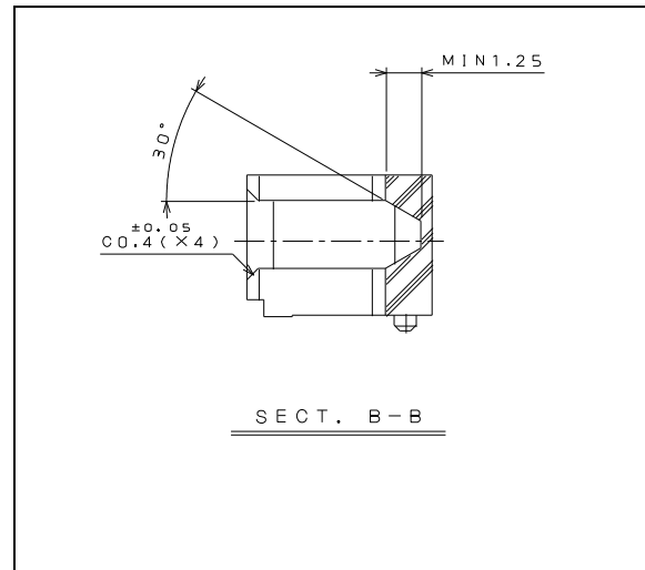
Figure 70 – 7.0 mm Slimline device plug connector interface dimensions section B-B
