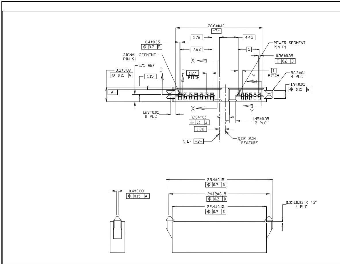
Figure 84 – Slimline host receptacle connector interface dimensions
