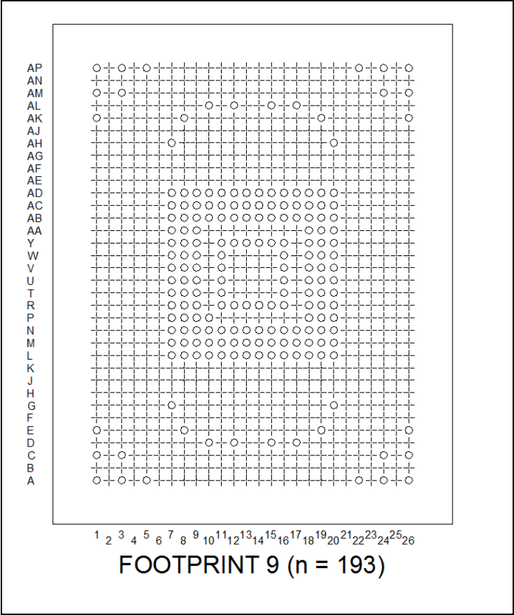
Figure 106 – Footprint 9, SATA MicroSSD variant AK and CB, 193 balls (informative)
