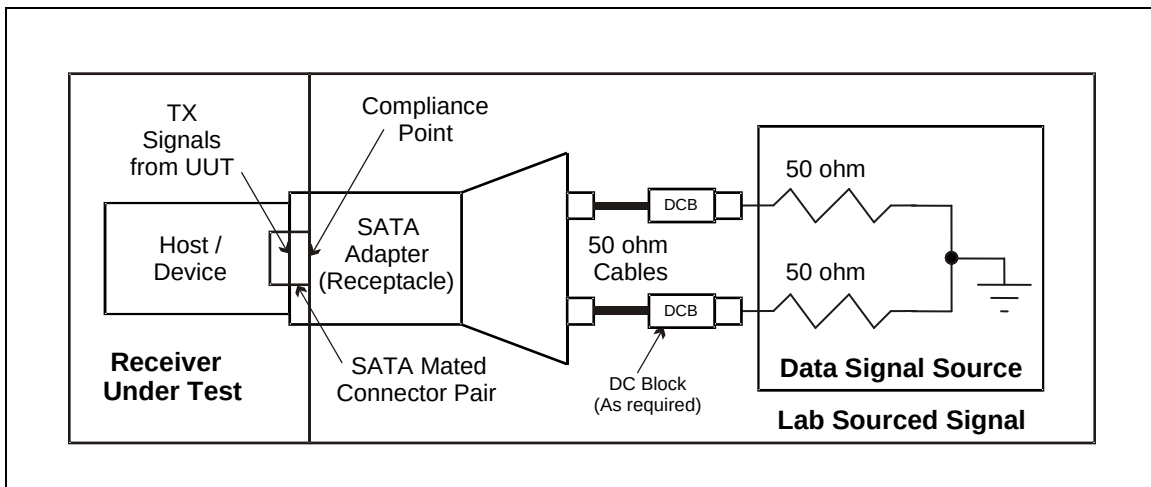
Figure 219 – Receiver amplitude test
