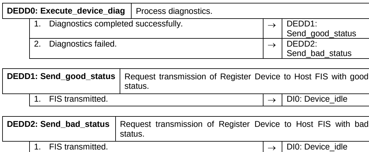
Figure 319 – Device command layer diagnostic state machine
