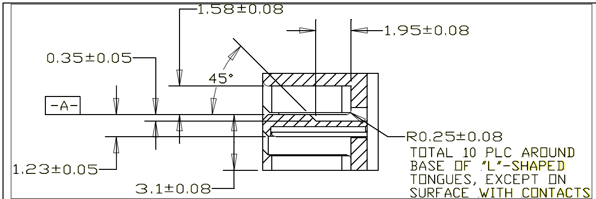
Figure 74 – Slimline device plug connector interface dimensions (section A-A)
