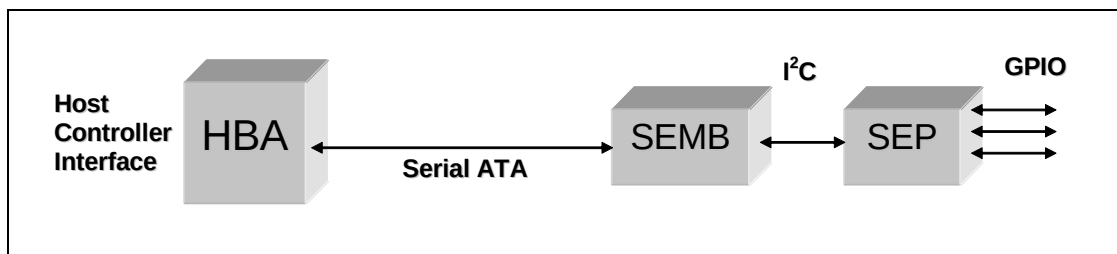
Figure 402 – Simplified view of generic topology
