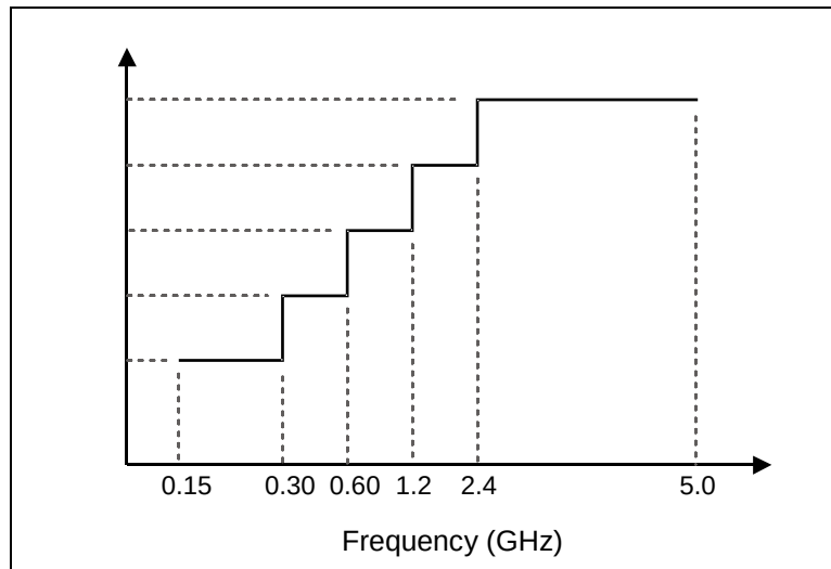
Figure 173 – Common mode return loss limits
