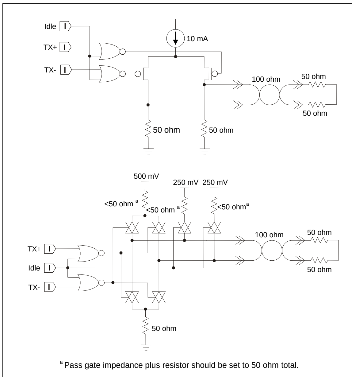
Figure 253 – Transmitter examples
