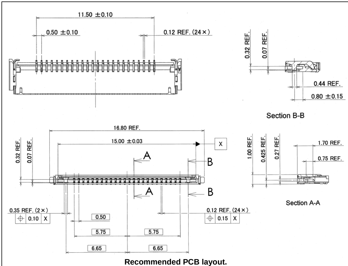
Figure 92 – Device internal LIF-SATA surface mounting type connector
