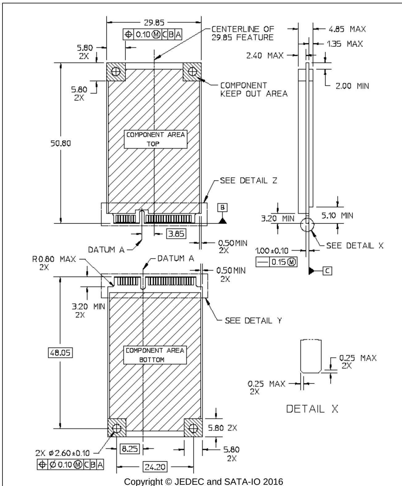
Figure 97 – Device mSATA card type internal connector (informative)
