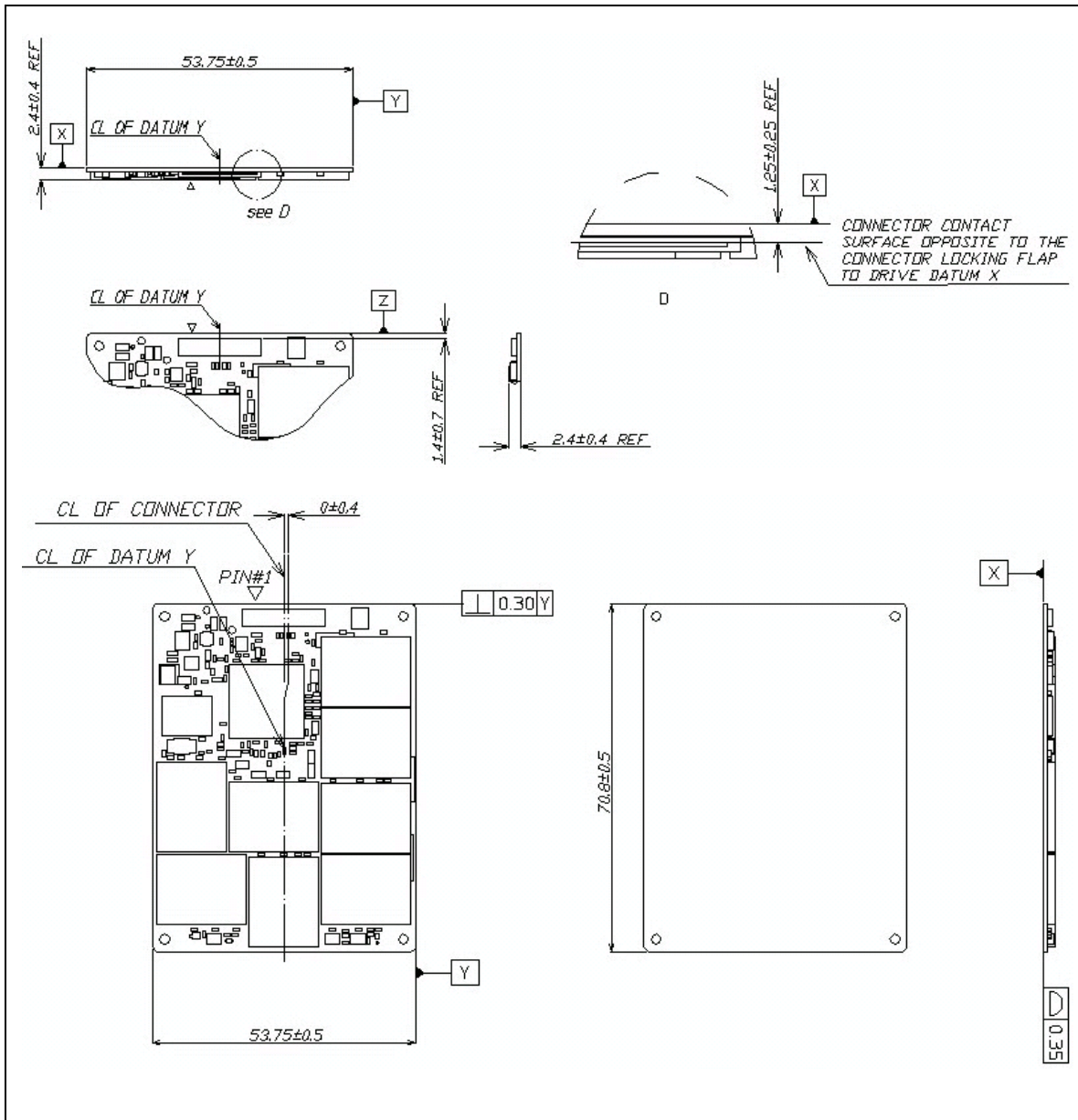
Figure 90 – Internal LIF-SATA connector location for 1.8 inch SSD bulk of single-sided mount type
