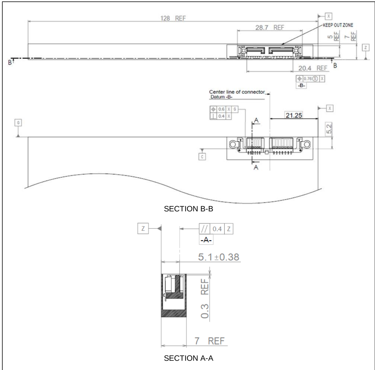
Figure 63 – 7.0 mm Slimline drive connector locations (informative)
