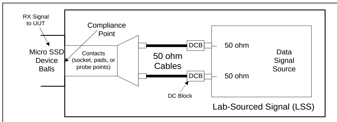
Figure 207 – Lab-Sourced Signal (LSS) for SATA MicroSSD device
