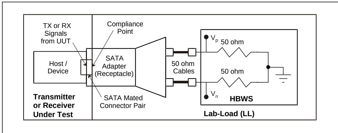
Figure 249 – Sequencing transient Voltage lab-load (LL)
