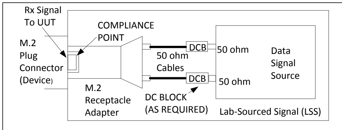
Figure 209 – Lab-Sourced Signal (LSS) for M.2 device
