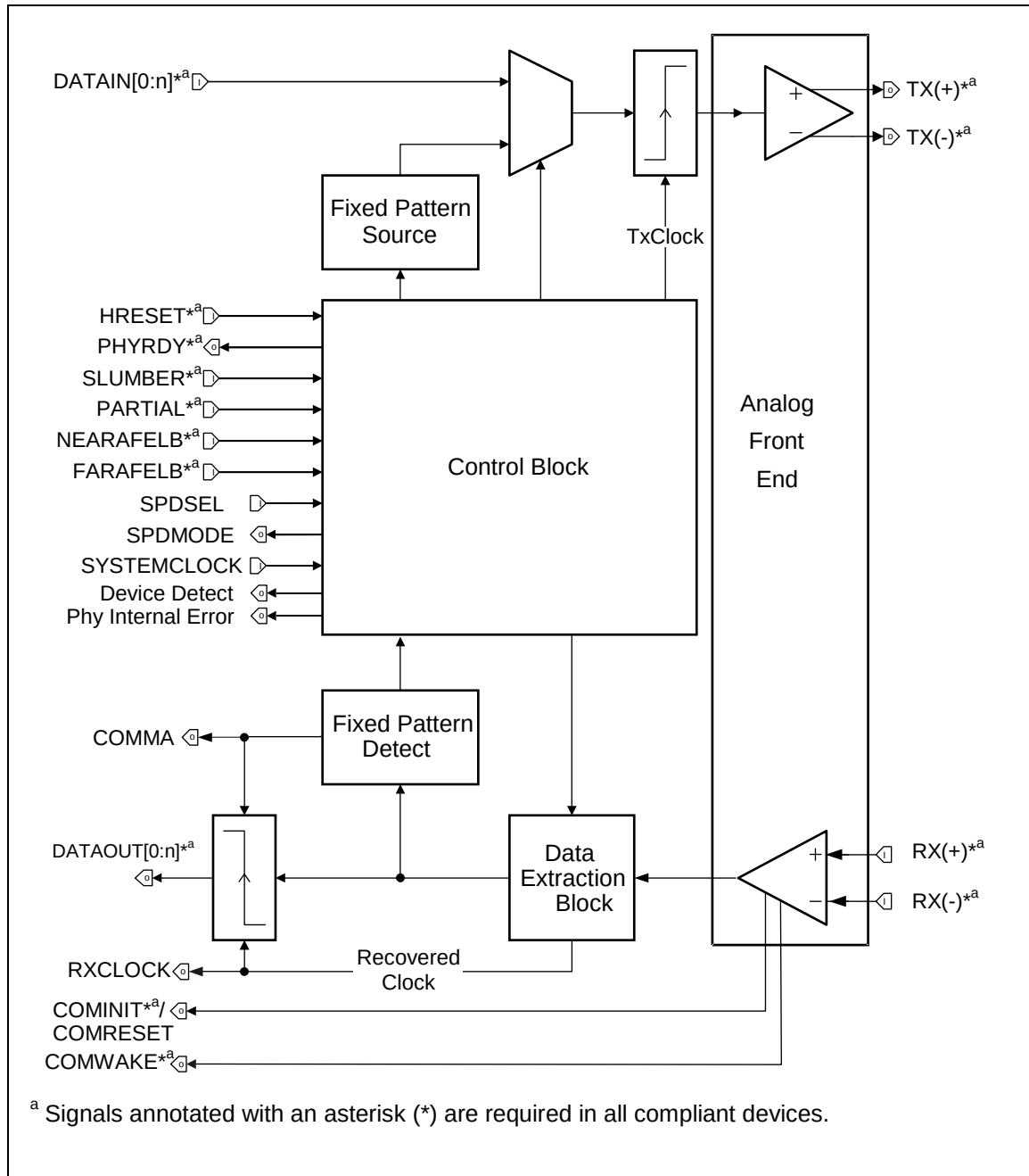
Figure 162 – Physical plant overall block diagram (informative)
