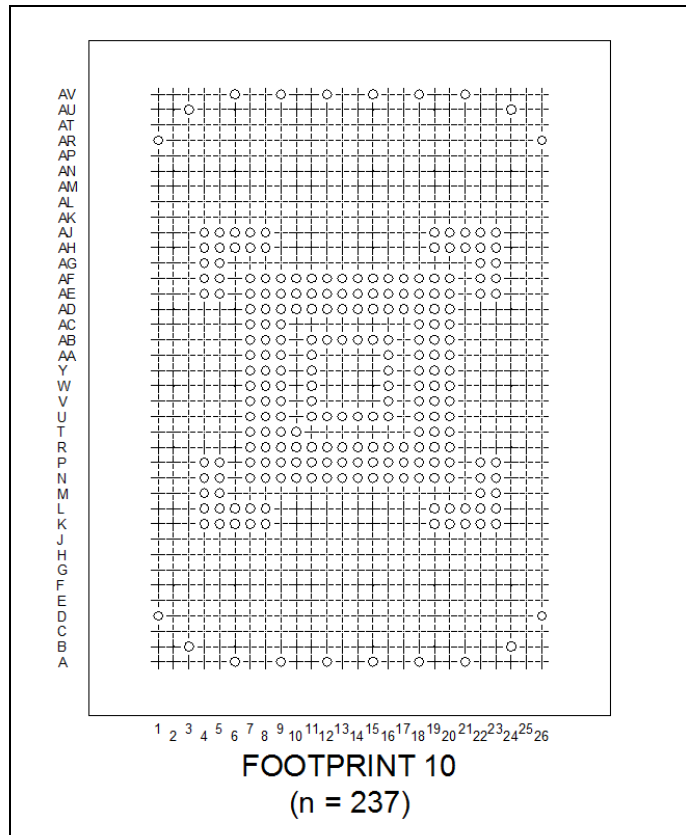
Figure 107 – Footprint 10, SATA MicroSSD variant AL, 237 balls (informative)
