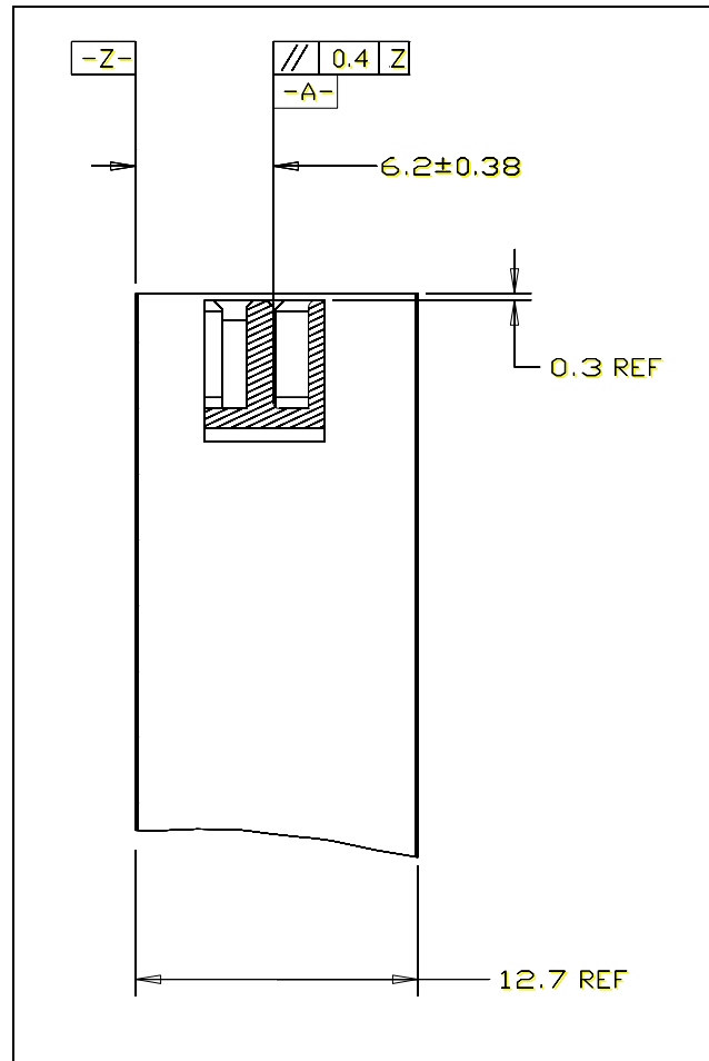
Figure 67 – 12.7 mm Slimline drive connector location (section A-A) (informative)
