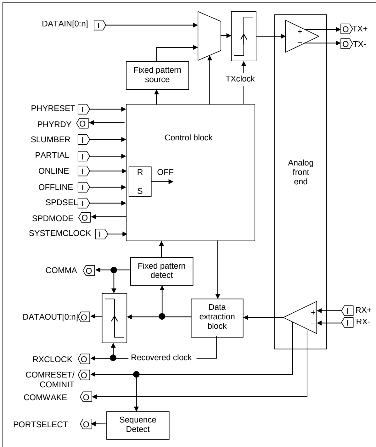
Figure 450 – Phy block diagram
