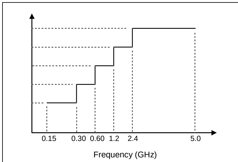
Figure 174 – Impedance balance limits
