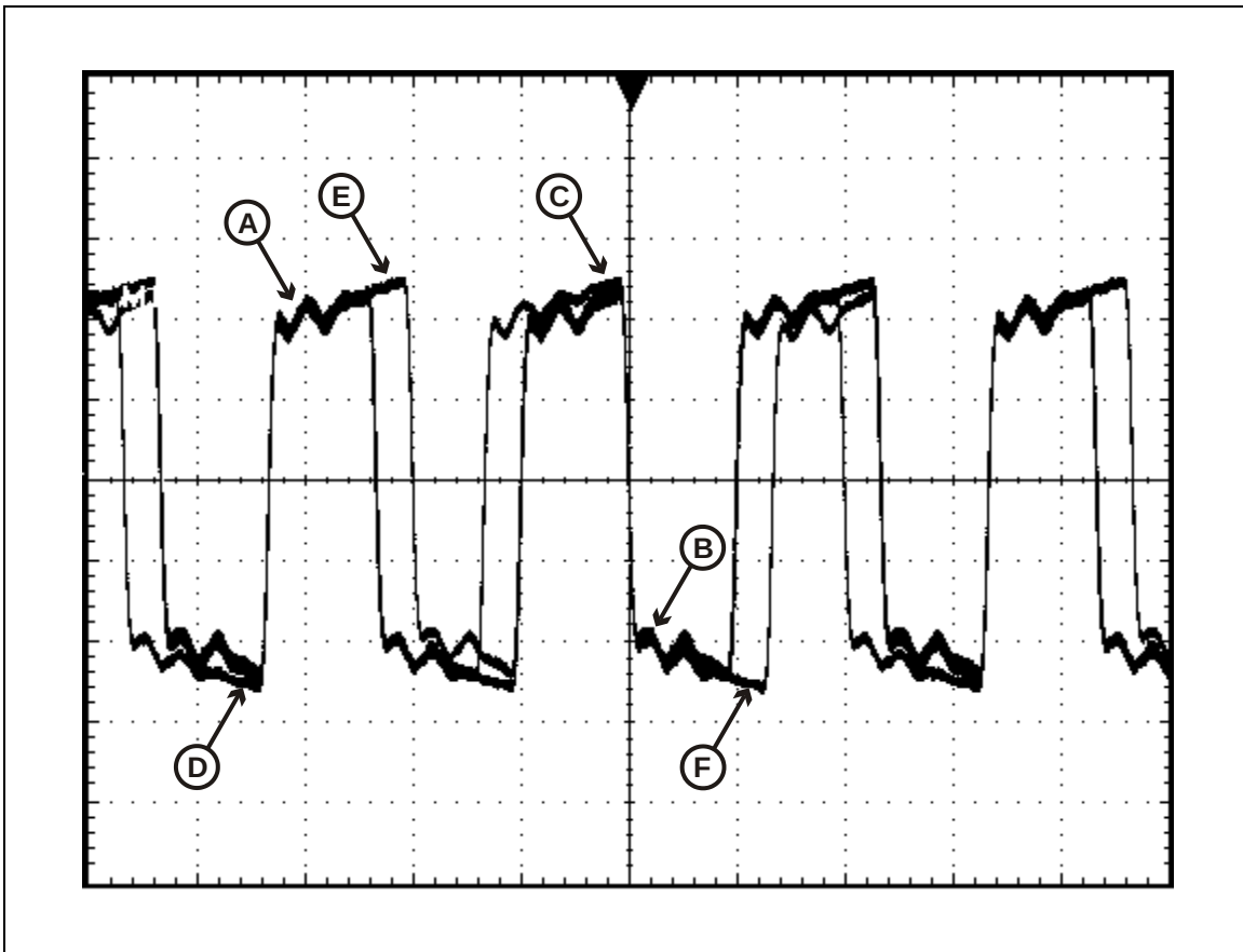
Figure 213 – LFTP Pattern on High BW Scope (HBWS)
