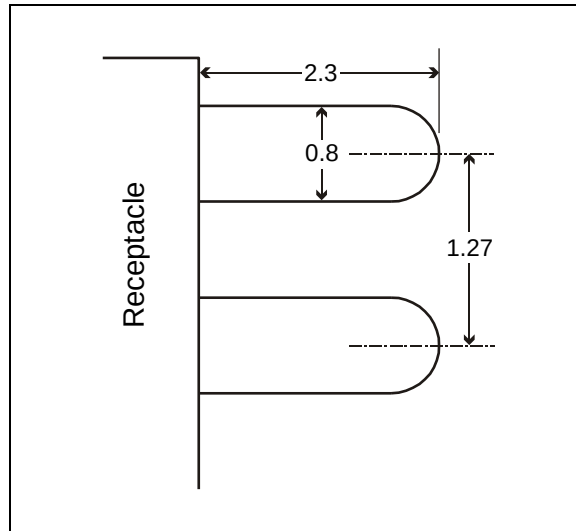
Figure 188 – Mated connector pair, pin tail detail
