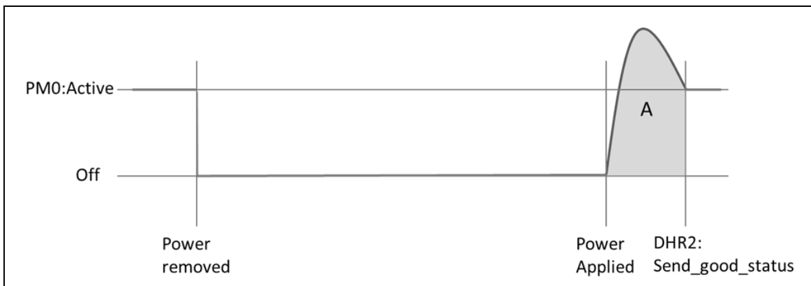
Figure 395 – Transitional Energy, PM0: Active to Off, and Off to PM0: Active
