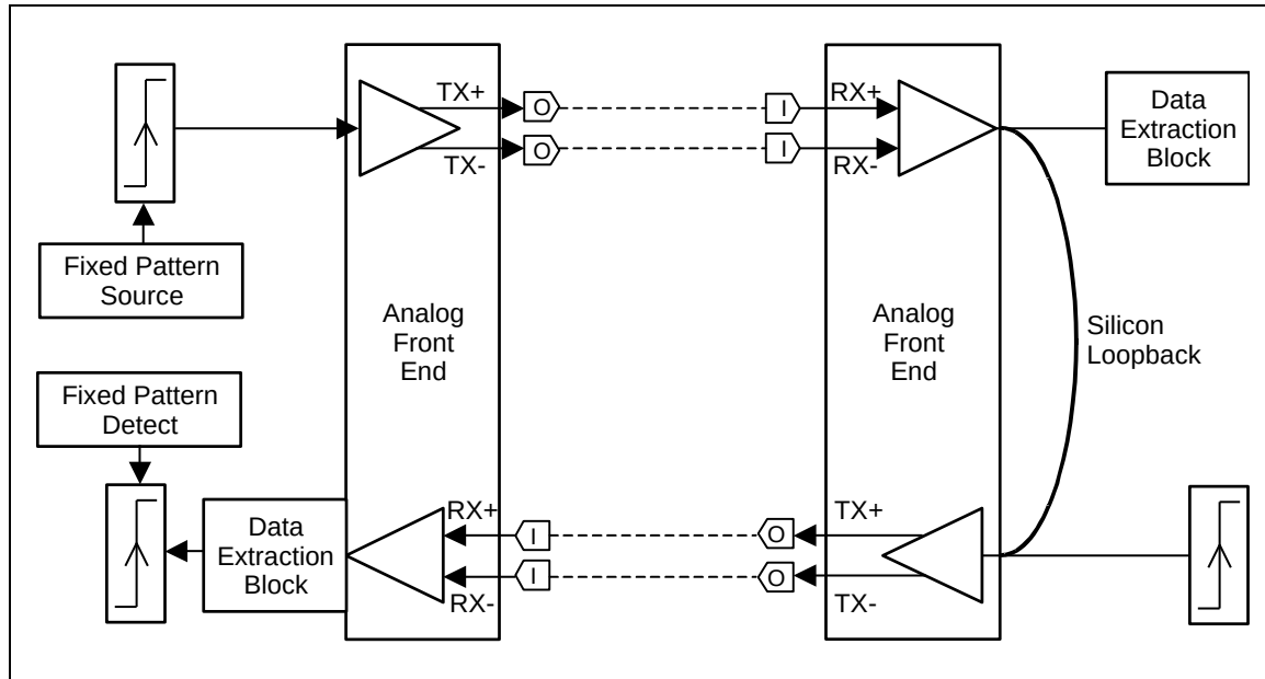
Figure 183 – Far-End Analog Loopback
