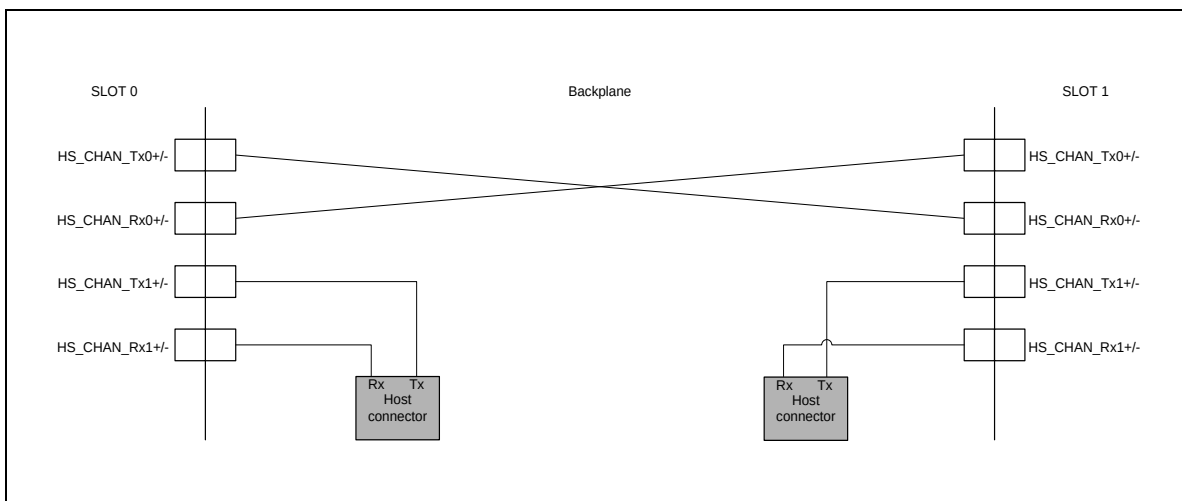
Figure D.5 – High-speed channels – configuration 1
