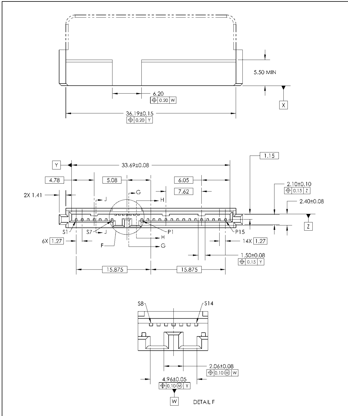
Figure 129 – SATA Express device cable receptacle connector drawing
