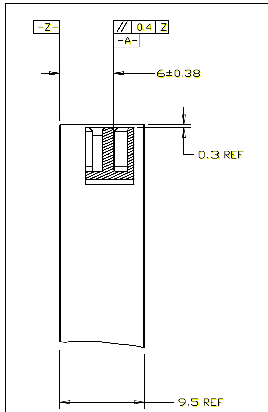
Figure 66 – 9.5 mm Slimline drive connector location (section A-A) (informative)
