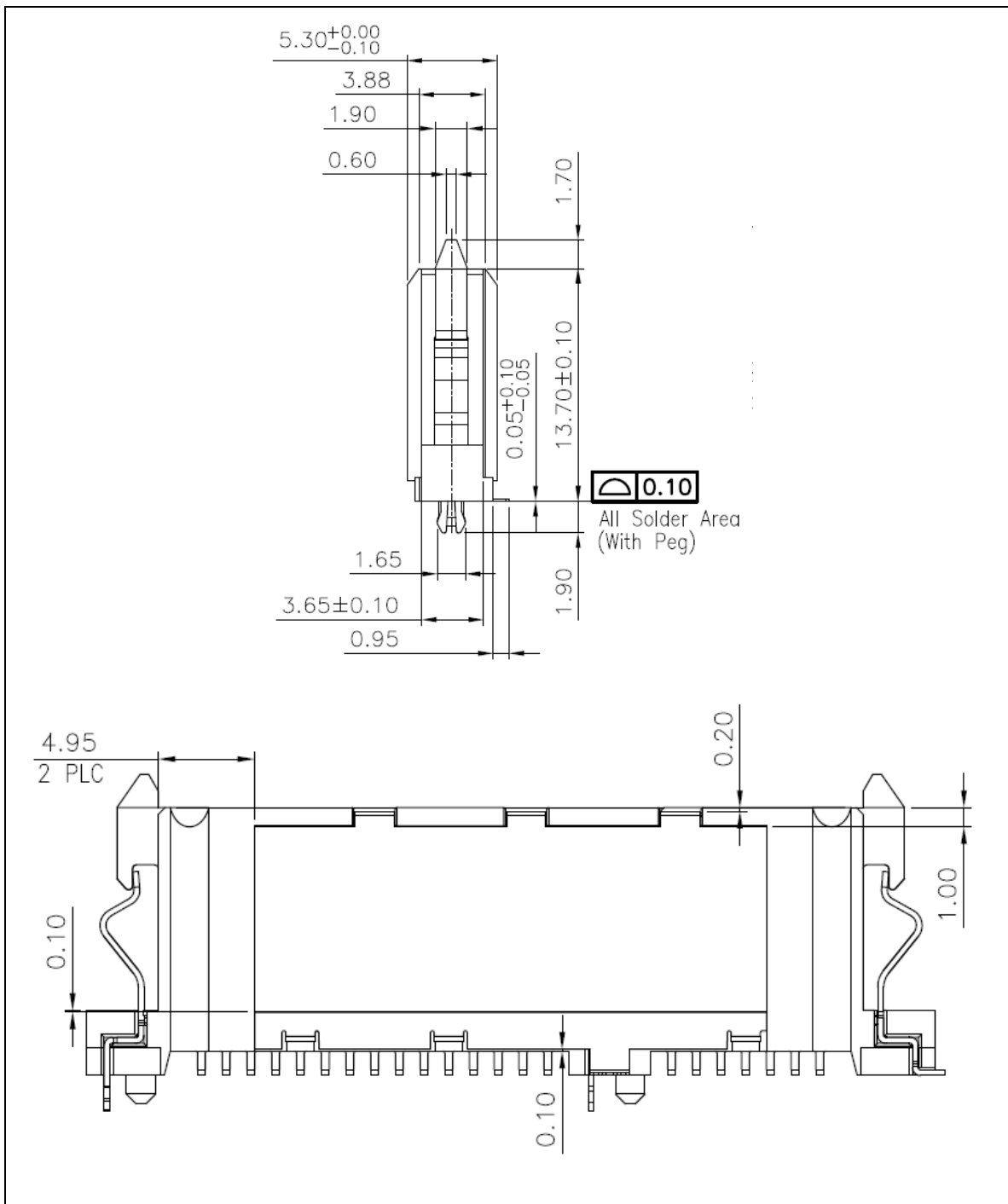
Figure 102 – SATA USM vertical receptacle continued (see INF-8280)
