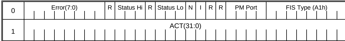
Figure 373 – Set Device Bits FIS with error notification and command completions
