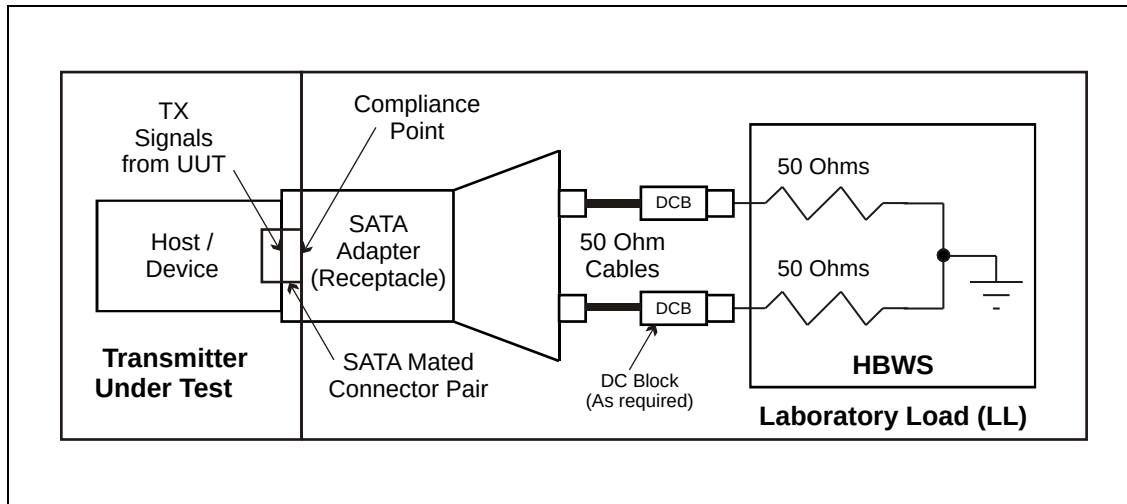
Figure 211 – Differential Voltage amplitude measurement
