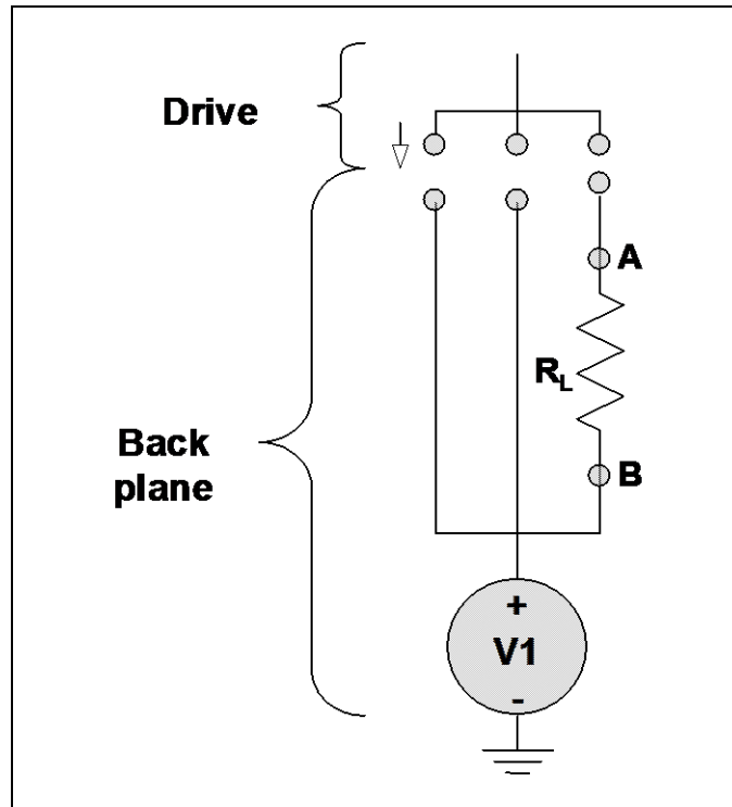
Figure 160 – Typical precharge configuration
