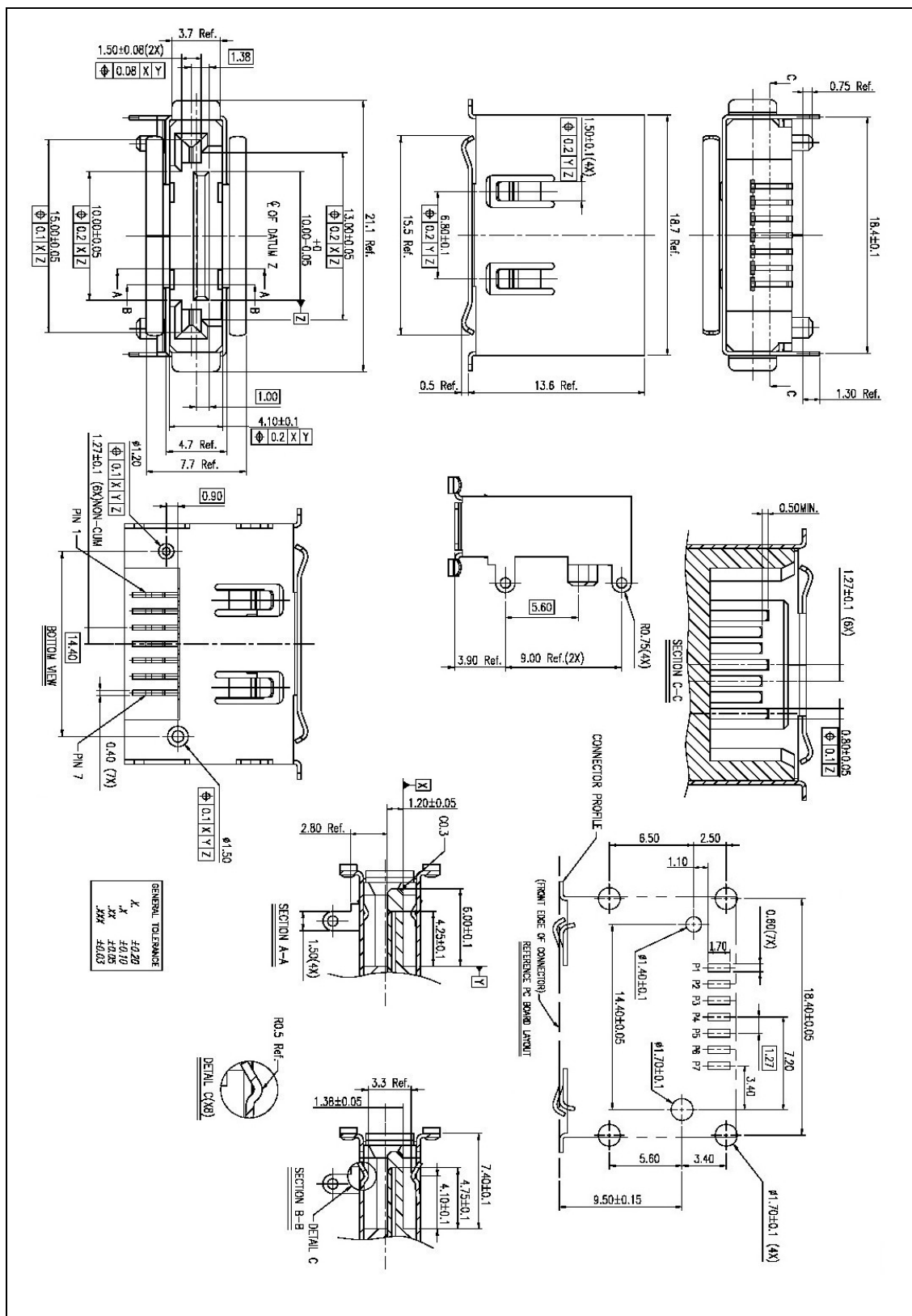
Figure 145 – Mechanical dimensions of External SATA RA SMT plug – reversed pin out
