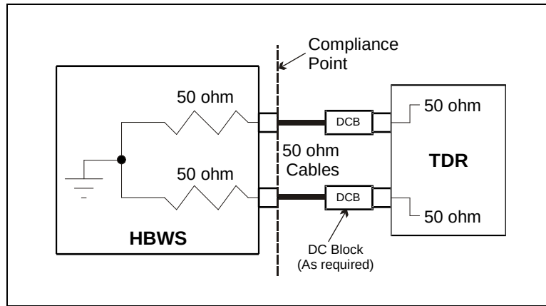
Figure 243 – TDR differential impedance test – setting risetime
