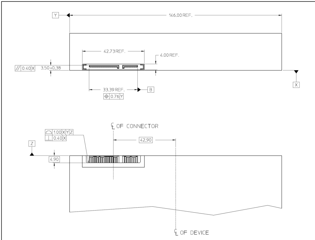
Figure 24 – Non-optical alternate device plug connector location on 5.25 inch form factor
