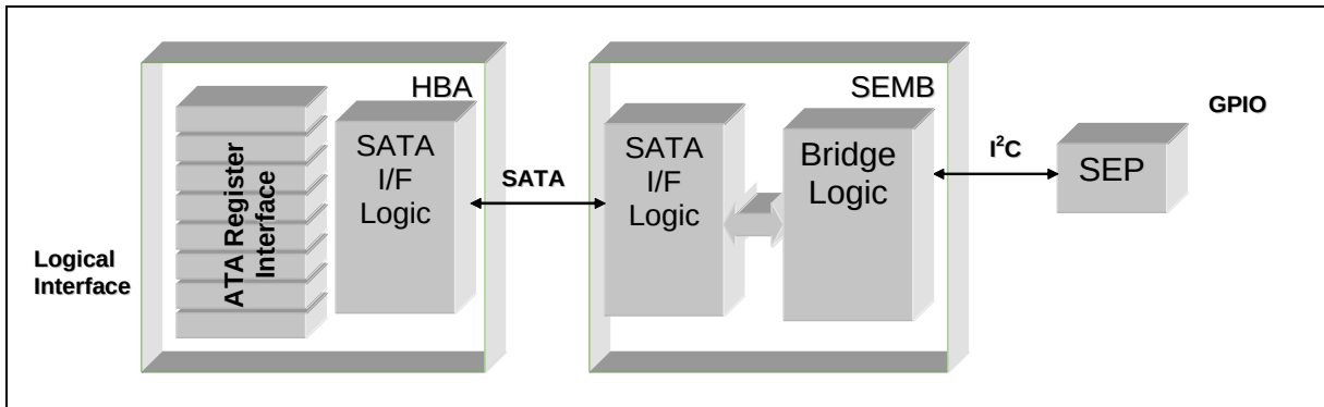
Figure 403 – Enclosure services definition configuration
