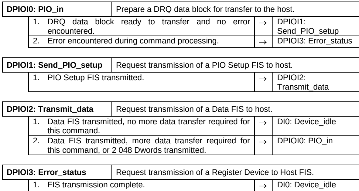
Figure 327 – Device command layer PIO data-in state machine
