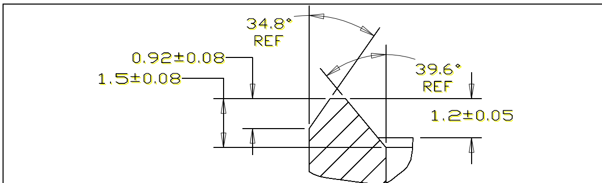
Figure 85 – Slimline host receptacle connector interface dimensions section C-C
