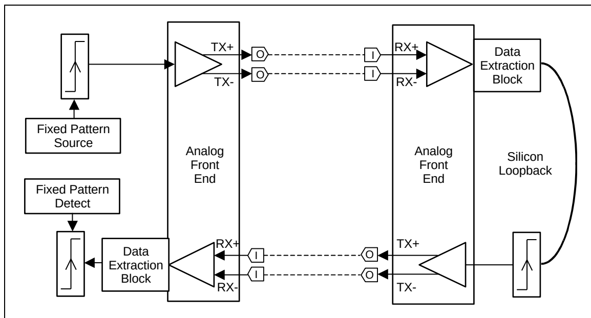
Figure 182 – Far-End Retimed Loopback
