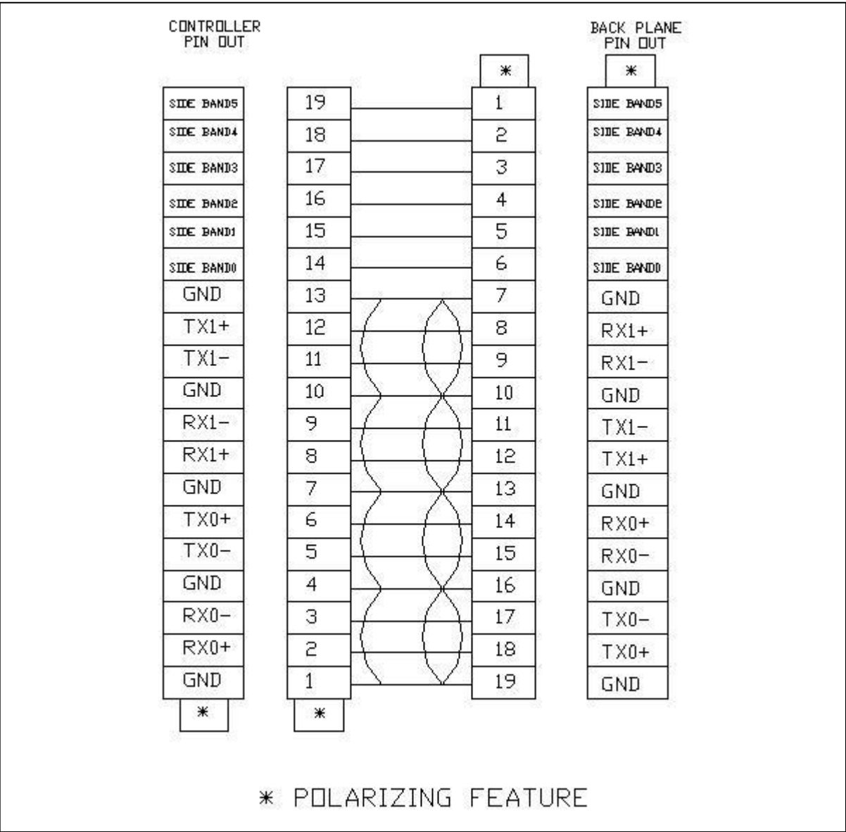
Figure 51 – 2 lane fanout pin assignments
