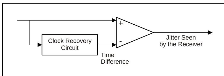
Figure 223 – Jitter at receiver
