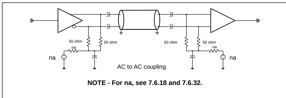
Figure 170 – Common mode biasing for Gen1m, Gen1u, Gen2i, Gen2m, Gen2u, Gen3i, and Gen3u
