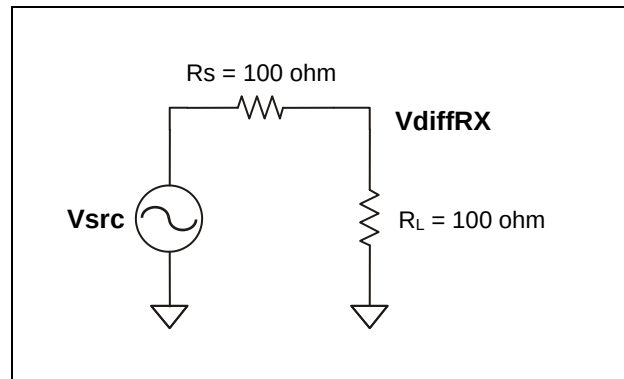
Figure 180 – Rx differential input Voltage conditions
