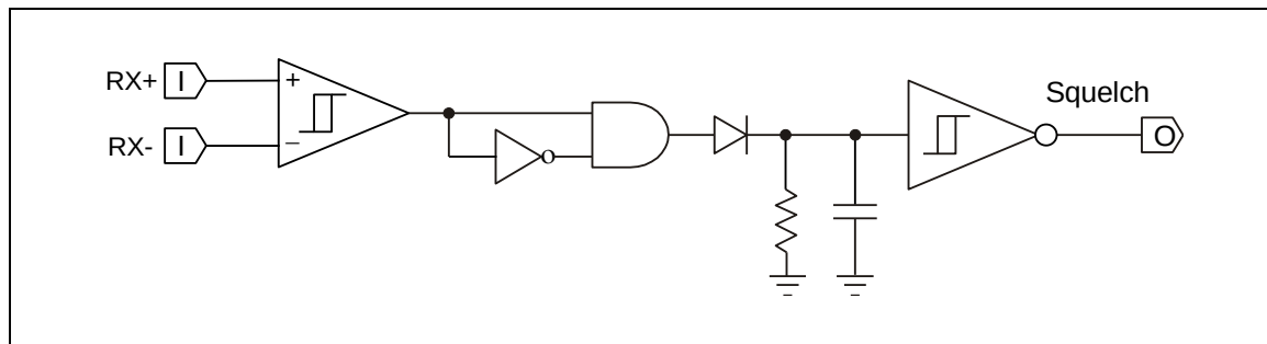
Figure 257 – Squelch detector
