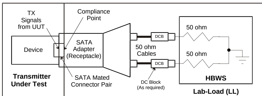
Figure 250 – Device transmit emphasis test with Lab-Load (LL)
