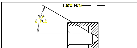
Figure 75 – Slimline device plug connector interface dimensions (section B-B)
