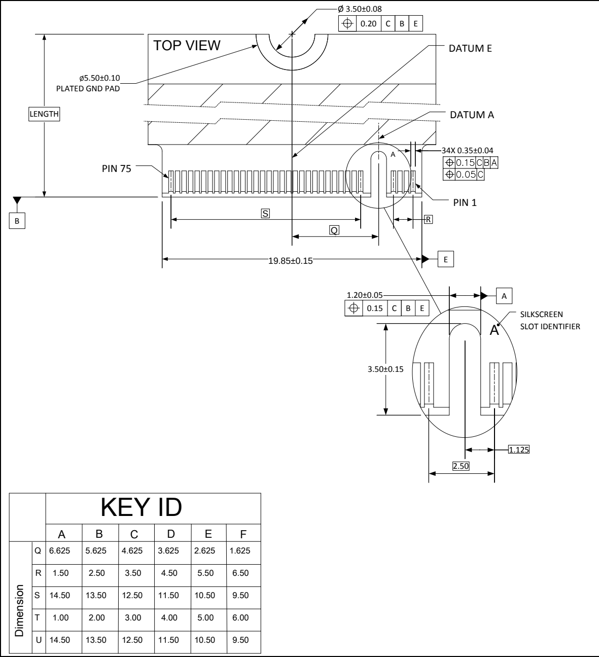
Figure 112 – M.2 board connector top slot details (informative)
