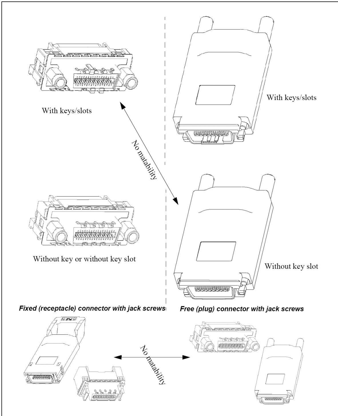
Figure 151 – Plug/receptacle keying
