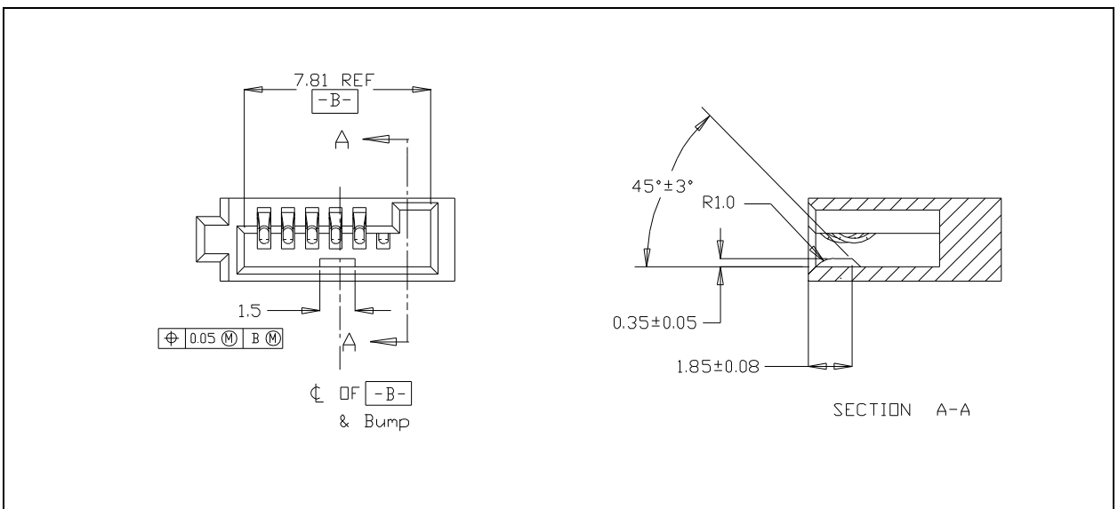
Figure 83 – Slimline power receptacle connector option with bump
