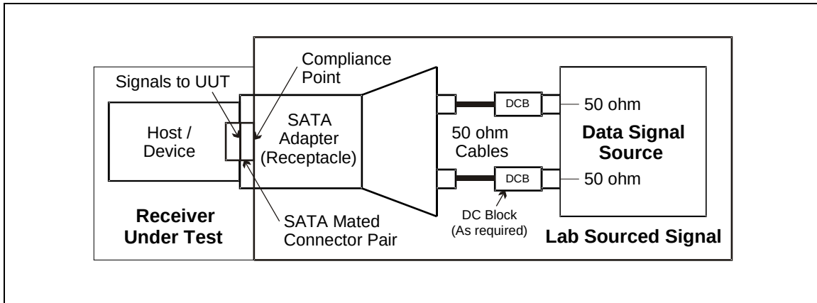
Figure 237 – Receiver intra-pair skew test
