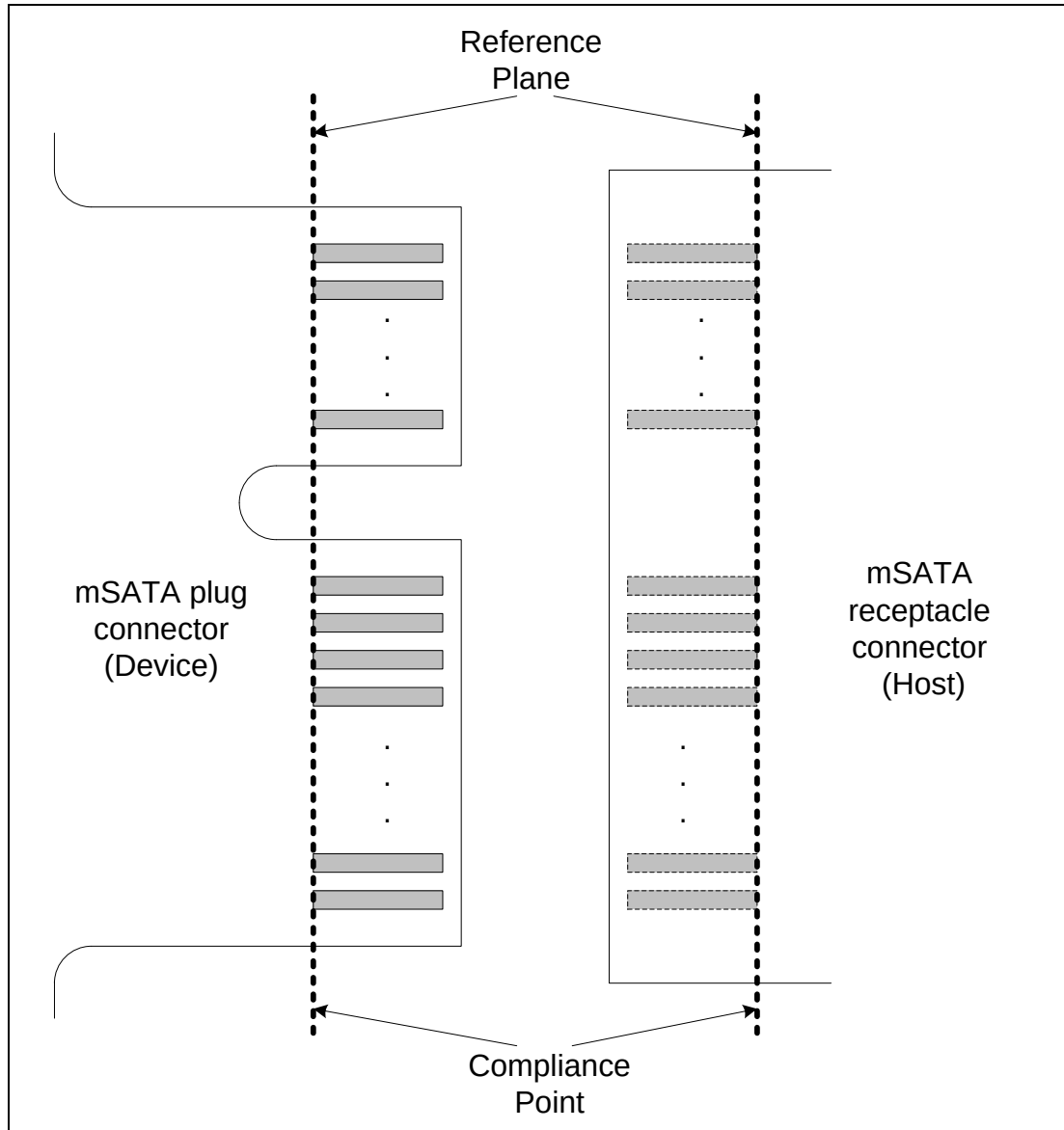
Figure 189 – Mated connector pair for mSATA
